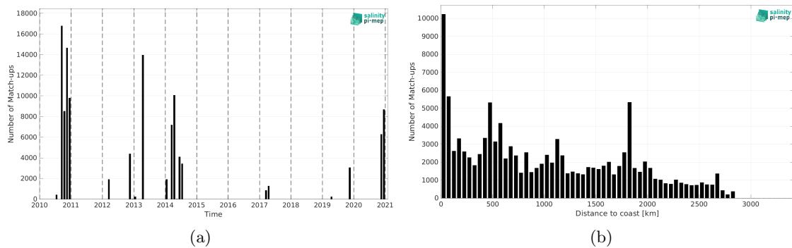
Figure 2: Number of match-ups between TSG (GOSUD-Sailing-ship) and ISAS SSS as a function of time (a) and as function of the distance to coast (b) over the South Atlantic Ocean Pi-MEP region and for the full satellite product period.
