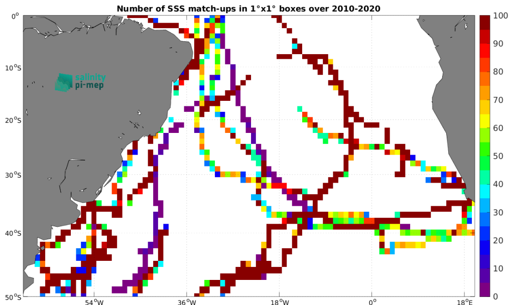
Figure 5: Number of SSS match-ups between TSG (GOSUD-Sailing-ship) SSS and the ISAS SSS product for the South Atlantic Ocean Pi-MEP region over 1^\circ \times 1^\circ boxes and for the full satellite product period.
