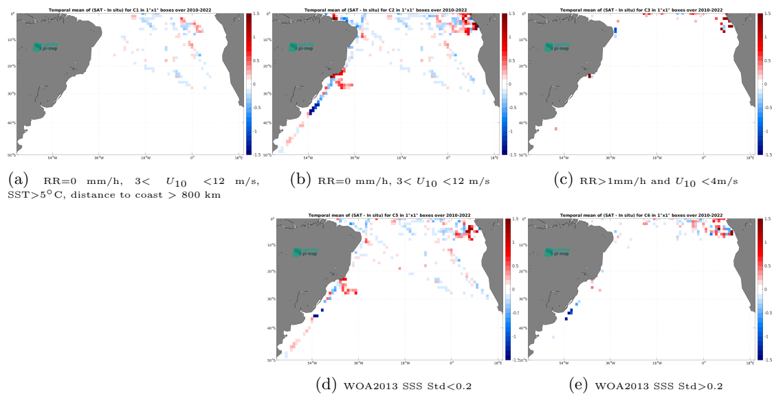
Figure 14: Temporal mean gridded over spatial boxes of size 1^\circ \times 1^\circ of \Delta\text{SSS} (ISAS v7 - Monthly (Ifremer-LOPS-CMEMS) - TSG (GOSUD-Research-vessel)) for 5 different subdatasets corresponding to:RR=0 mm/h, 3 < U_{10} < 12 m/s, SST >5^\circ\text{C} , distance to coast > 800 km (a), RR=0 mm/h, 3 < U_{10} < 12 m/s (b), RR >1 mm/h and U_{10} < 4 m/s (c), WOA2013 SSS Std <0.2 (d), WOA2013 SSS Std >0.2 (e).
