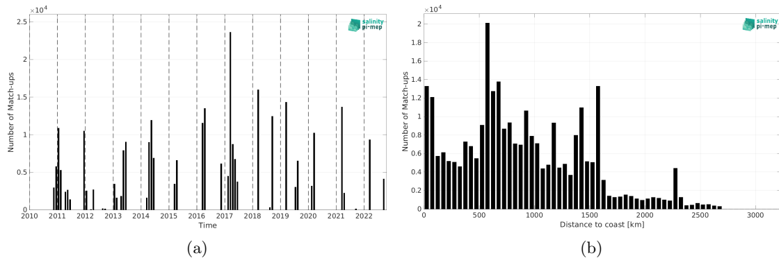
Figure 2: Number of match-ups between TSG (GOSUD-Research-vessel) and ISAS v7 - Monthly (Ifremer-LOPS-CMEMS) SSS as a function of time (a) and as function of the distance to coast (b) over the South Atlantic Ocean Pi-MEP region and for the full satellite product period.
