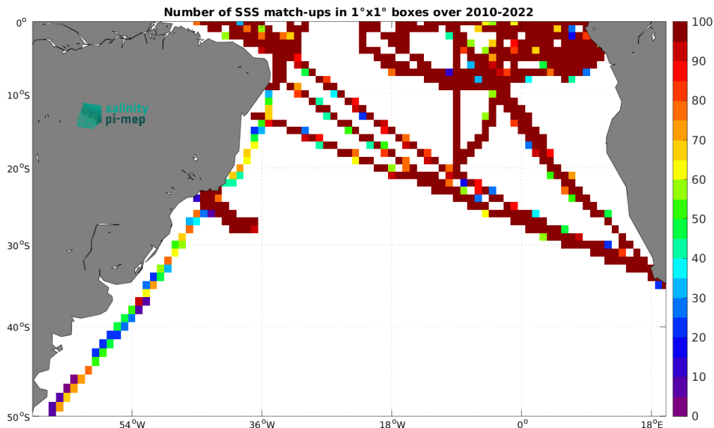
Figure 5: Number of SSS match-ups between TSG (GOSUD-Research-vessel) SSS and the ISAS v7 - Monthly (Ifremer-LOPS-CMEMS) SSS product for the South Atlantic Ocean Pi-MEP region over 1^{\circ} \times 1^{\circ} boxes and for the full satellite product period.
