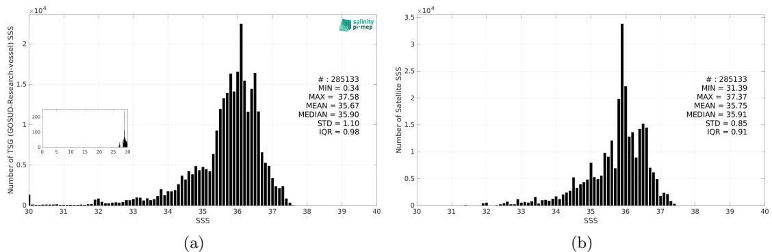
Figure 3: Histograms of SSS from TSG (GOSUD-Research-vessel) (a) and ISAS v7 - Monthly (Ifremer-LOPS-CMEMS) (b) considering all match-up pairs per bins of 0.1 over the South Atlantic Ocean Pi-MEP region and for the full satellite product period.
