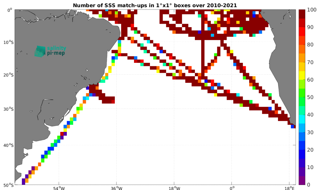
Figure 5: Number of SSS match-ups between TSG (GOSUD-Research-vessel) SSS and the ISAS SSS product for the South Atlantic Ocean Pi-MEP region over 1^{\circ} \times 1^{\circ} boxes and for the full satellite product period.
