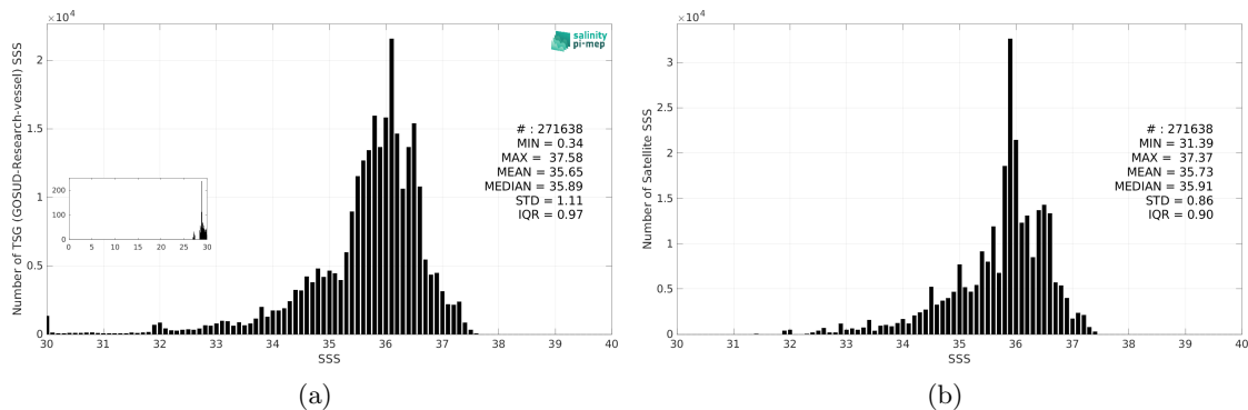
Figure 3: Histograms of SSS from TSG (GOSUD-Research-vessel) (a) and ISAS (b) considering all match-up pairs per bins of 0.1 over the South Atlantic Ocean Pi-MEP region and for the full satellite product period.
