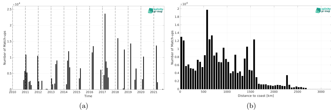
Figure 2: Number of match-ups between TSG (GOSUD-Research-vessel) and ISAS SSS as a function of time (a) and as function of the distance to coast (b) over the South Atlantic Ocean Pi-MEP region and for the full satellite product period.
