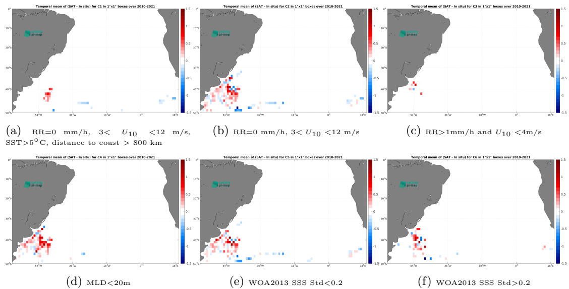
Figure 14: Temporal mean gridded over spatial boxes of size 1^\circ \times 1^\circ of \Delta SSS (ISAS v7 - Monthly (Ifremer-LOPS-CMEMS) - Marine mammals) for 6 different subdatasets corresponding to:RR=0 mm/h, 3 < U_{10} < 12 m/s, SST >5^\circ C, distance to coast > 800 km (a), RR=0 mm/h, 3 < U_{10} < 12 m/s (b), RR >1 mm/h and U_{10} < 4 m/s (c),MLD <20 m (d),WOA2013 SSS Std <0.2 (e),WOA2013 SSS Std >0.2 (f).
