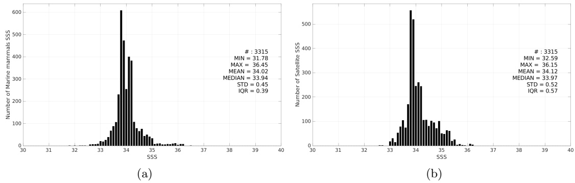
Figure 3: Histograms of SSS from Marine mammals (a) and ISAS v7 - Monthly (Ifremer-LOPS-CMEMS) (b) considering all match-up pairs per bins of 0.1 over the South Atlantic Ocean Pi-MEP region and for the full satellite product period.
