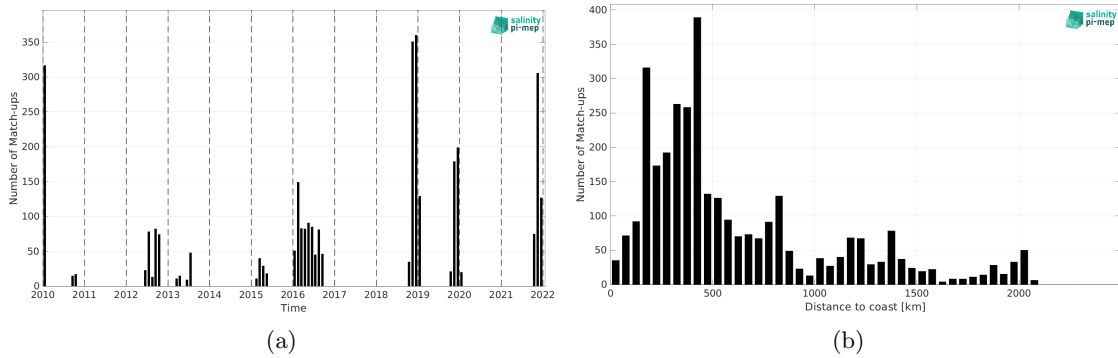
Figure 2: Number of match-ups between Marine mammals and ISAS v7 - Monthly (Ifremer-LOPS-CMEMS) SSS as a function of time (a) and as function of the distance to coast (b) over the South Atlantic Ocean Pi-MEP region and for the full satellite product period.
