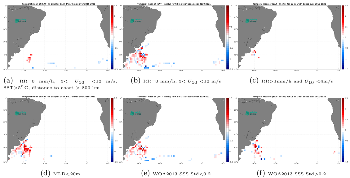
Figure 14: Temporal mean gridded over spatial boxes of size 1^\circ \times 1^\circ of \Delta SSS (ISAS - Marine mammals) for 6 different subdatasets corresponding to:RR=0 mm/h, 3 < U_{10} < 12 m/s, SST > 5^\circ\text{C} , distance to coast > 800 km (a), RR=0 mm/h, 3 < U_{10} < 12 m/s (b), RR > 1 mm/h and U_{10} < 4 m/s (c),MLD < 20 m (d),WOA2013 SSS Std < 0.2 (e),WOA2013 SSS Std > 0.2 (f).
