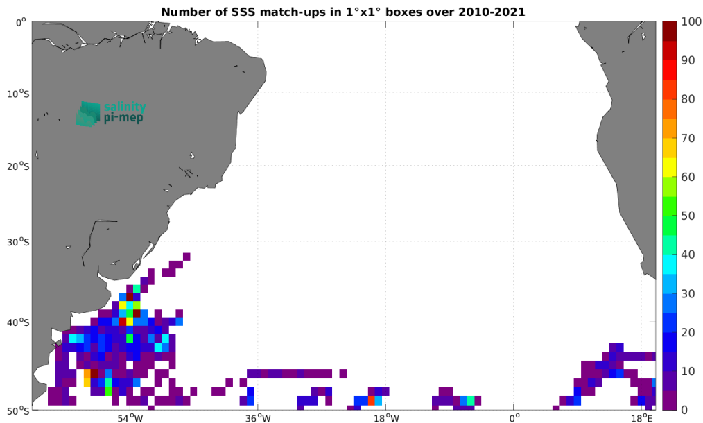
Figure 5: Number of SSS match-ups between Marine mammals SSS and the ISAS SSS product for the South Atlantic Ocean Pi-MEP region over 1^\circ \times 1^\circ boxes and for the full satellite product period.
