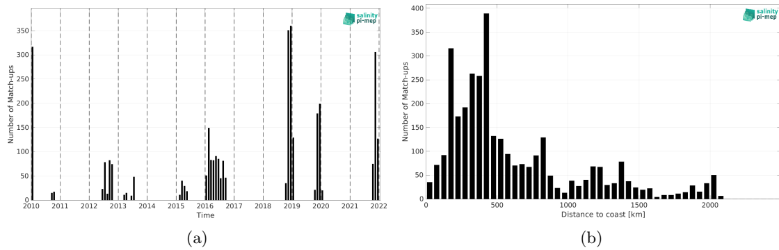
Figure 2: Number of match-ups between Marine mammals and ISAS SSS as a function of time (a) and as function of the distance to coast (b) over the South Atlantic Ocean Pi-MEP region and for the full satellite product period.
