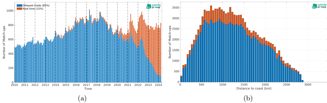
Figure 2: Number of match-ups between Argo and ISAS SSS as a function of time (a) and as function of the distance to coast (b) over the South Atlantic Ocean Pi-MEP region and for the full satellite product period.
