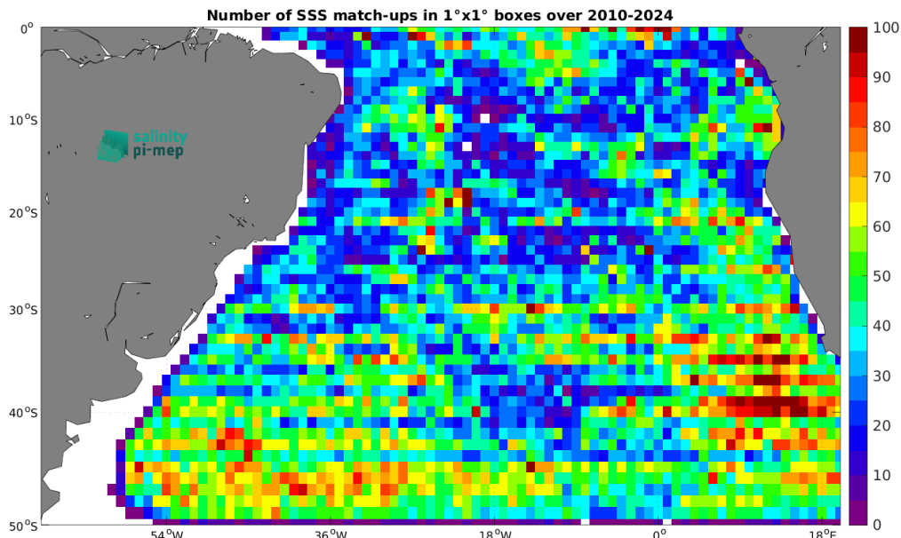
Figure 5: Number of SSS match-ups between Argo SSS and the ISAS SSS product for the South Atlantic Ocean Pi-MEP region over 1^{\circ} \times 1^{\circ} boxes and for the full satellite product period.
