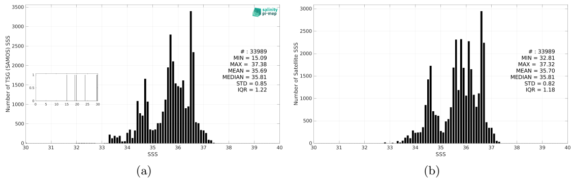
Figure 3: Histograms of SSS from TSG (SAMOS) (a) and CCI SSS L4 Merged-OI v5.5 - 7-day running (ESA) (b) considering all match-up pairs per bins of 0.1 over the South Atlantic Ocean Pi-MEP region and for the full satellite product period.
