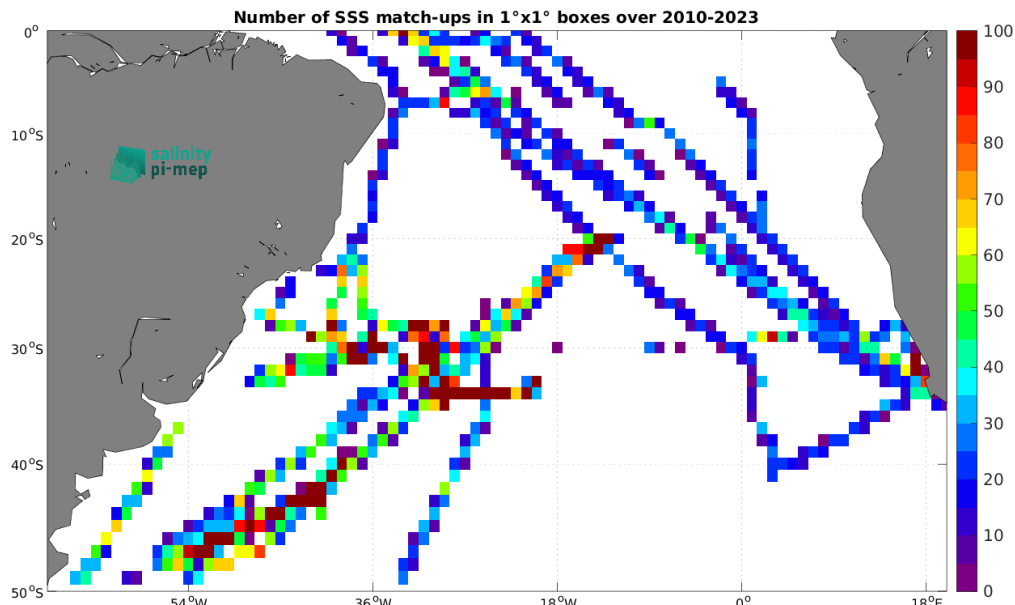
Figure 5: Number of SSS match-ups between TSG (SAMOS) SSS and the CCI SSS L4 Merged-OI v5.5 - 7-day running (ESA) SSS product for the South Atlantic Ocean Pi-MEP region over 1^\circ \times 1^\circ boxes and for the full satellite product period.
