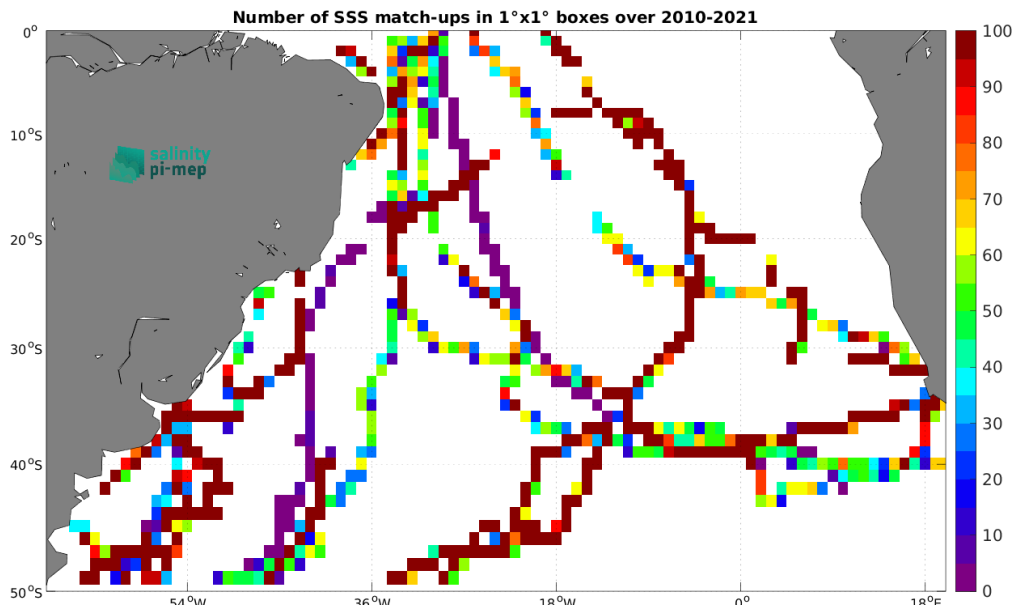
Figure 5: Number of SSS match-ups between TSG (GOSUD-Sailing-ship) SSS and the CCI SSS L4 Merged-OI v5.5 - 7-day running (ESA) SSS product for the South Atlantic Ocean Pi-MEP region over 1^\circ \times 1^\circ boxes and for the full satellite product period.
