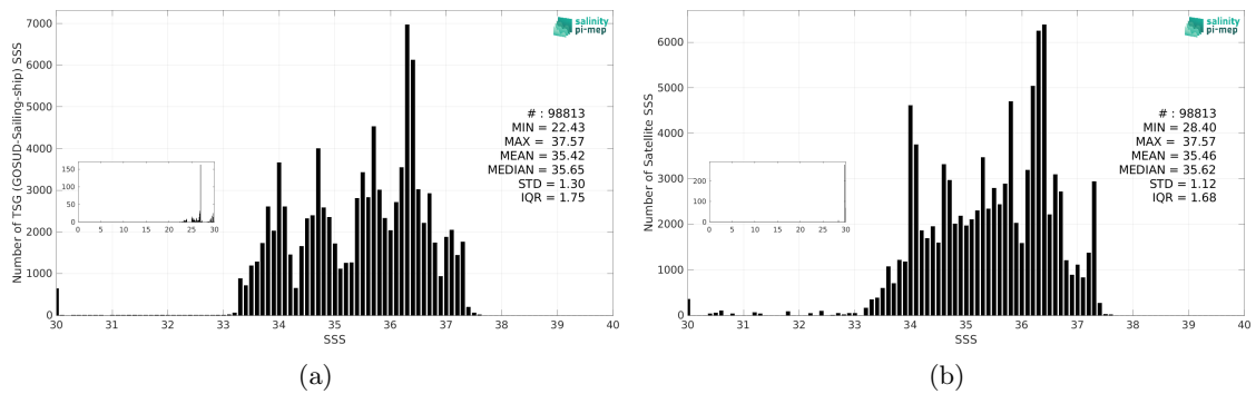
Figure 3: Histograms of SSS from TSG (GOSUD-Sailing-ship) (a) and CCI SSS L4 Merged-OI v5.5 - 7-day running (ESA) (b) considering all match-up pairs per bins of 0.1 over the South Atlantic Ocean Pi-MEP region and for the full satellite product period.
