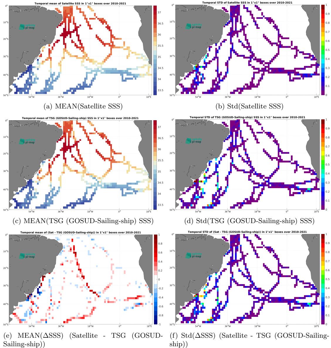
Figure 7: Temporal mean (left) and Std (right) of SSS from CCI SSS L4 Merged-OI v5.5 - 7-day running (ESA) (top), TSG (GOSUD-Sailing-ship) (middle), and of \Delta SSS (Satellite - TSG (GOSUD-Sailing-ship)). Only match-up pairs are used to generate these maps.
