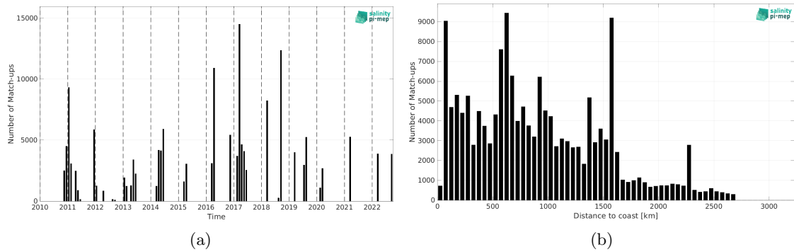
Figure 2: Number of match-ups between TSG (GOSUD-Research-vessel) and CCI SSS L4 Merged-OI v5.5 - 7-day running (ESA) SSS as a function of time (a) and as function of the distance to coast (b) over the South Atlantic Ocean Pi-MEP region and for the full satellite product period.
