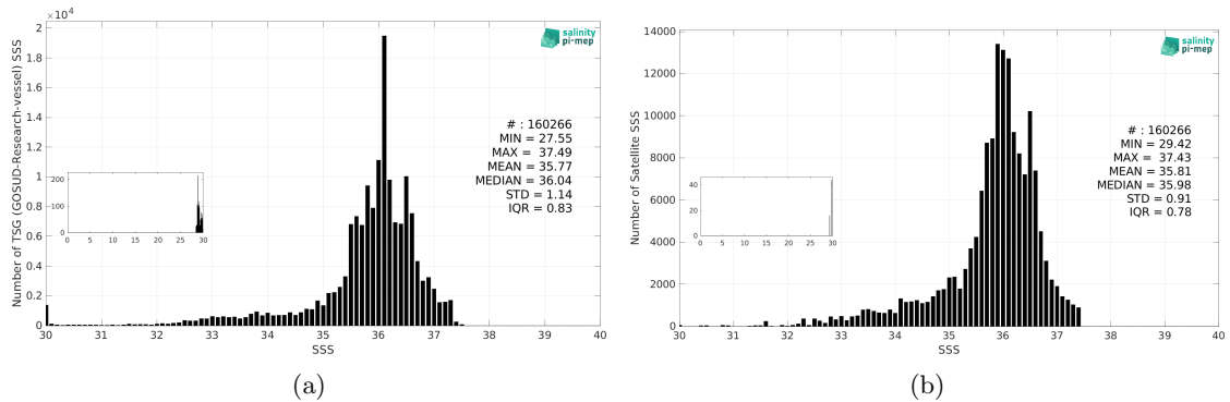
Figure 3: Histograms of SSS from TSG (GOSUD-Research-vessel) (a) and CCI SSS L4 Merged-OI v5.5 - 7-day running (ESA) (b) considering all match-up pairs per bins of 0.1 over the South Atlantic Ocean Pi-MEP region and for the full satellite product period.
