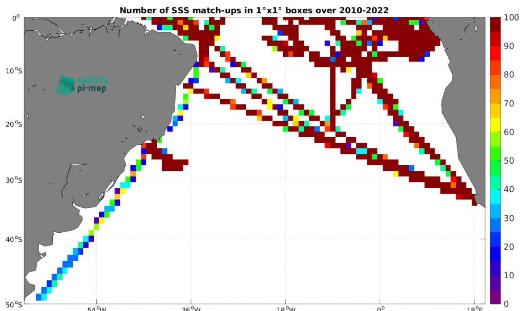
Figure 5: Number of SSS match-ups between TSG (GOSUD-Research-vessel) SSS and the CCI SSS L4 Merged-OI v5.5 - 7-day running (ESA) SSS product for the South Atlantic Ocean Pi-MEP region over 1^\circ \times 1^\circ boxes and for the full satellite product period.
