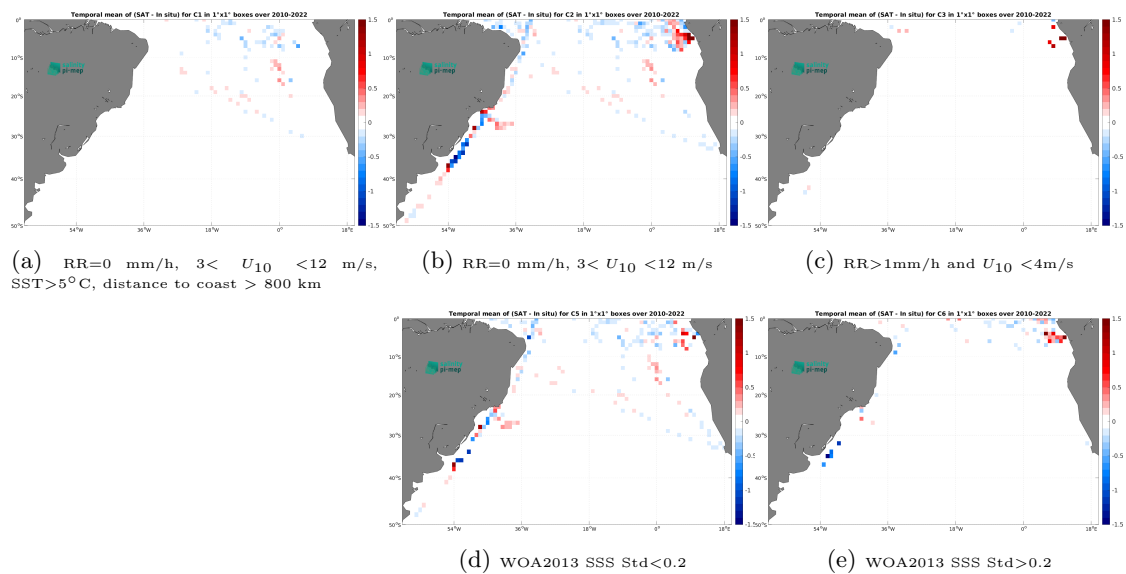
Figure 14: Temporal mean gridded over spatial boxes of size 1^\circ \times 1^\circ of \Delta\text{SSS} (CCI SSS L4 Merged-OI v5.5 - 7-day running (ESA) - TSG (GOSUD-Research-vessel)) for 5 different subdatasets corresponding to:RR=0 mm/h, 3 < U_{10} < 12 m/s, SST >5^\circ\text{C} , distance to coast > 800 km (a), RR=0 mm/h, 3 < U_{10} < 12 m/s (b), RR >1 mm/h and U_{10} < 4 m/s (c), WOA2013 SSS Std <0.2 (d), WOA2013 SSS Std >0.2 (e).
