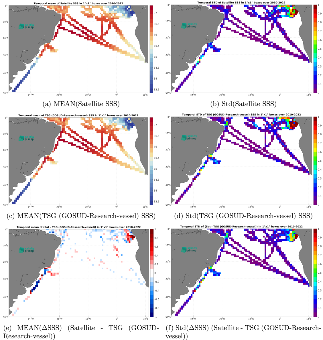
Figure 7: Temporal mean (left) and Std (right) of SSS from CCI SSS L4 Merged-OI v5.5 - 7-day running (ESA) (top), TSG (GOSUD-Research-vessel) (middle), and of \Delta SSS (Satellite - TSG (GOSUD-Research-vessel)). Only match-up pairs are used to generate these maps.
