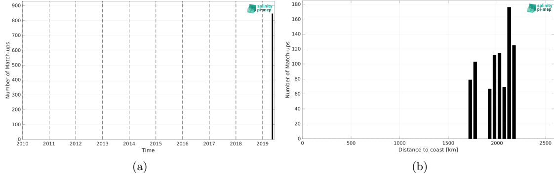
Figure 2: Number of match-ups between Saildrone and CCI SSS L4 Merged-OI v5.5 - 7-day running (ESA) SSS as a function of time (a) and as function of the distance to coast (b) over the South Atlantic Ocean Pi-MEP region and for the full satellite product period.
