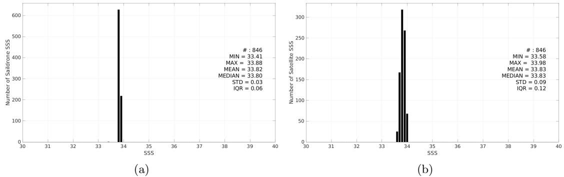
Figure 3: Histograms of SSS from Saildrone (a) and CCI SSS L4 Merged-OI v5.5 - 7-day running (ESA) (b) considering all match-up pairs per bins of 0.1 over the South Atlantic Ocean Pi-MEP region and for the full satellite product period.
