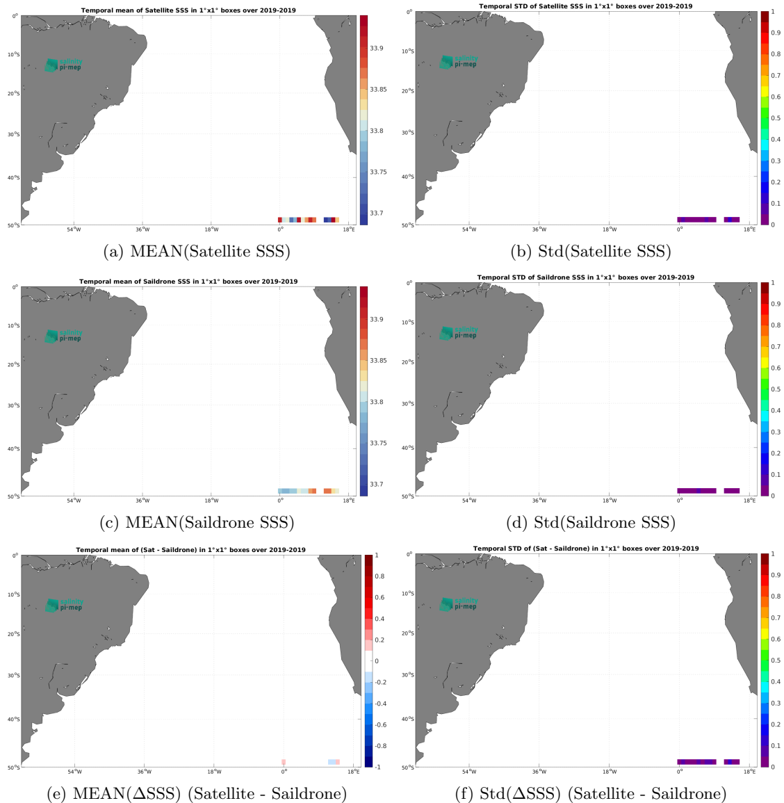
Figure 7: Temporal mean (left) and Std (right) of SSS from CCI SSS L4 Merged-OI v5.5 - 7-day running (ESA) (top), Saildrone (middle), and of \Delta SSS (Satellite - Saildrone). Only match-up pairs are used to generate these maps.
