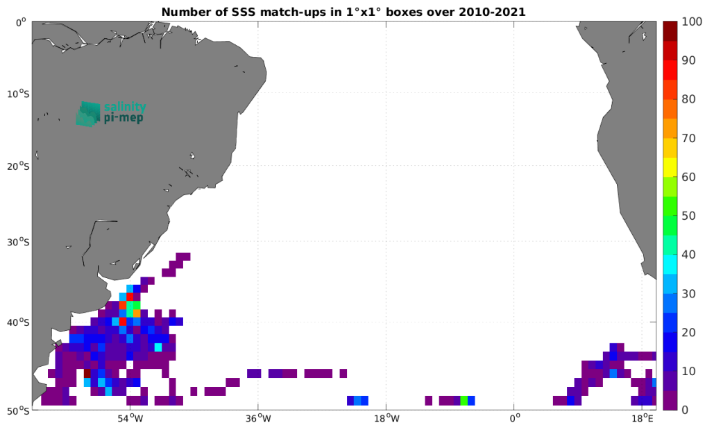
Figure 5: Number of SSS match-ups between Marine mammals SSS and the CCI SSS L4 Merged-OI v5.5 - 7-day running (ESA) SSS product for the South Atlantic Ocean Pi-MEP region over 1^\circ \times 1^\circ boxes and for the full satellite product period.
