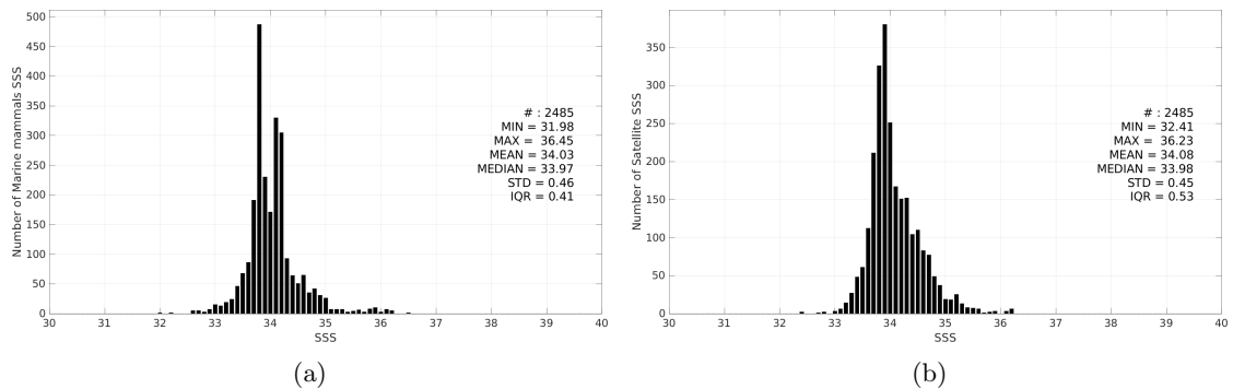
Figure 3: Histograms of SSS from Marine mammals (a) and CCI SSS L4 Merged-OI v5.5 - 7-day running (ESA) (b) considering all match-up pairs per bins of 0.1 over the South Atlantic Ocean Pi-MEP region and for the full satellite product period.
