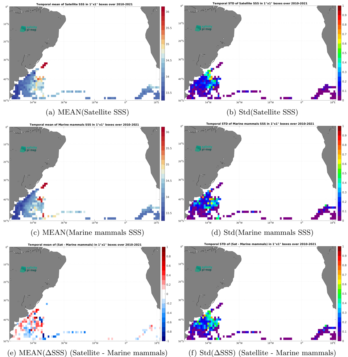
Figure 7: Temporal mean (left) and Std (right) of SSS from CCI SSS L4 Merged-OI v5.5 - 7-day running (ESA) (top), Marine mammals (middle), and of \Delta SSS (Satellite - Marine mammals). Only match-up pairs are used to generate these maps.
