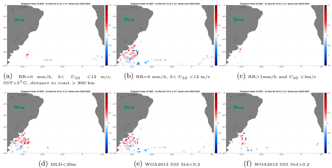
Figure 14: Temporal mean gridded over spatial boxes of size 1^\circ \times 1^\circ of \Delta SSS (CCI SSS L4 Merged-OI v5.5 - 7-day running (ESA) - Marine mammals) for 6 different subdatasets corresponding to:RR=0 mm/h, 3 < U_{10} < 12 m/s, SST >5^\circ C, distance to coast > 800 km (a), RR=0 mm/h, 3 < U_{10} < 12 m/s (b), RR >1 mm/h and U_{10} < 4 m/s (c),MLD <20 m (d),WOA2013 SSS Std <0.2 (e),WOA2013 SSS Std >0.2 (f).
