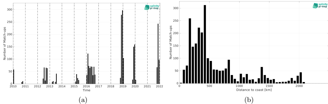
Figure 2: Number of match-ups between Marine mammals and CCI SSS L4 Merged-OI v5.5 - 7-day running (ESA) SSS as a function of time (a) and as function of the distance to coast (b) over the South Atlantic Ocean Pi-MEP region and for the full satellite product period.
