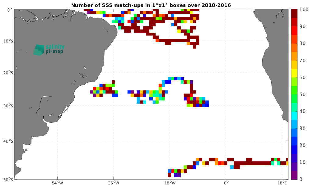
Figure 4: Number of SSS match-ups between Surface drifters SSS and the CCI SSS L4 Merged-OI v5.5 - 7-day running (ESA) SSS product for the South Atlantic Ocean Pi-MEP region over 1^\circ \times 1^\circ boxes and for the full satellite product period.
