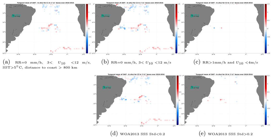
Figure 13: Temporal mean gridded over spatial boxes of size 1^\circ \times 1^\circ of \Delta\text{SSS} (CCI SSS L4 Merged-OI v5.5 - 7-day running (ESA) - Surface drifters) for 5 different subdatasets corresponding to:RR=0 mm/h, 3 < U_{10} < 12 m/s, SST >5^\circ\text{C} , distance to coast > 800 km (a), RR=0 mm/h, 3 < U_{10} < 12 m/s (b), RR >1 mm/h and U_{10} < 4 m/s (c), WOA2013 SSS Std <0.2 (d), WOA2013 SSS Std >0.2 (e).
