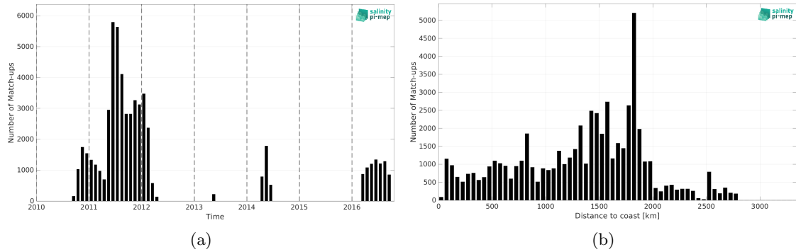
Figure 2: Number of match-ups between Surface drifters and CCI SSS L4 Merged-OI v5.5 - 7-day running (ESA) SSS as a function of time (a) and as function of the distance to coast (b) over the South Atlantic Ocean Pi-MEP region and for the full satellite product period.
