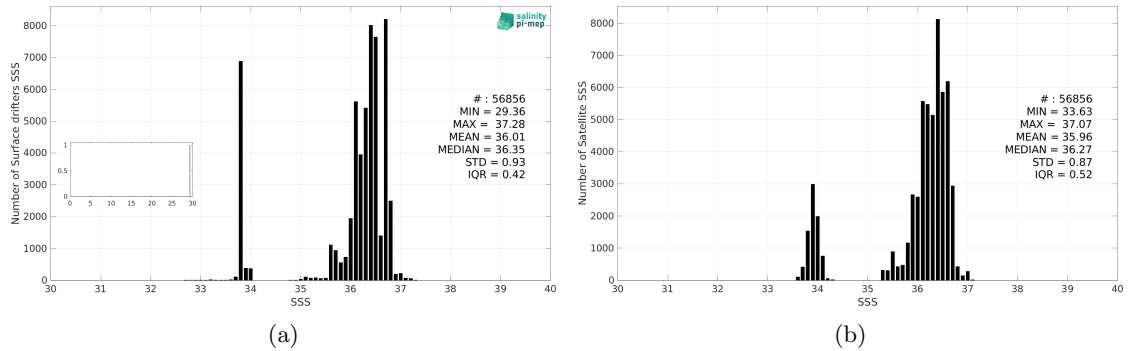
Figure 3: Histograms of SSS from Surface drifters (a) and CCI SSS L4 Merged-OI v5.5 - 7-day running (ESA) (b) considering all match-up pairs per bins of 0.1 over the South Atlantic Ocean Pi-MEP region and for the full satellite product period.
