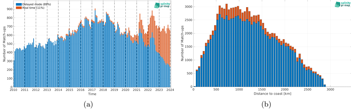
Figure 2: Number of match-ups between Argo and CCI SSS L4 Merged-OI v5.5 - 7-day running (ESA) SSS as a function of time (a) and as function of the distance to coast (b) over the South Atlantic Ocean Pi-MEP region and for the full satellite product period.
