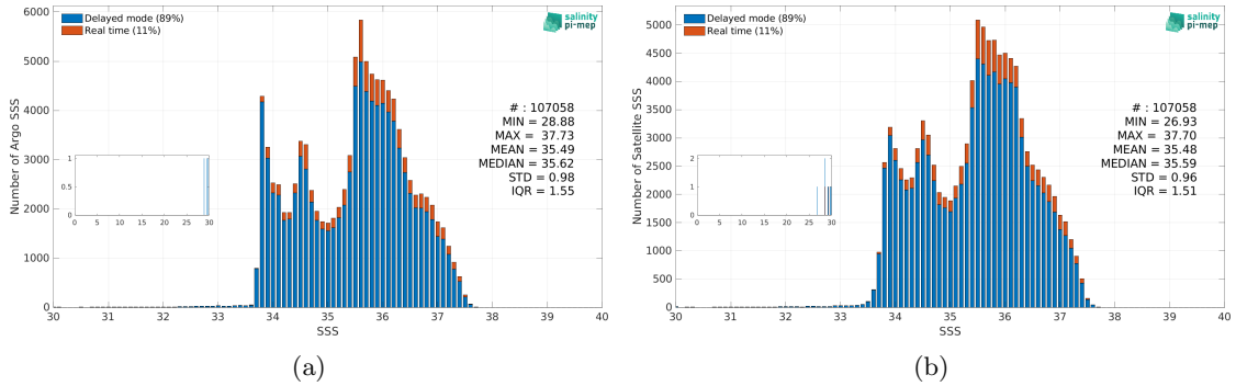
Figure 3: Histograms of SSS from Argo (a) and CCI SSS L4 Merged-OI v5.5 - 7-day running (ESA) (b) considering all match-up pairs per bins of 0.1 over the South Atlantic Ocean Pi-MEP region and for the full satellite product period.
