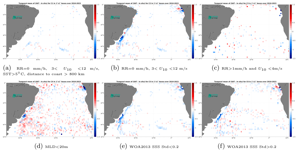
Figure 14: Temporal mean gridded over spatial boxes of size 1^\circ \times 1^\circ of \Delta SSS (CCI SSS L4 Merged-OI v5.5 - 7-day running (ESA) - Argo) for 6 different subdatasets corresponding to:RR=0 mm/h, 3 < U_{10} < 12 m/s, SST > 5^\circ\text{C} , distance to coast > 800 km (a), RR=0 mm/h, 3 < U_{10} < 12 m/s (b), RR > 1 mm/h and U_{10} < 4 m/s (c),MLD < 20 m (d),WOA2013 SSS Std < 0.2 (e),WOA2013 SSS Std > 0.2 (f).
