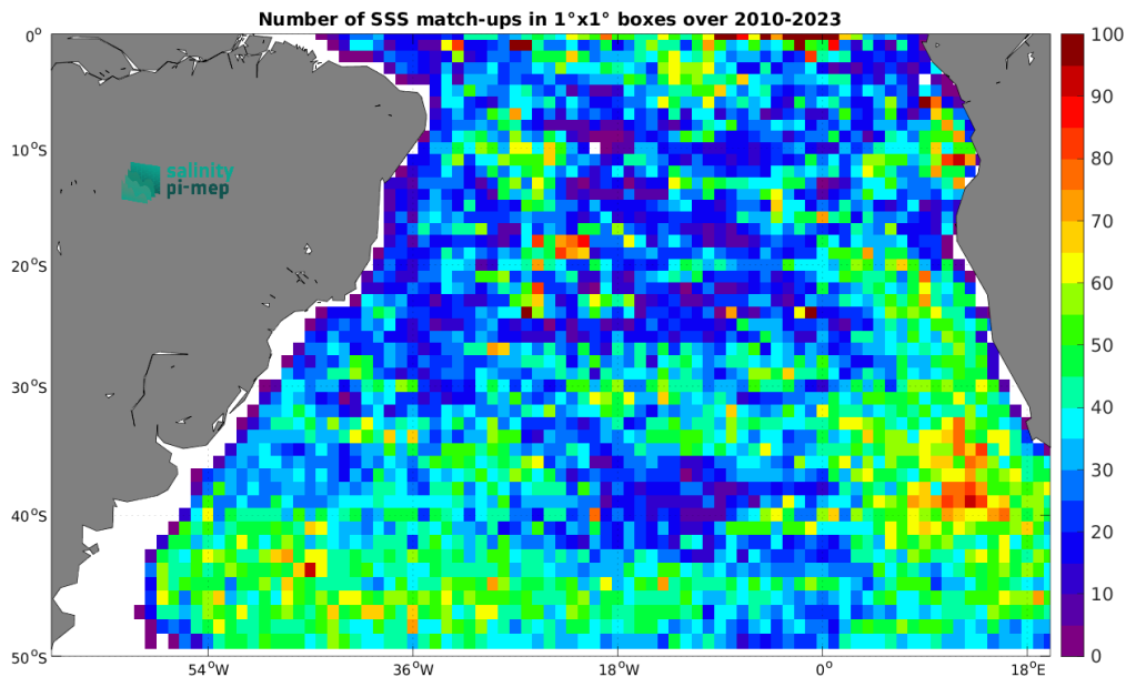
Figure 5: Number of SSS match-ups between Argo SSS and the CCI SSS L4 Merged-OI v5.5 - 7-day running (ESA) SSS product for the South Atlantic Ocean Pi-MEP region over 1^\circ \times 1^\circ boxes and for the full satellite product period.
