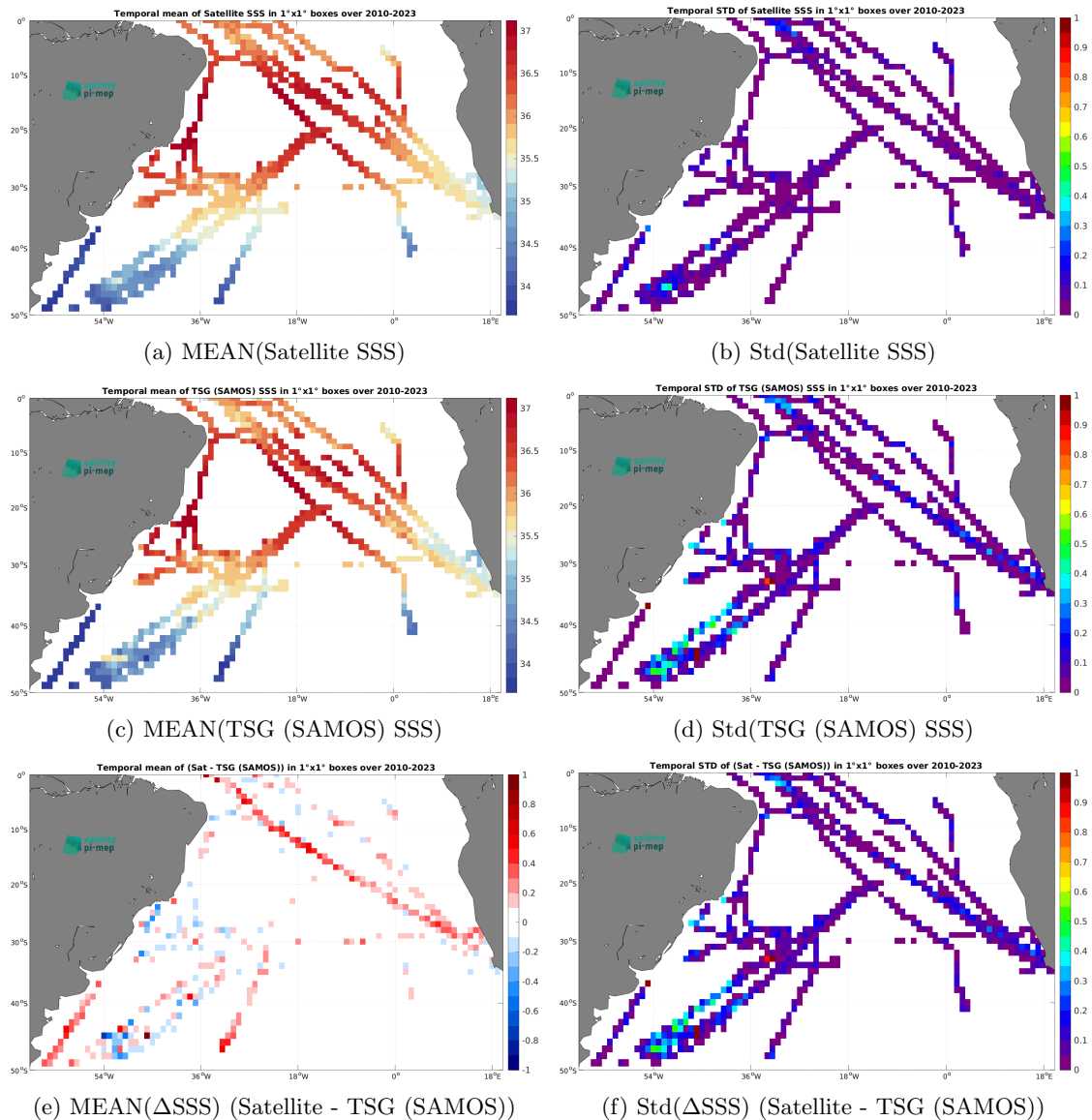
Figure 7: Temporal mean (left) and Std (right) of SSS from CCI SSS L4 Merged-OI v5.5 - 30-day running (ESA) (top), TSG (SAMOS) (middle), and of \Delta SSS (Satellite - TSG (SAMOS)). Only match-up pairs are used to generate these maps.
