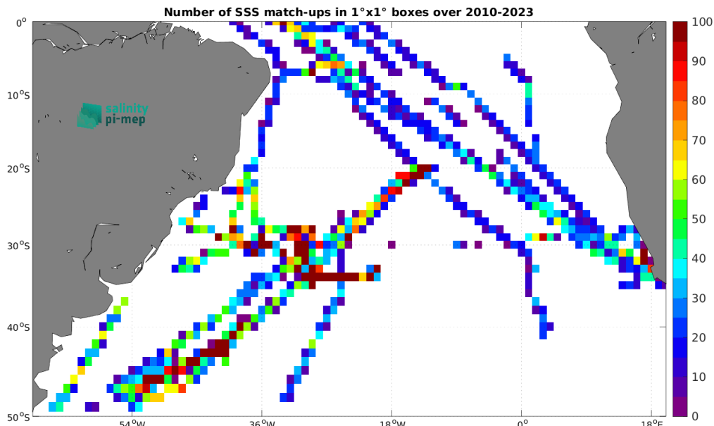
Figure 5: Number of SSS match-ups between TSG (SAMOS) SSS and the CCI SSS L4 Merged-OI v5.5 - 30-day running (ESA) SSS product for the South Atlantic Ocean Pi-MEP region over 1^\circ \times 1^\circ boxes and for the full satellite product period.
