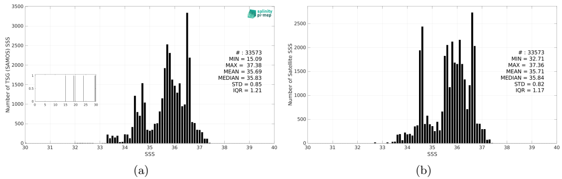
Figure 3: Histograms of SSS from TSG (SAMOS) (a) and CCI SSS L4 Merged-OI v5.5 - 30-day running (ESA) (b) considering all match-up pairs per bins of 0.1 over the South Atlantic Ocean Pi-MEP region and for the full satellite product period.
