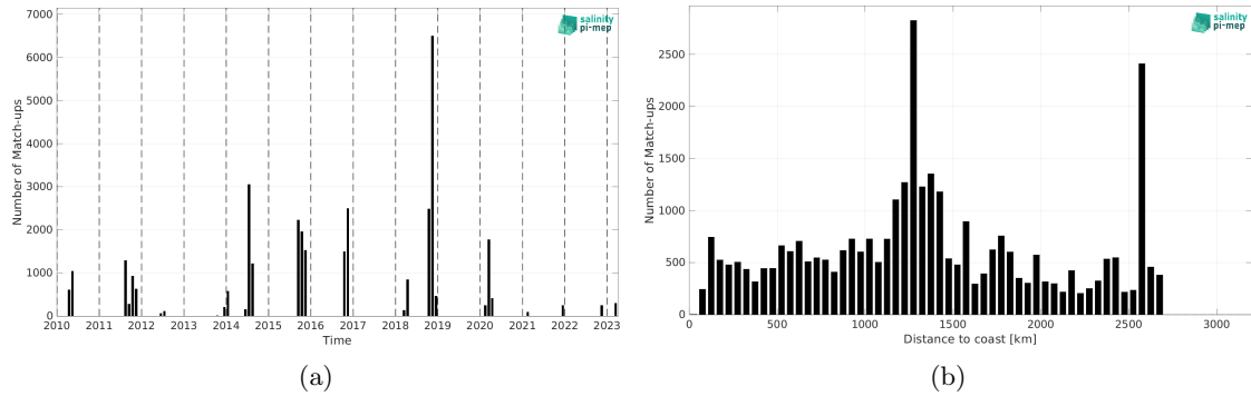
Figure 2: Number of match-ups between TSG (SAMOS) and CCI SSS L4 Merged-OI v5.5 - 30-day running (ESA) SSS as a function of time (a) and as function of the distance to coast (b) over the South Atlantic Ocean Pi-MEP region and for the full satellite product period.
