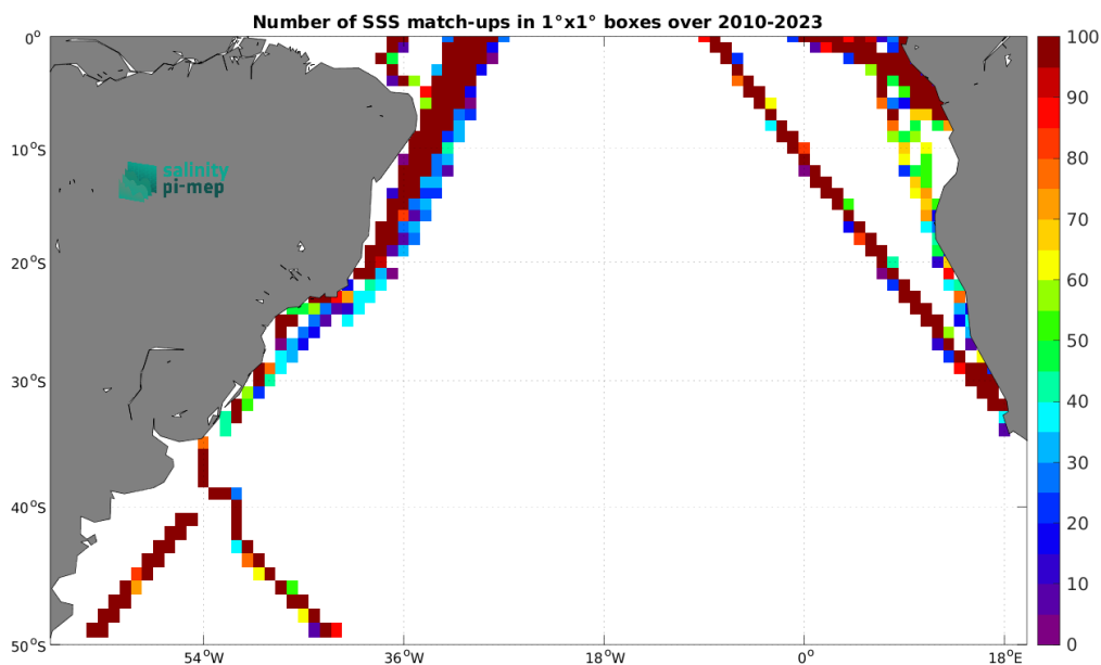
Figure 5: Number of SSS match-ups between TSG (LEGOS-DM) SSS and the CCI SSS L4 Merged-OI v5.5 - 30-day running (ESA) SSS product for the South Atlantic Ocean Pi-MEP region over 1^\circ \times 1^\circ boxes and for the full satellite product period.
