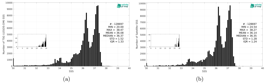
Figure 3: Histograms of SSS from TSG (LEGOS-DM) (a) and CCI SSS L4 Merged-OI v5.5 - 30-day running (ESA) (b) considering all match-up pairs per bins of 0.1 over the South Atlantic Ocean Pi-MEP region and for the full satellite product period.
