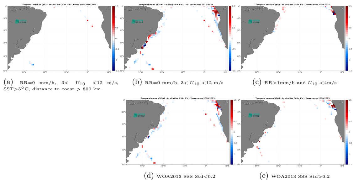
Figure 14: Temporal mean gridded over spatial boxes of size 1^\circ \times 1^\circ of \Delta\text{SSS} (CCI SSS L4 Merged-OI v5.5 - 30-day running (ESA) - TSG (LEGOS-DM)) for 5 different subdatasets corresponding to:RR=0 mm/h, 3 < U_{10} < 12 m/s, SST >5^\circ\text{C} , distance to coast > 800 km (a), RR=0 mm/h, 3 < U_{10} < 12 m/s (b), RR >1 mm/h and U_{10} < 4 m/s (c), WOA2013 SSS Std <0.2 (d), WOA2013 SSS Std >0.2 (e).
