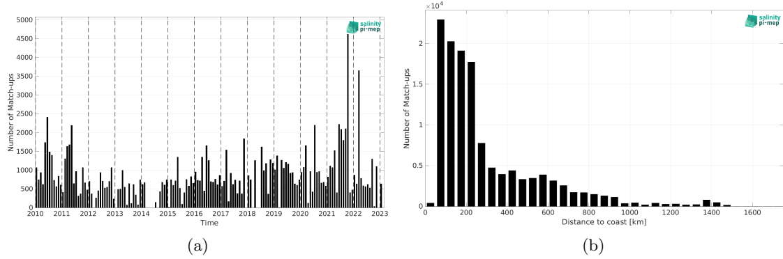
Figure 2: Number of match-ups between TSG (LEGOS-DM) and CCI SSS L4 Merged-OI v5.5 - 30-day running (ESA) SSS as a function of time (a) and as function of the distance to coast (b) over the South Atlantic Ocean Pi-MEP region and for the full satellite product period.
