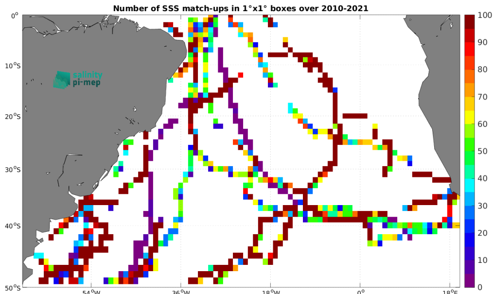
Figure 5: Number of SSS match-ups between TSG (GOSUD-Sailing-ship) SSS and the CCI SSS L4 Merged-OI v5.5 - 30-day running (ESA) SSS product for the South Atlantic Ocean Pi-MEP region over 1^\circ \times 1^\circ boxes and for the full satellite product period.
