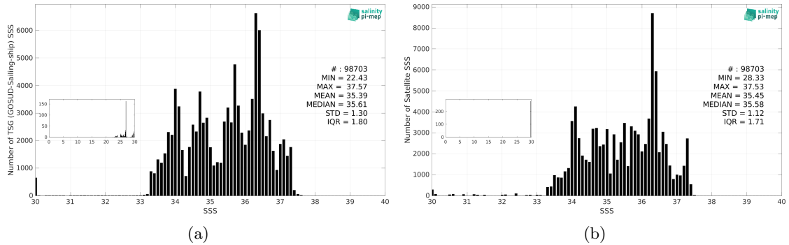
Figure 3: Histograms of SSS from TSG (GOSUD-Sailing-ship) (a) and CCI SSS L4 Merged-OI v5.5 - 30-day running (ESA) (b) considering all match-up pairs per bins of 0.1 over the South Atlantic Ocean Pi-MEP region and for the full satellite product period.
