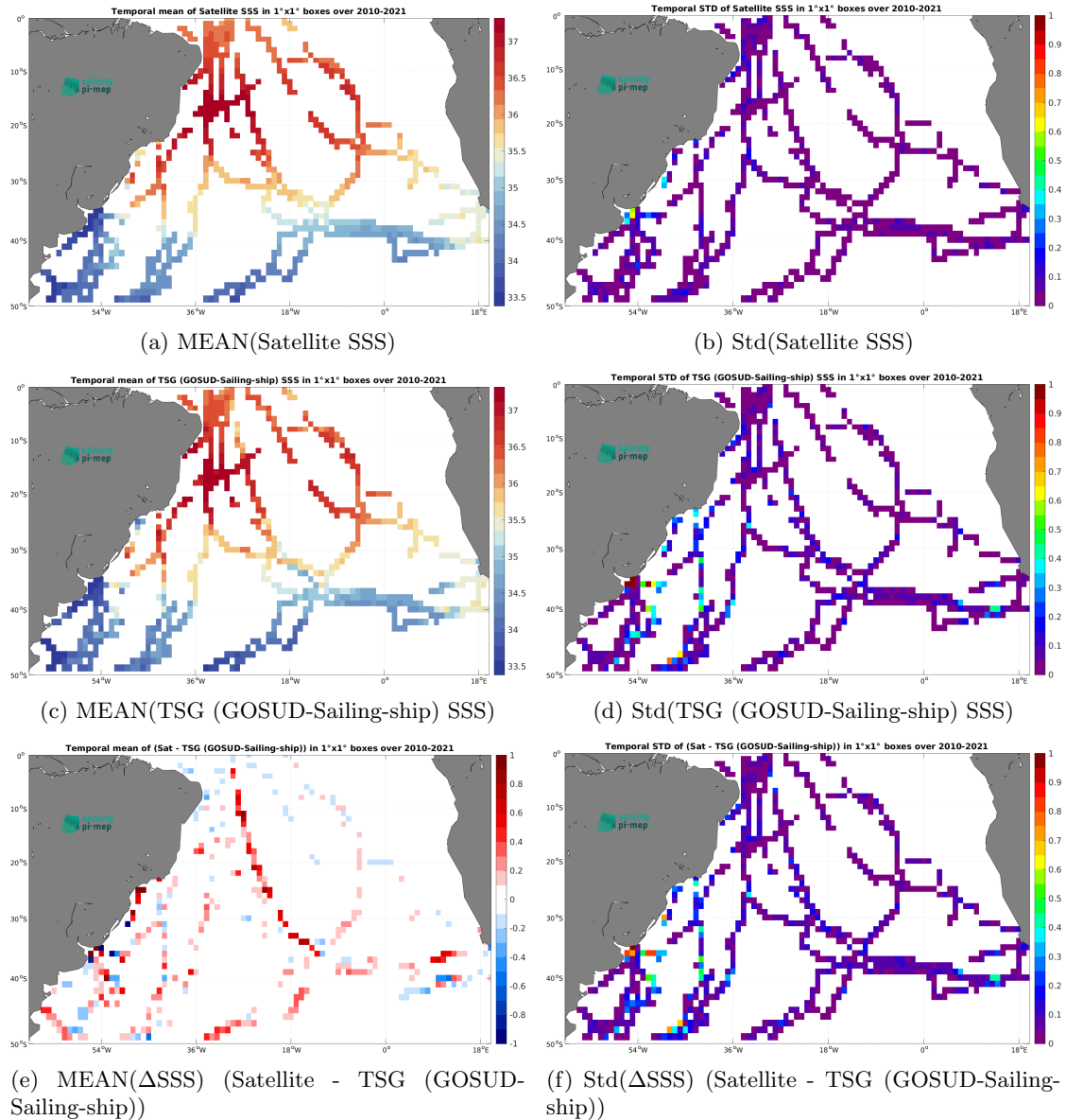
Figure 7: Temporal mean (left) and Std (right) of SSS from CCI SSS L4 Merged-OI v5.5 - 30-day running (ESA) (top), TSG (GOSUD-Sailing-ship) (middle), and of \Delta SSS (Satellite - TSG (GOSUD-Sailing-ship)). Only match-up pairs are used to generate these maps.
