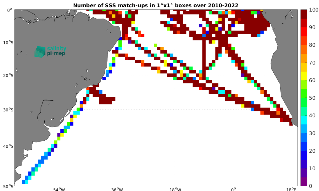
Figure 5: Number of SSS match-ups between TSG (GOSUD-Research-vessel) SSS and the CCI SSS L4 Merged-OI v5.5 - 30-day running (ESA) SSS product for the South Atlantic Ocean Pi-MEP region over 1^\circ \times 1^\circ boxes and for the full satellite product period.
