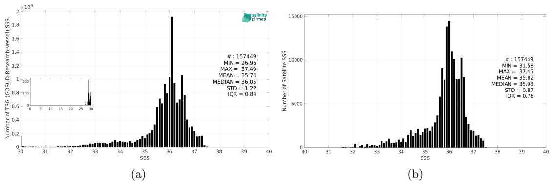
Figure 3: Histograms of SSS from TSG (GOSUD-Research-vessel) (a) and CCI SSS L4 Merged-OI v5.5 - 30-day running (ESA) (b) considering all match-up pairs per bins of 0.1 over the South Atlantic Ocean Pi-MEP region and for the full satellite product period.
