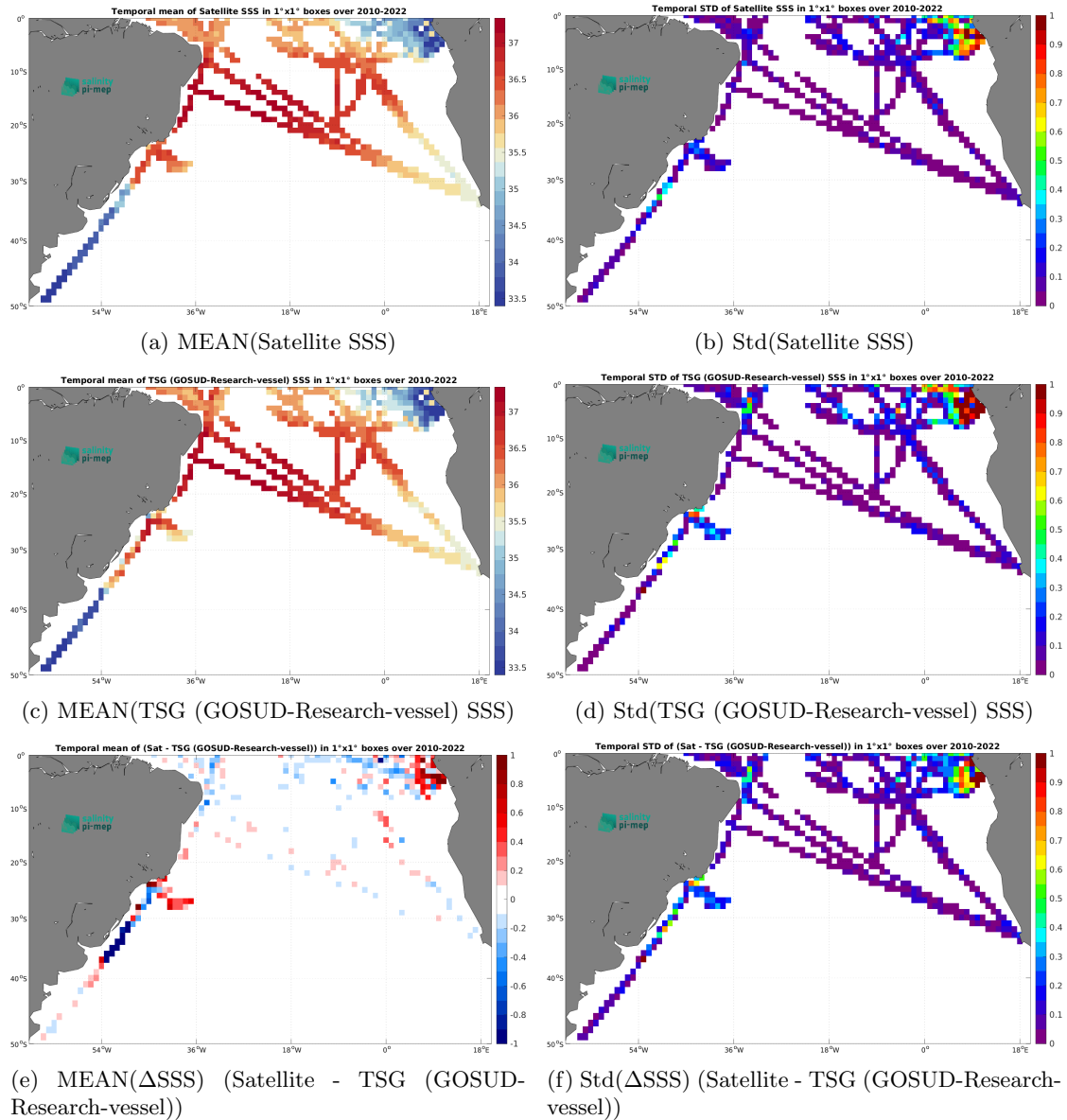
Figure 7: Temporal mean (left) and Std (right) of SSS from CCI SSS L4 Merged-OI v5.5 - 30-day running (ESA) (top), TSG (GOSUD-Research-vessel) (middle), and of \Delta SSS (Satellite - TSG (GOSUD-Research-vessel)). Only match-up pairs are used to generate these maps.
