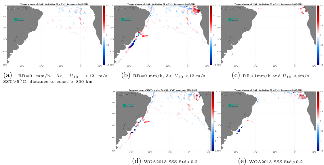
Figure 14: Temporal mean gridded over spatial boxes of size 1^\circ \times 1^\circ of \Delta\text{SSS} (CCI SSS L4 Merged-OI v5.5 - 30-day running (ESA) - TSG (GOSUD-Research-vessel)) for 5 different subdatasets corresponding to:RR=0 mm/h, 3 < U_{10} < 12 m/s, SST >5^\circ\text{C} , distance to coast > 800 km (a), RR=0 mm/h, 3 < U_{10} < 12 m/s (b), RR >1 mm/h and U_{10} < 4 m/s (c), WOA2013 SSS Std <0.2 (d), WOA2013 SSS Std >0.2 (e).
