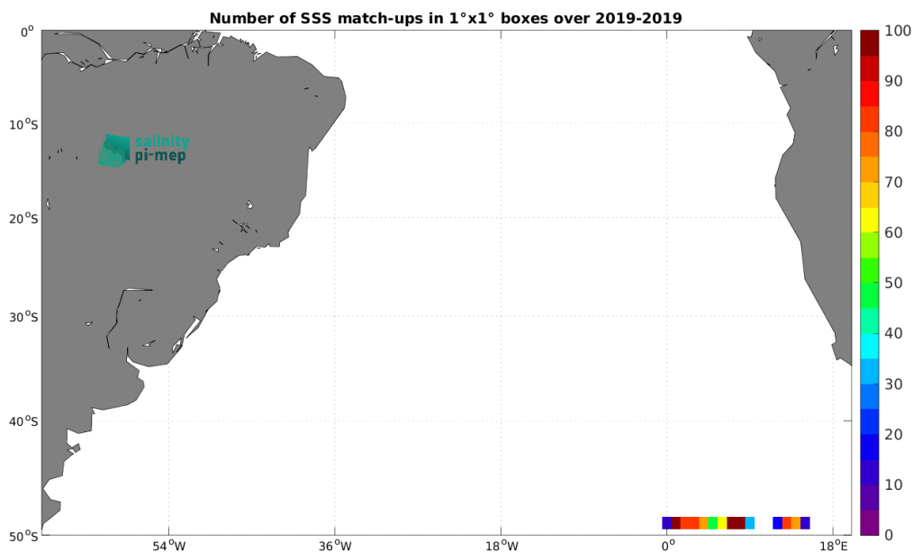
Figure 5: Number of SSS match-ups between Saildrone SSS and the CCI SSS L4 Merged-OI v5.5 - 30-day running (ESA) SSS product for the South Atlantic Ocean Pi-MEP region over 1^\circ \times 1^\circ boxes and for the full satellite product period.
