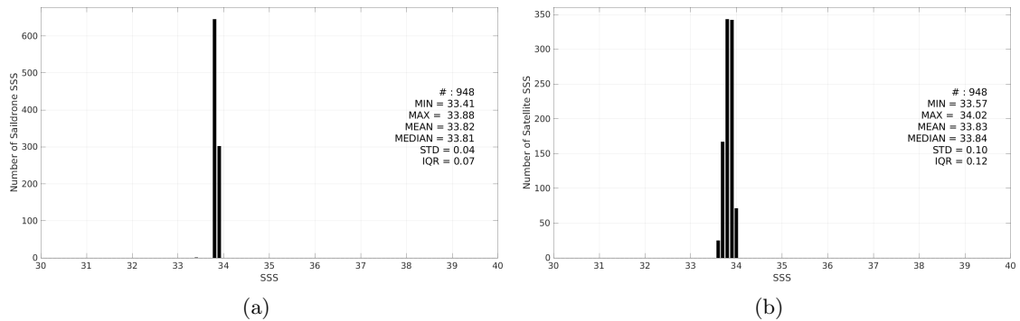
Figure 3: Histograms of SSS from Saildrone (a) and CCI SSS L4 Merged-OI v5.5 - 30-day running (ESA) (b) considering all match-up pairs per bins of 0.1 over the South Atlantic Ocean Pi-MEP region and for the full satellite product period.
