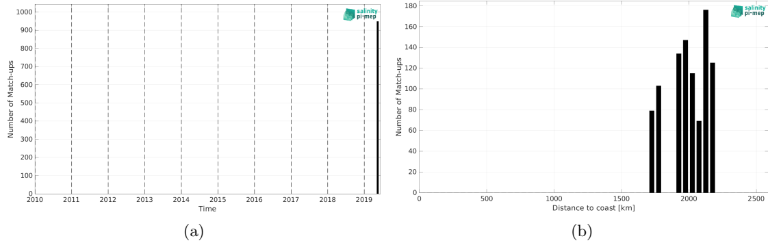
Figure 2: Number of match-ups between Saildrone and CCI SSS L4 Merged-OI v5.5 - 30-day running (ESA) SSS as a function of time (a) and as function of the distance to coast (b) over the South Atlantic Ocean Pi-MEP region and for the full satellite product period.
