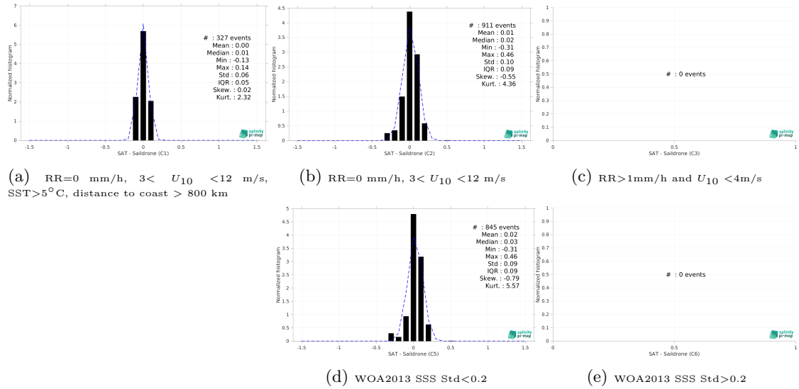
Figure 15: Normalized histogram of \Delta SSS (CCI SSS L4 Merged-OI v5.5 - 30-day running (ESA) - Saldrone) for 5 different subdatasets corresponding to: RR=0 mm/h, 3 < U_{10} < 12 m/s, SST > 5°C, distance to coast > 800 km (a), RR=0 mm/h, 3 < U_{10} < 12 m/s (b), RR > 1mm/h and U_{10} < 4 m/s (c), WOA2013 SSS Std < 0.2 (d), WOA2013 SSS Std > 0.2 (e).
