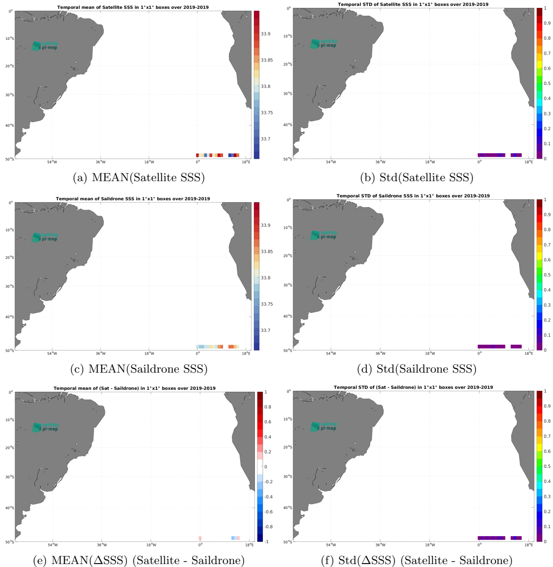
Figure 7: Temporal mean (left) and Std (right) of SSS from CCI SSS L4 Merged-OI v5.5 - 30-day running (ESA) (top), Saildrone (middle), and of \Delta SSS (Satellite - Saildrone). Only match-up pairs are used to generate these maps.
