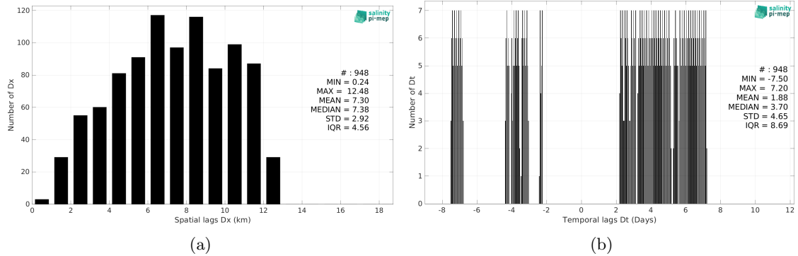
Figure 6: Histograms of the spatial (a) and temporal (b) lags between the location/time of the Sairdrone measurement and the date of the corresponding CCI SSS L4 Merged-OI v5.5 - 30-day running (ESA) SSS pixel.
