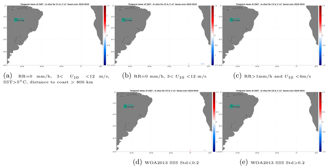
Figure 14: Temporal mean gridded over spatial boxes of size 1^\circ \times 1^\circ of \Delta SSS (CCI SSS L4 Merged-OI v5.5 - 30-day running (ESA) - Saildrone) for 5 different subdatasets corresponding to:RR=0 mm/h, 3 < U_{10} < 12 m/s, SST>5°C, distance to coast > 800 km (a), RR=0 mm/h, 3 < U_{10} < 12 m/s (b), RR>1mm/h and U_{10} < 4 m/s (c), WOA2013 SSS Std<0.2 (d), WOA2013 SSS Std>0.2 (e).
