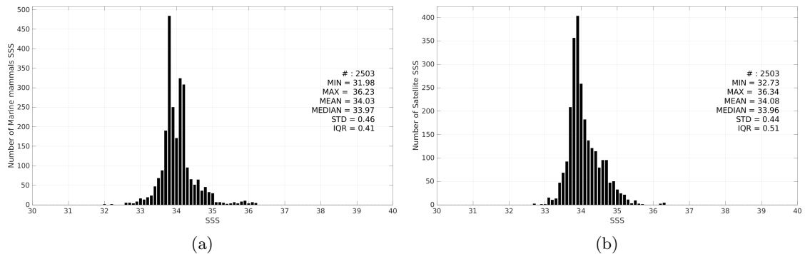
Figure 3: Histograms of SSS from Marine mammals (a) and CCI SSS L4 Merged-OI v5.5 - 30-day running (ESA) (b) considering all match-up pairs per bins of 0.1 over the South Atlantic Ocean Pi-MEP region and for the full satellite product period.
