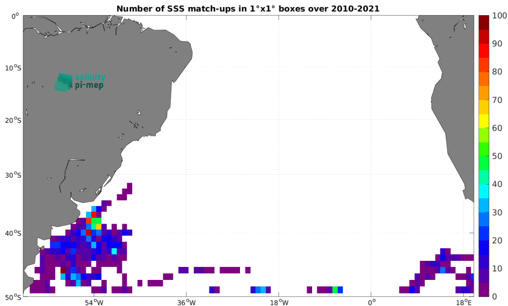
Figure 5: Number of SSS match-ups between Marine mammals SSS and the CCI SSS L4 Merged-OI v5.5 - 30-day running (ESA) SSS product for the South Atlantic Ocean Pi-MEP region over 1^\circ \times 1^\circ boxes and for the full satellite product period.
