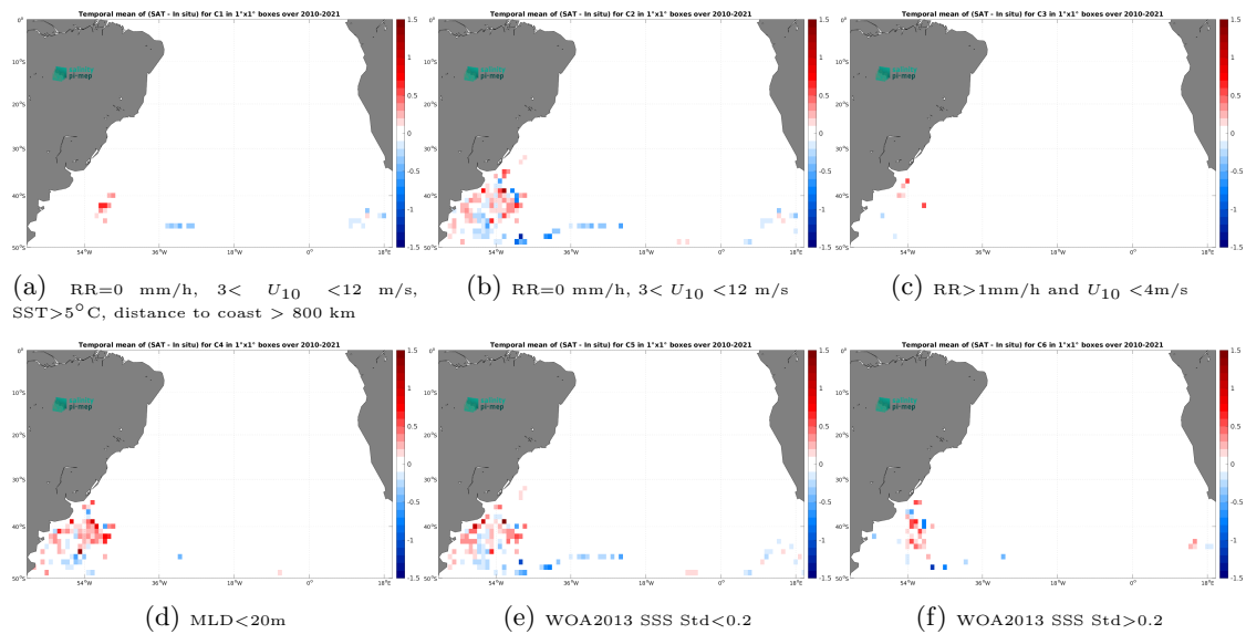
Figure 14: Temporal mean gridded over spatial boxes of size 1^\circ \times 1^\circ of \Delta SSS (CCI SSS L4 Merged-OI v5.5 - 30-day running (ESA) - Marine mammals) for 6 different subdatasets corresponding to:RR=0 mm/h, 3 < U_{10} < 12 m/s, SST >5^\circ C, distance to coast > 800 km (a), RR=0 mm/h, 3 < U_{10} < 12 m/s (b), RR >1 mm/h and U_{10} < 4 m/s (c),MLD <20 m (d),WOA2013 SSS Std <0.2 (e),WOA2013 SSS Std >0.2 (f).
