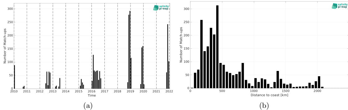
Figure 2: Number of match-ups between Marine mammals and CCI SSS L4 Merged-OI v5.5 - 30-day running (ESA) SSS as a function of time (a) and as function of the distance to coast (b) over the South Atlantic Ocean Pi-MEP region and for the full satellite product period.
