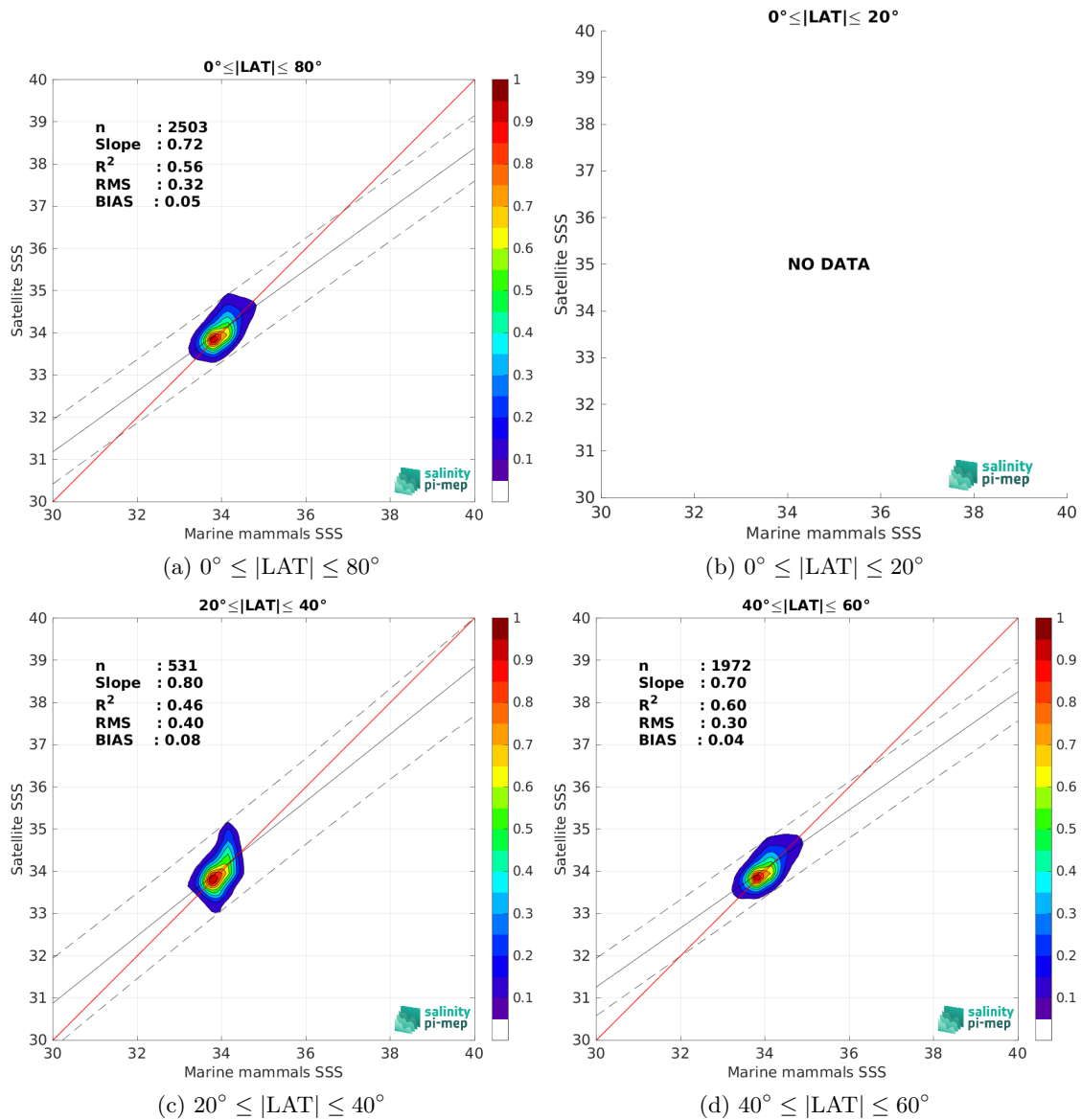
Figure 10: Contour maps of the concentration of CCI SSS L4 Merged-OI v5.5 - 30-day running (ESA) SSS (y-axis) versus Marine mammals SSS (x-axis) at match-up pairs for different latitude bands. For each plot, the red line shows x=y . The black thin and dashed lines indicate a linear fit through the data cloud and the \pm 95\% confidence levels, respectively. The number match-up pairs n , the slope and R^2 coefficient of the linear fit, the root mean square (RMS) and the mean bias between satellite and in situ data are indicated for each latitude band in each plots.
