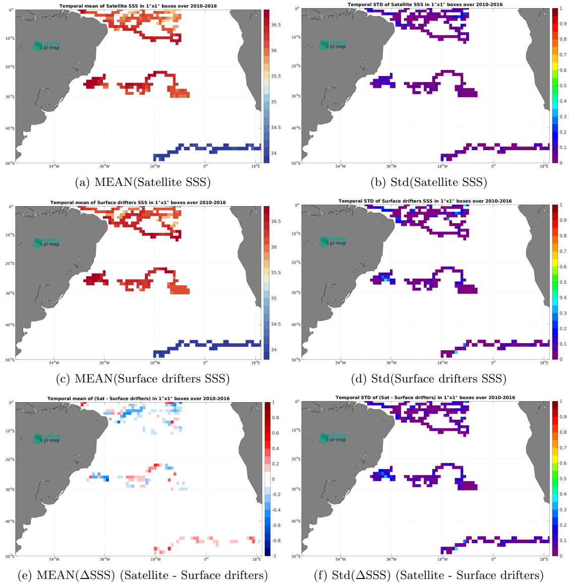
Figure 6: Temporal mean (left) and Std (right) of SSS from CCI SSS L4 Merged-OI v5.5 - 30-day running (ESA) (top), Surface drifters (middle), and of \Delta SSS (Satellite - Surface drifters). Only match-up pairs are used to generate these maps.
