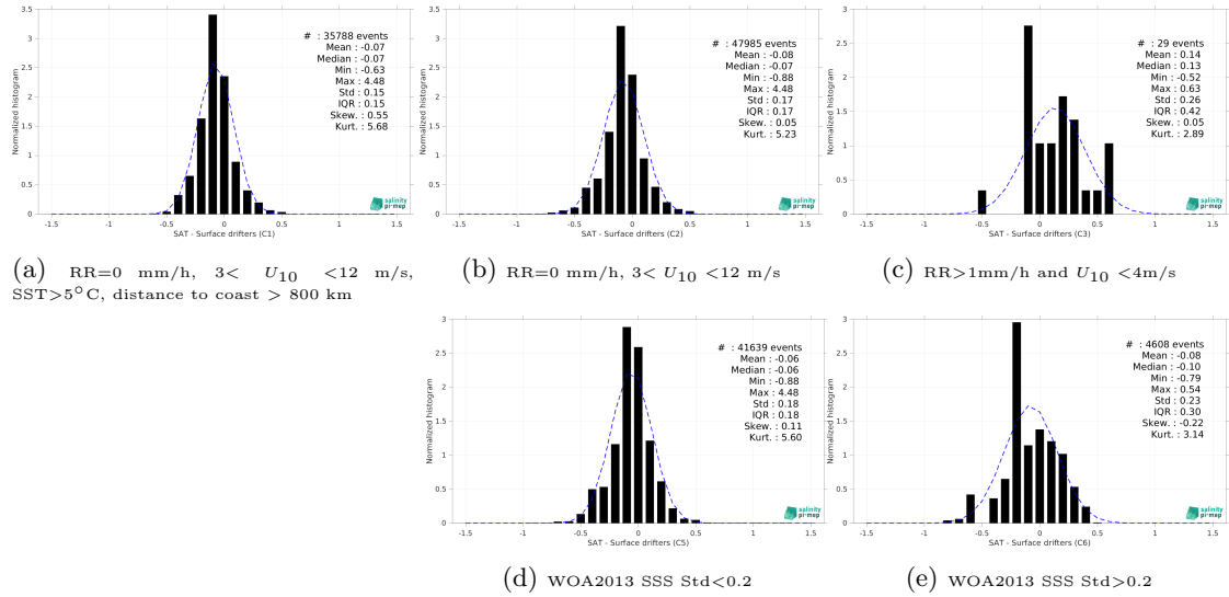
Figure 14: Normalized histogram of \Delta SSS (CCI SSS L4 Merged-OI v5.5 - 30-day running (ESA) - Surface drifters) for 5 different subdatasets corresponding to: RR=0 mm/h, 3 < U_{10} < 12 m/s, SST>5°C, distance to coast > 800 km (a), RR=0 mm/h, 3 < U_{10} < 12 m/s (b), RR>1mm/h and U_{10} < 4 m/s (c), WOA2013 SSS Std<0.2 (d), WOA2013 SSS Std>0.2 (e).
