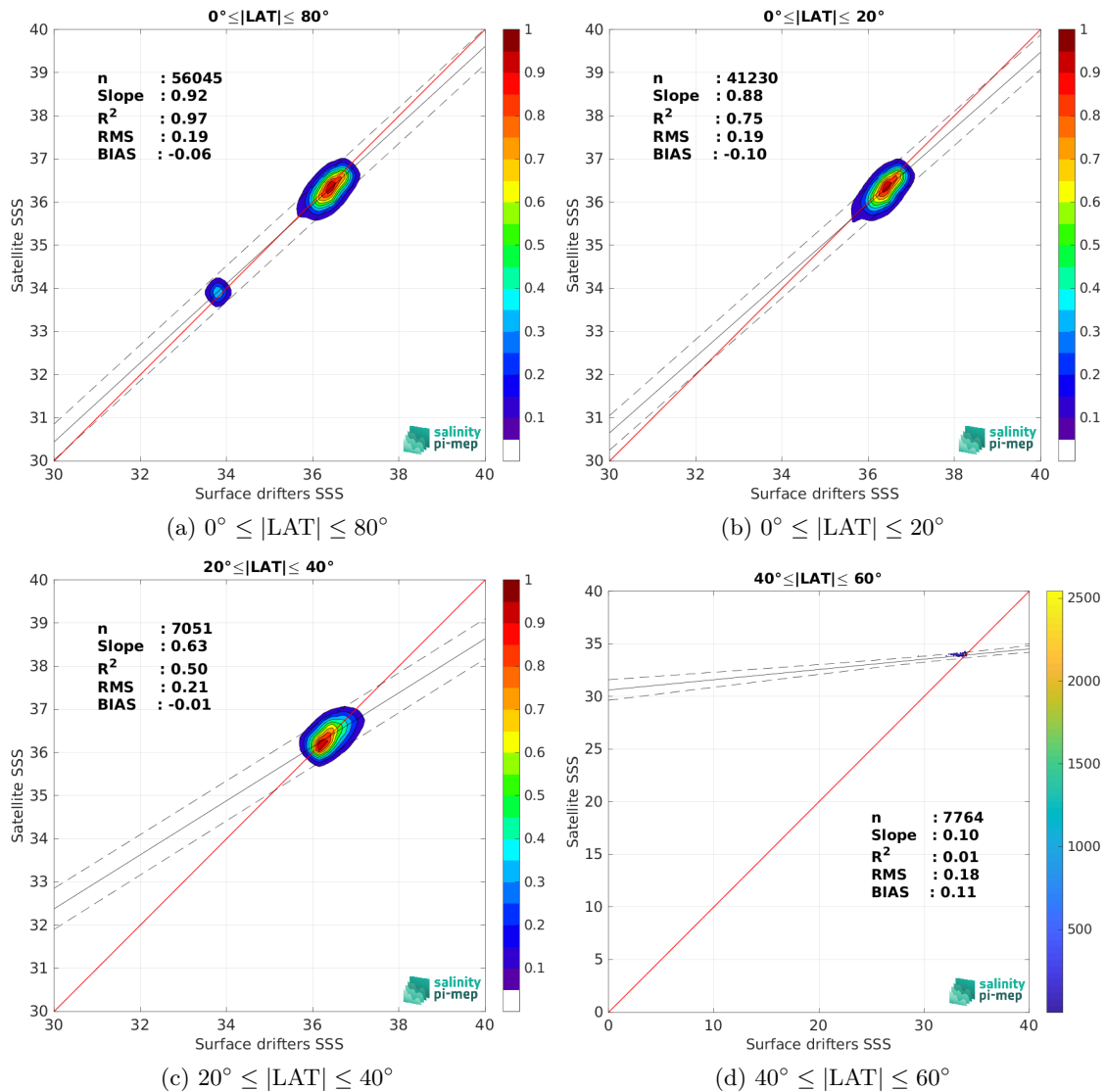
Figure 9: Contour maps of the concentration of CCI SSS L4 Merged-OI v5.5 - 30-day running (ESA) SSS (y-axis) versus Surface drifters SSS (x-axis) at match-up pairs for different latitude bands. For each plot, the red line shows x=y . The black thin and dashed lines indicate a linear fit through the data cloud and the \pm 95\% confidence levels, respectively. The number match-up pairs n , the slope and R^2 coefficient of the linear fit, the root mean square (RMS) and the mean bias between satellite and in situ data are indicated for each latitude band in each plots.
