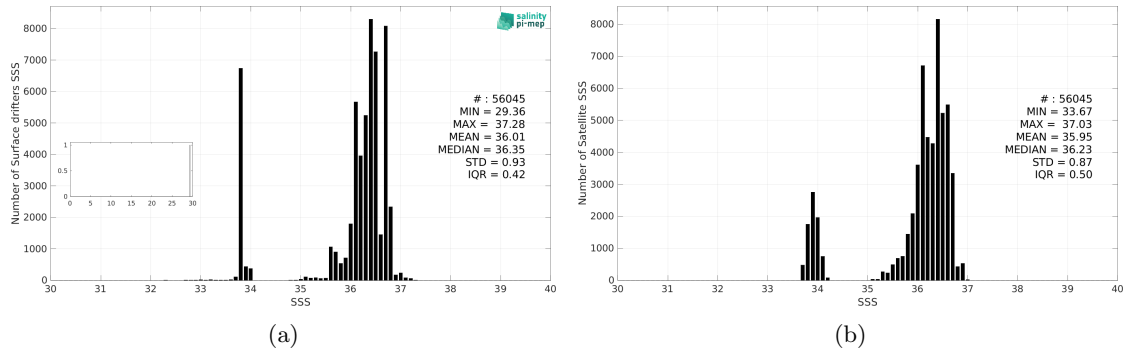
Figure 3: Histograms of SSS from Surface drifters (a) and CCI SSS L4 Merged-OI v5.5 - 30-day running (ESA) (b) considering all match-up pairs per bins of 0.1 over the South Atlantic Ocean Pi-MEP region and for the full satellite product period.
