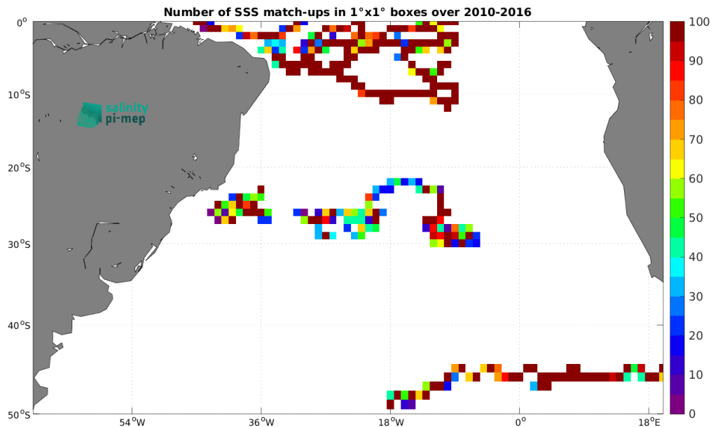
Figure 4: Number of SSS match-ups between Surface drifters SSS and the CCI SSS L4 Merged-OI v5.5 - 30-day running (ESA) SSS product for the South Atlantic Ocean Pi-MEP region over 1^\circ \times 1^\circ boxes and for the full satellite product period.
