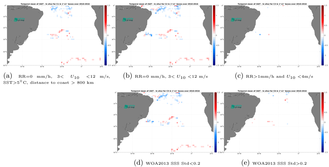
Figure 13: Temporal mean gridded over spatial boxes of size 1^\circ \times 1^\circ of \Delta\text{SSS} (CCI SSS L4 Merged-OI v5.5 - 30-day running (ESA) - Surface drifters) for 5 different subdatasets corresponding to:RR=0 mm/h, 3 < U_{10} < 12 m/s, SST >5^\circ\text{C} , distance to coast > 800 km (a), RR=0 mm/h, 3 < U_{10} < 12 m/s (b), RR >1 mm/h and U_{10} < 4 m/s (c), WOA2013 SSS Std <0.2 (d), WOA2013 SSS Std >0.2 (e).
