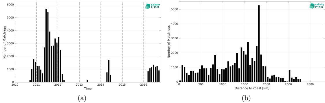
Figure 2: Number of match-ups between Surface drifters and CCI SSS L4 Merged-OI v5.5 - 30-day running (ESA) SSS as a function of time (a) and as function of the distance to coast (b) over the South Atlantic Ocean Pi-MEP region and for the full satellite product period.
