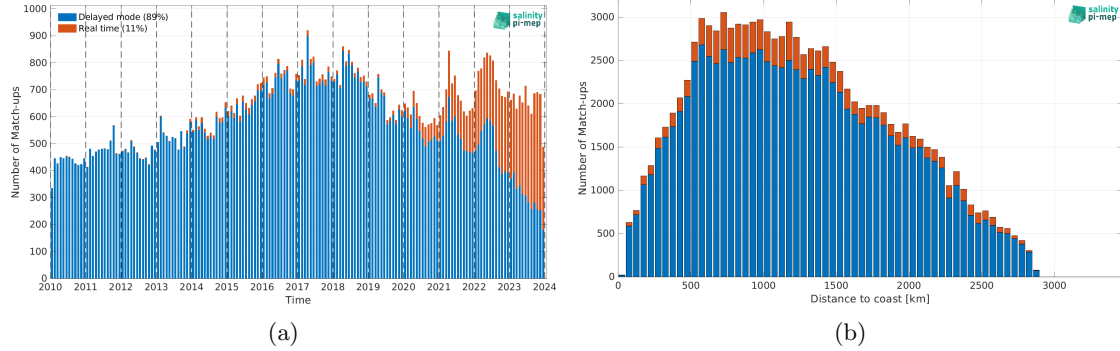
Figure 2: Number of match-ups between Argo and CCI SSS L4 Merged-OI v5.5 - 30-day running (ESA) SSS as a function of time (a) and as function of the distance to coast (b) over the South Atlantic Ocean Pi-MEP region and for the full satellite product period.
