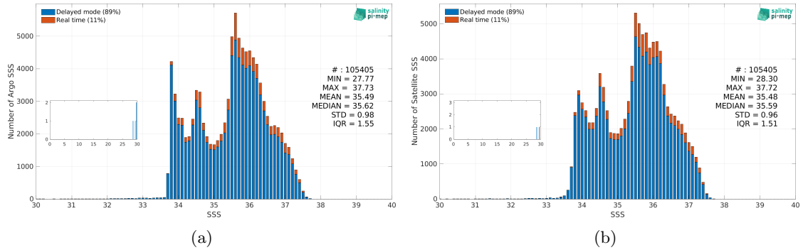
Figure 3: Histograms of SSS from Argo (a) and CCI SSS L4 Merged-OI v5.5 - 30-day running (ESA) (b) considering all match-up pairs per bins of 0.1 over the South Atlantic Ocean Pi-MEP region and for the full satellite product period.
