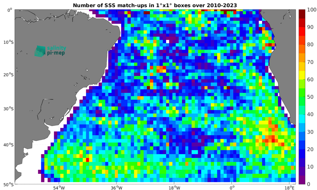
Figure 5: Number of SSS match-ups between Argo SSS and the CCI SSS L4 Merged-OI v5.5 - 30-day running (ESA) SSS product for the South Atlantic Ocean Pi-MEP region over 1^\circ \times 1^\circ boxes and for the full satellite product period.
