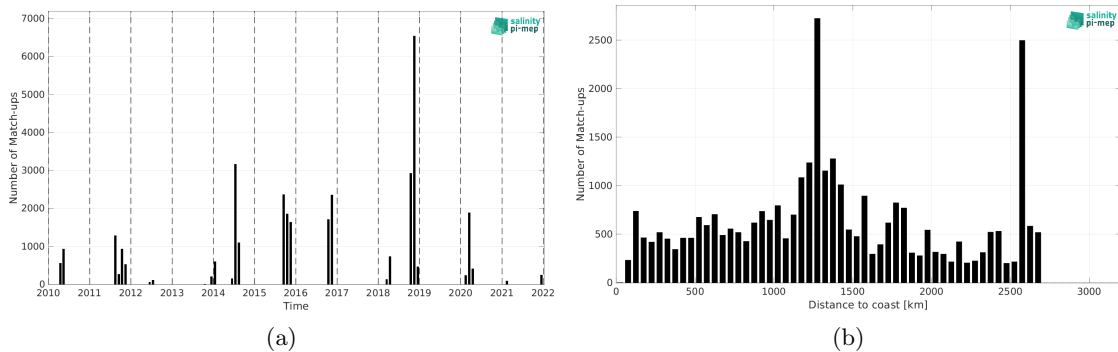
Figure 2: Number of match-ups between TSG (SAMOS) and CCI SSS L4 Merged-OI v4.41 - 7-day running (ESA) SSS as a function of time (a) and as function of the distance to coast (b) over the South Atlantic Ocean Pi-MEP region and for the full satellite product period.
