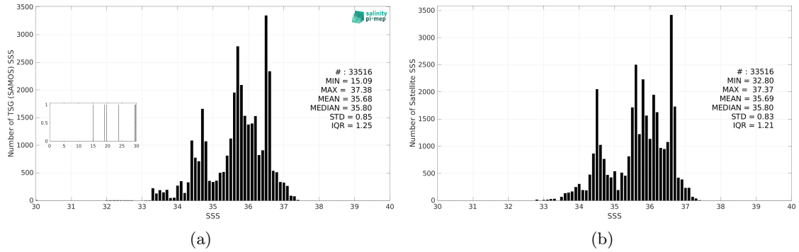
Figure 3: Histograms of SSS from TSG (SAMOS) (a) and CCI SSS L4 Merged-OI v4.41 - 7-day running (ESA) (b) considering all match-up pairs per bins of 0.1 over the South Atlantic Ocean Pi-MEP region and for the full satellite product period.
