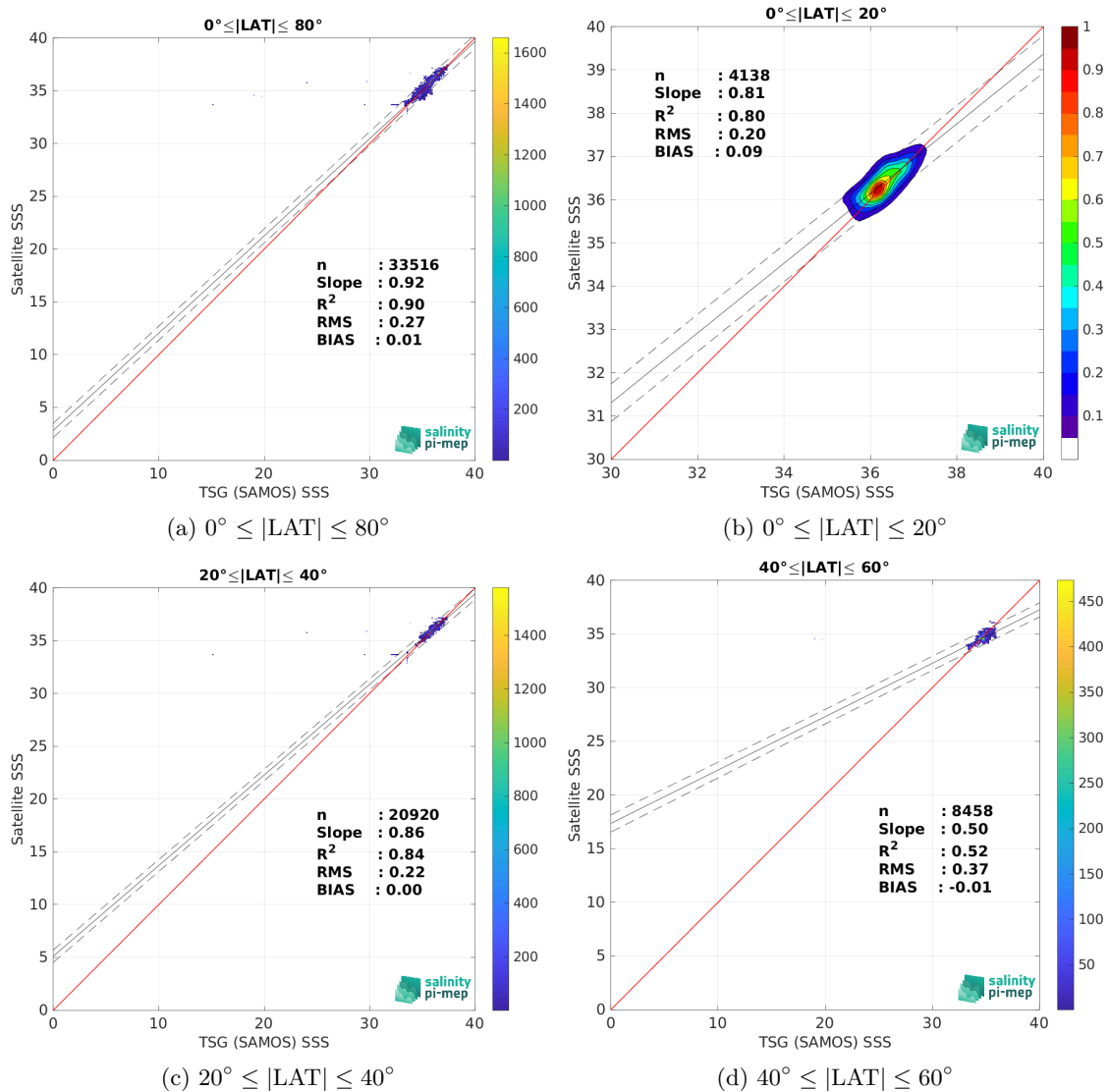
Figure 10: Contour maps of the concentration of CCI SSS L4 Merged-OI v4.41 - 7-day running (ESA) SSS (y-axis) versus TSG (SAMOS) SSS (x-axis) at match-up pairs for different latitude bands. For each plot, the red line shows x=y . The black thin and dashed lines indicate a linear fit through the data cloud and the \pm 95\% confidence levels, respectively. The number match-up pairs n , the slope and R^2 coefficient of the linear fit, the root mean square (RMS) and the mean bias between satellite and in situ data are indicated for each latitude band in each plots.
