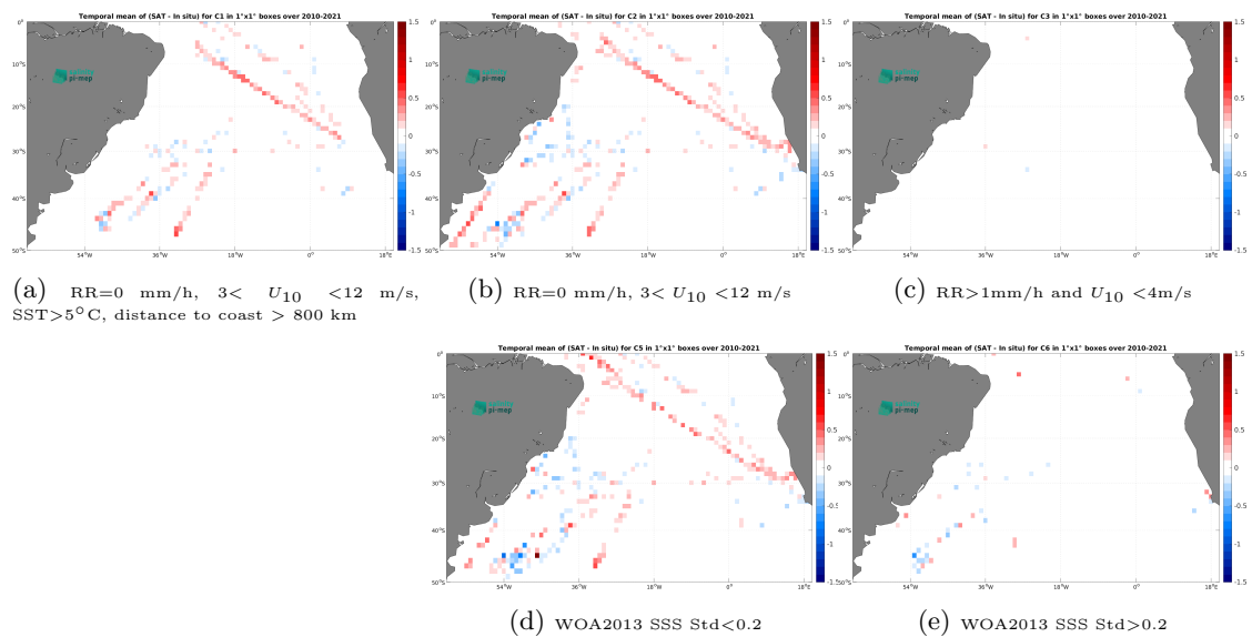
Figure 14: Temporal mean gridded over spatial boxes of size 1^\circ \times 1^\circ of \Delta\text{SSS} (CCI SSS L4 Merged-OI v4.41 - 7-day running (ESA) - TSG (SAMOS)) for 5 different subdatasets corresponding to:RR=0 mm/h, 3 < U_{10} < 12 m/s, SST >5^\circ\text{C} , distance to coast > 800 km (a), RR=0 mm/h, 3 < U_{10} < 12 m/s (b), RR >1 mm/h and U_{10} < 4 m/s (c), WOA2013 SSS Std <0.2 (d), WOA2013 SSS Std >0.2 (e).
