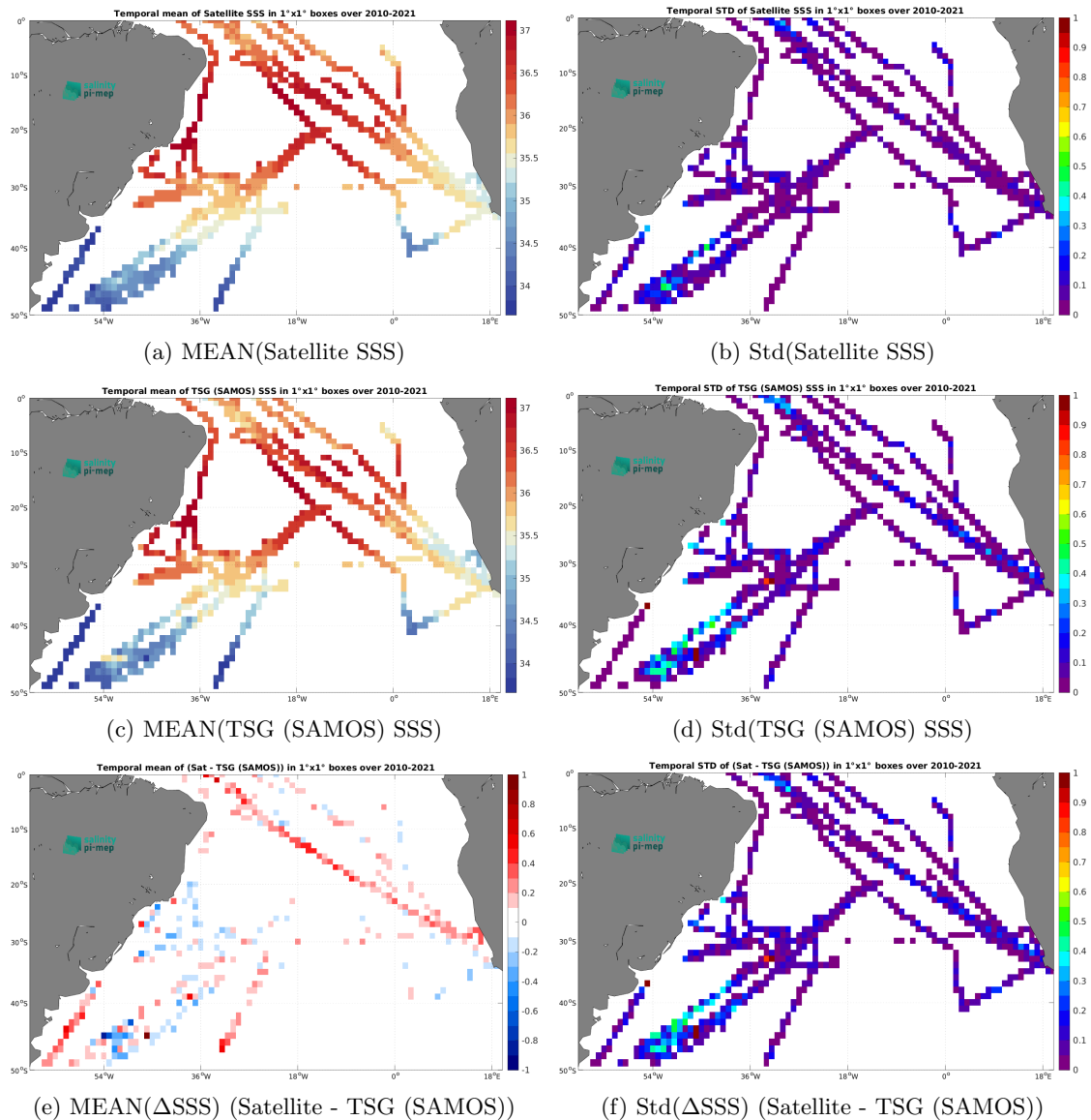
Figure 7: Temporal mean (left) and Std (right) of SSS from CCI SSS L4 Merged-OI v4.41 - 7-day running (ESA) (top), TSG (SAMOS) (middle), and of \Delta SSS (Satellite - TSG (SAMOS)). Only match-up pairs are used to generate these maps.
