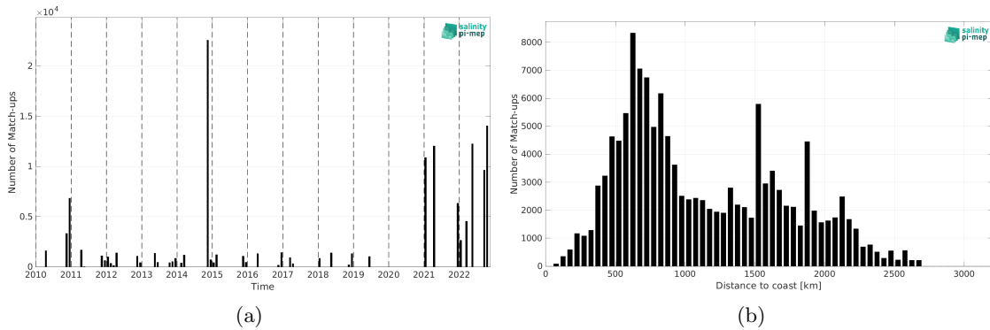
Figure 2: Number of match-ups between TSG (Polarstern) and CCI SSS L4 Merged-OI v4.41 - 7-day running (ESA) SSS as a function of time (a) and as function of the distance to coast (b) over the South Atlantic Ocean Pi-MEP region and for the full satellite product period.
