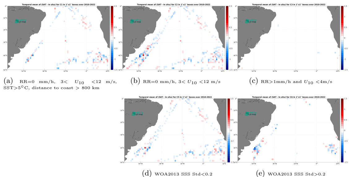
Figure 14: Temporal mean gridded over spatial boxes of size 1^\circ \times 1^\circ of \Delta\text{SSS} (CCI SSS L4 Merged-OI v4.41 - 7-day running (ESA) - TSG (Polarstern)) for 5 different subdatasets corresponding to:RR=0 mm/h, 3 < U_{10} < 12 m/s, SST >5^\circ\text{C} , distance to coast > 800 km (a), RR=0 mm/h, 3 < U_{10} < 12 m/s (b), RR >1 mm/h and U_{10} < 4 m/s (c), WOA2013 SSS Std <0.2 (d), WOA2013 SSS Std >0.2 (e).
