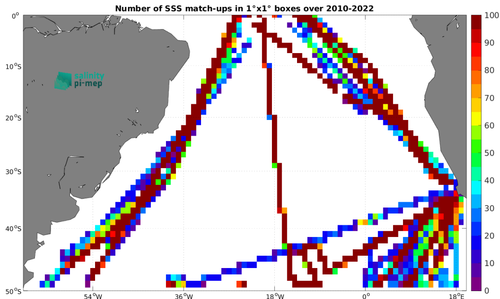
Figure 5: Number of SSS match-ups between TSG (Polarstern) SSS and the CCI SSS L4 Merged-OI v4.41 - 7-day running (ESA) SSS product for the South Atlantic Ocean Pi-MEP region over 1^\circ \times 1^\circ boxes and for the full satellite product period.
