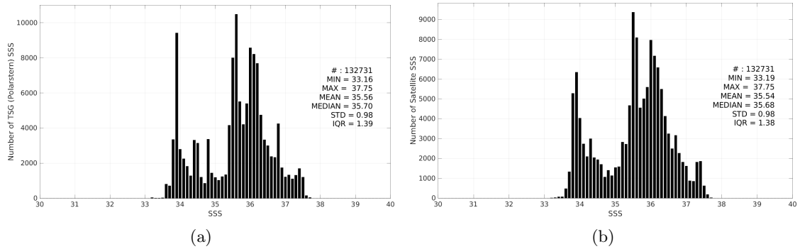
Figure 3: Histograms of SSS from TSG (Polarstern) (a) and CCI SSS L4 Merged-OI v4.41 - 7-day running (ESA) (b) considering all match-up pairs per bins of 0.1 over the South Atlantic Ocean Pi-MEP region and for the full satellite product period.
