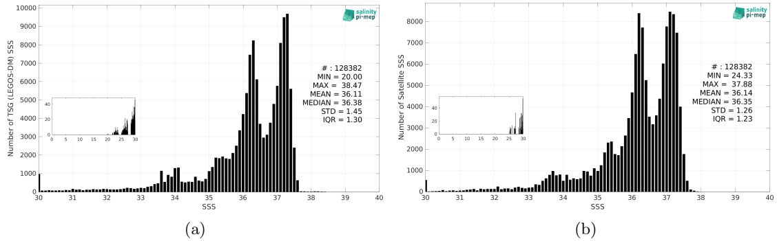
Figure 3: Histograms of SSS from TSG (LEGOS-DM) (a) and CCI SSS L4 Merged-OI v4.41 - 7-day running (ESA) (b) considering all match-up pairs per bins of 0.1 over the South Atlantic Ocean Pi-MEP region and for the full satellite product period.
