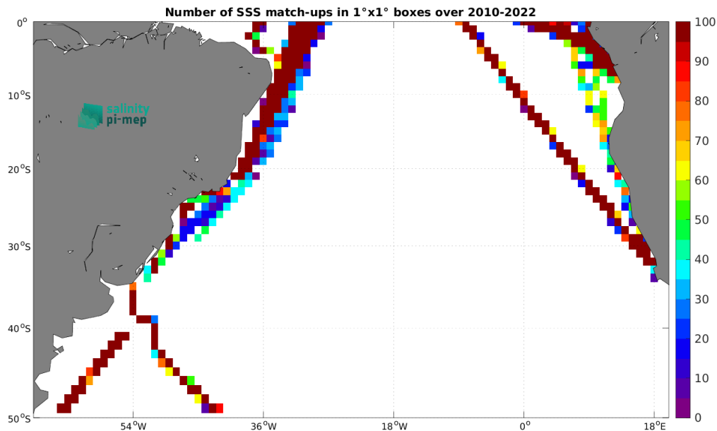
Figure 5: Number of SSS match-ups between TSG (LEGOS-DM) SSS and the CCI SSS L4 Merged-OI v4.41 - 7-day running (ESA) SSS product for the South Atlantic Ocean Pi-MEP region over 1^\circ \times 1^\circ boxes and for the full satellite product period.
