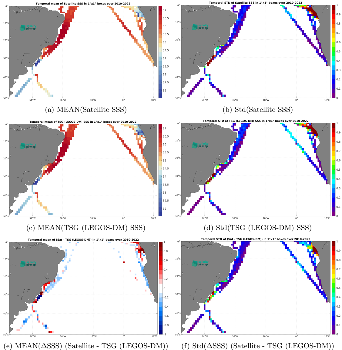
Figure 7: Temporal mean (left) and Std (right) of SSS from CCI SSS L4 Merged-OI v4.41 - 7-day running (ESA) (top), TSG (LEGOS-DM) (middle), and of \Delta SSS (Satellite - TSG (LEGOS-DM)). Only match-up pairs are used to generate these maps.
