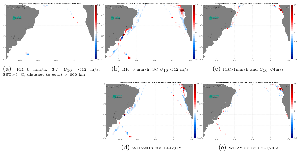
Figure 14: Temporal mean gridded over spatial boxes of size 1^\circ \times 1^\circ of \Delta\text{SSS} (CCI SSS L4 Merged-OI v4.41 - 7-day running (ESA) - TSG (LEGOS-DM)) for 5 different subdatasets corresponding to:RR=0 mm/h, 3 < U_{10} < 12 m/s, SST >5^\circ\text{C} , distance to coast > 800 km (a), RR=0 mm/h, 3 < U_{10} < 12 m/s (b), RR >1 mm/h and U_{10} < 4 m/s (c), WOA2013 SSS Std <0.2 (d), WOA2013 SSS Std >0.2 (e).
