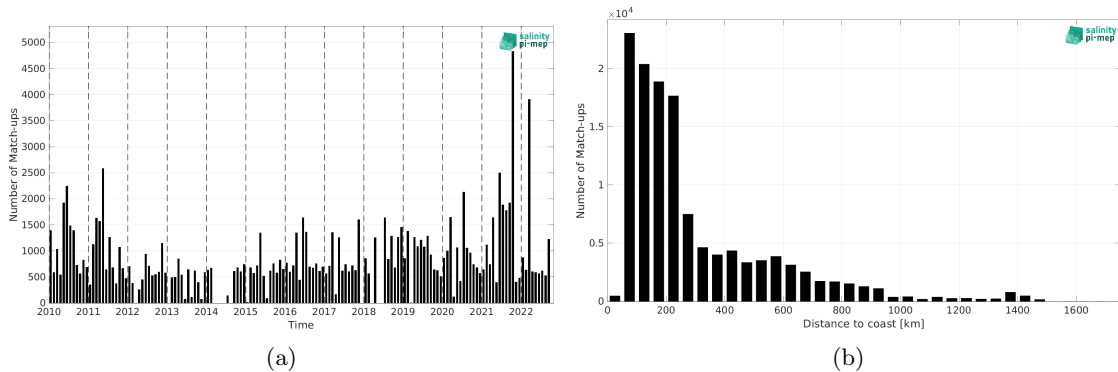
Figure 2: Number of match-ups between TSG (LEGOS-DM) and CCI SSS L4 Merged-OI v4.41 - 7-day running (ESA) SSS as a function of time (a) and as function of the distance to coast (b) over the South Atlantic Ocean Pi-MEP region and for the full satellite product period.
