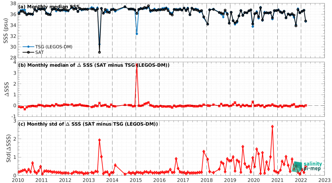
Figure 8: Time series of the monthly median SSS (top), median of \Delta\text{SSS} (Satellite - TSG (LEGOS-DM)) and Std of \Delta\text{SSS} (Satellite - TSG (LEGOS-DM)) over the South Atlantic Ocean Pi-MEP region considering all match-ups collected by the Pi-MEP.
