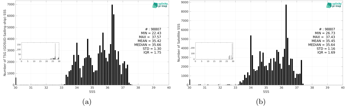
Figure 3: Histograms of SSS from TSG (GOSUD-Sailing-ship) (a) and CCI SSS L4 Merged-OI v4.41 - 7-day running (ESA) (b) considering all match-up pairs per bins of 0.1 over the South Atlantic Ocean Pi-MEP region and for the full satellite product period.
