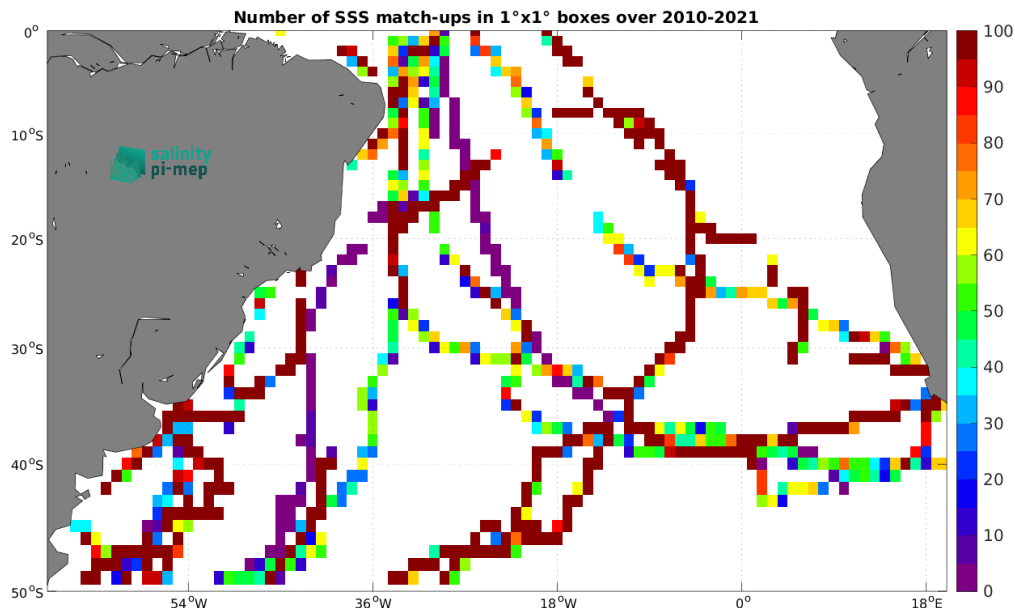
Figure 5: Number of SSS match-ups between TSG (GOSUD-Sailing-ship) SSS and the CCI SSS L4 Merged-OI v4.41 - 7-day running (ESA) SSS product for the South Atlantic Ocean Pi-MEP region over 1^\circ \times 1^\circ boxes and for the full satellite product period.
