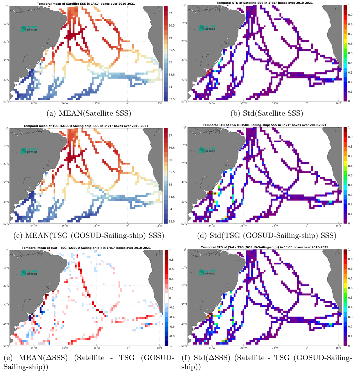
Figure 7: Temporal mean (left) and Std (right) of SSS from CCI SSS L4 Merged-OI v4.41 - 7-day running (ESA) (top), TSG (GOSUD-Sailing-ship) (middle), and of \Delta SSS (Satellite - TSG (GOSUD-Sailing-ship)). Only match-up pairs are used to generate these maps.
