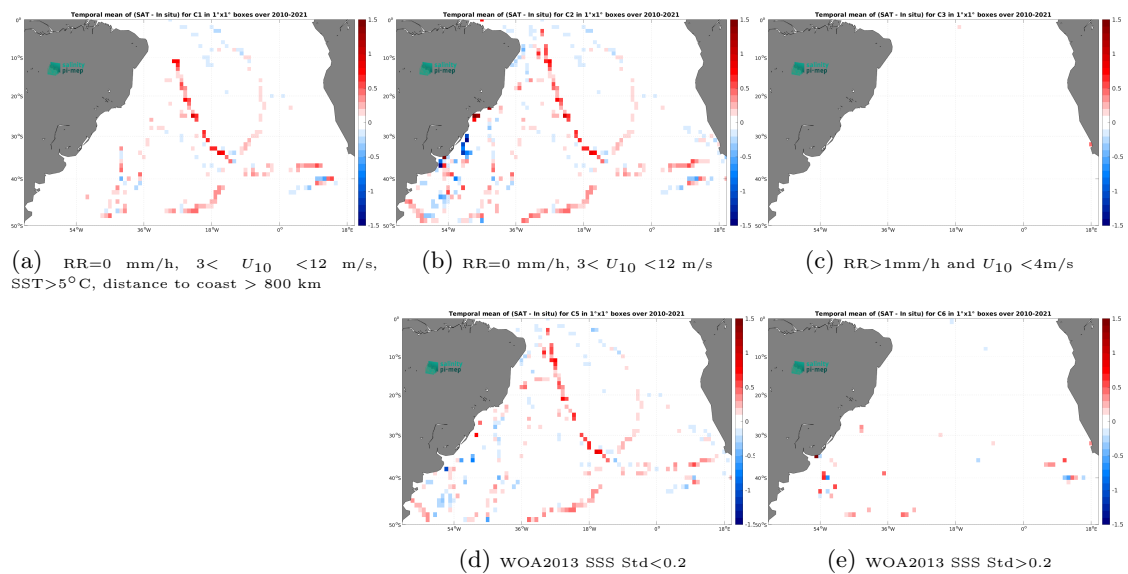
Figure 14: Temporal mean gridded over spatial boxes of size 1^\circ \times 1^\circ of \Delta\text{SSS} (CCI SSS L4 Merged-OI v4.41 - 7-day running (ESA) - TSG (GOSUD-Sailing-ship)) for 5 different subdatasets corresponding to:RR=0 mm/h, 3 < U_{10} < 12 m/s, SST >5^\circ\text{C} , distance to coast > 800 km (a), RR=0 mm/h, 3 < U_{10} < 12 m/s (b), RR >1 mm/h and U_{10} < 4 m/s (c), WOA2013 SSS Std <0.2 (d), WOA2013 SSS Std >0.2 (e).
