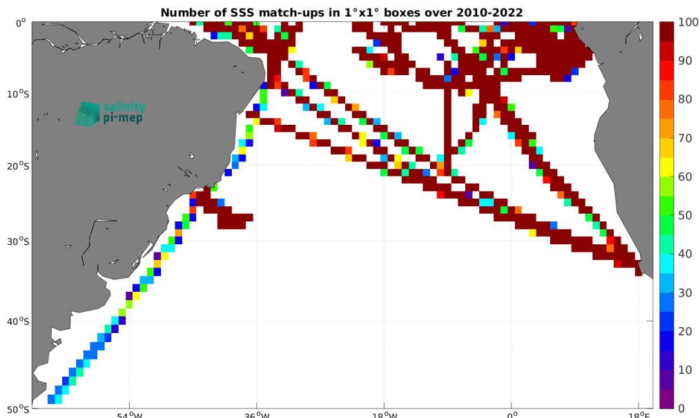
Figure 5: Number of SSS match-ups between TSG (GOSUD-Research-vessel) SSS and the CCI SSS L4 Merged-OI v4.41 - 7-day running (ESA) SSS product for the South Atlantic Ocean Pi-MEP region over 1^\circ \times 1^\circ boxes and for the full satellite product period.
