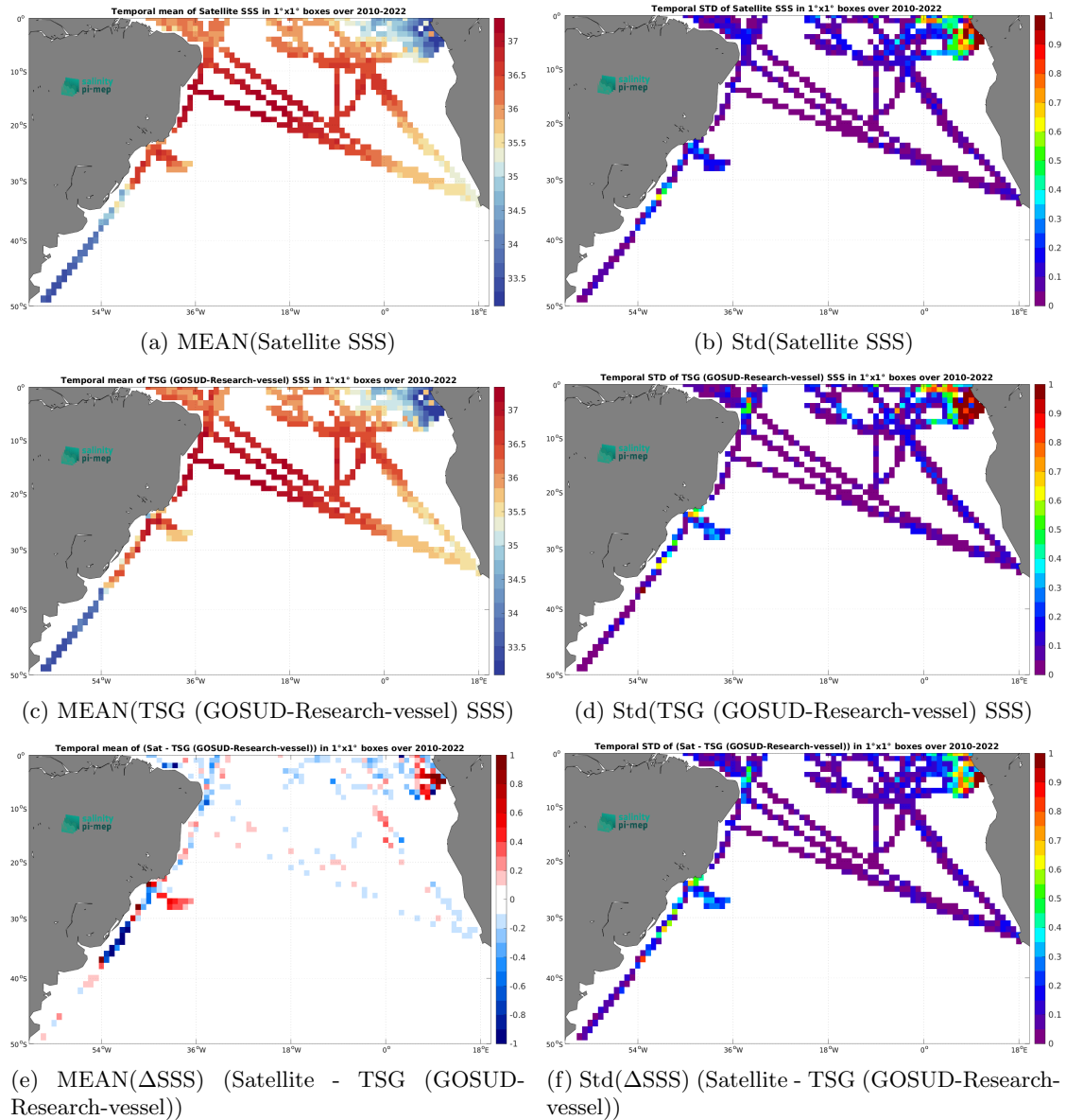
Figure 7: Temporal mean (left) and Std (right) of SSS from CCI SSS L4 Merged-OI v4.41 - 7-day running (ESA) (top), TSG (GOSUD-Research-vessel) (middle), and of \Delta SSS (Satellite - TSG (GOSUD-Research-vessel)). Only match-up pairs are used to generate these maps.
