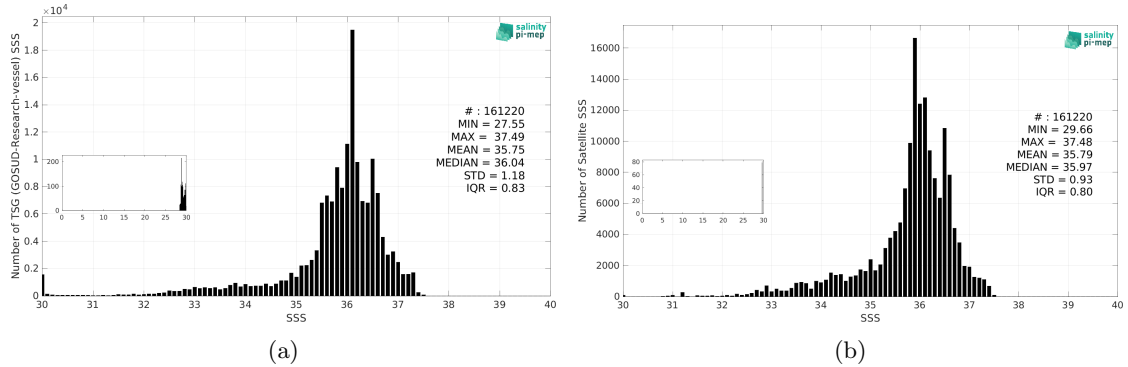
Figure 3: Histograms of SSS from TSG (GOSUD-Research-vessel) (a) and CCI SSS L4 Merged-OI v4.41 - 7-day running (ESA) (b) considering all match-up pairs per bins of 0.1 over the South Atlantic Ocean Pi-MEP region and for the full satellite product period.
