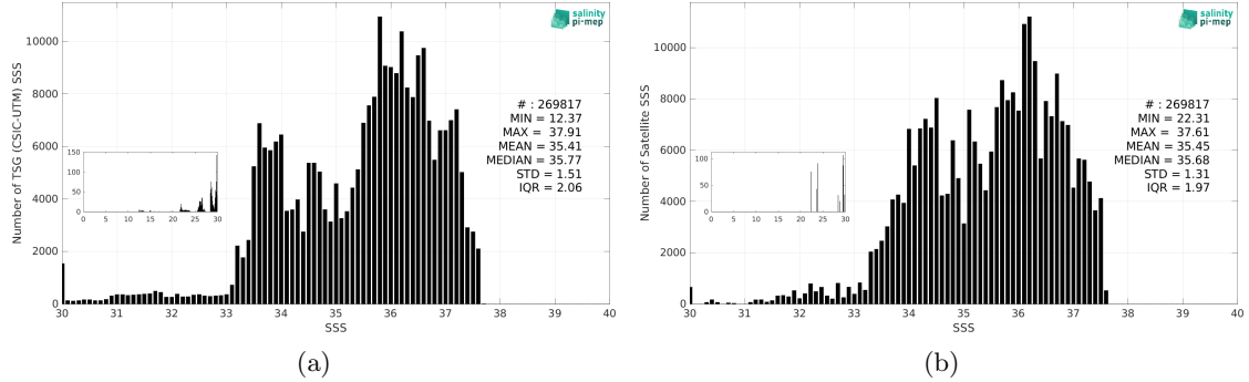
Figure 3: Histograms of SSS from TSG (CSIC-UTM) (a) and CCI SSS L4 Merged-OI v4.41 - 7-day running (ESA) (b) considering all match-up pairs per bins of 0.1 over the South Atlantic Ocean Pi-MEP region and for the full satellite product period.
