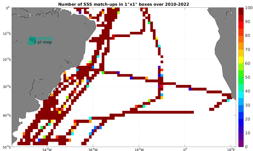
Figure 5: Number of SSS match-ups between TSG (CSIC-UTM) SSS and the CCI SSS L4 Merged-OI v4.41 - 7-day running (ESA) SSS product for the South Atlantic Ocean Pi-MEP region over 1^\circ \times 1^\circ boxes and for the full satellite product period.
