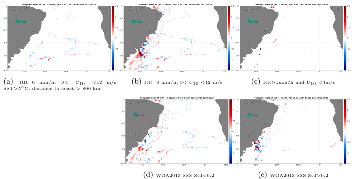
Figure 14: Temporal mean gridded over spatial boxes of size 1^\circ \times 1^\circ of \Delta\text{SSS} (CCI SSS L4 Merged-OI v4.41 - 7-day running (ESA) - TSG (CSIC-UTM)) for 5 different subdatasets corresponding to:RR=0 mm/h, 3 < U_{10} < 12 m/s, SST >5^\circ\text{C} , distance to coast > 800 km (a), RR=0 mm/h, 3 < U_{10} < 12 m/s (b), RR >1 mm/h and U_{10} < 4 m/s (c), WOA2013 SSS Std <0.2 (d), WOA2013 SSS Std >0.2 (e).
