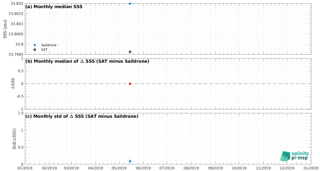
Figure 8: Time series of the monthly median SSS (top), median of \Delta SSS (Satellite - Sairdrone) and Std of \Delta SSS (Satellite - Sairdrone) over the South Atlantic Ocean Pi-MEP region considering all match-ups collected by the Pi-MEP.
