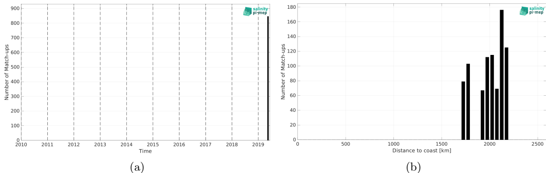
Figure 2: Number of match-ups between Saildrone and CCI SSS L4 Merged-OI v4.41 - 7-day running (ESA) SSS as a function of time (a) and as function of the distance to coast (b) over the South Atlantic Ocean Pi-MEP region and for the full satellite product period.
