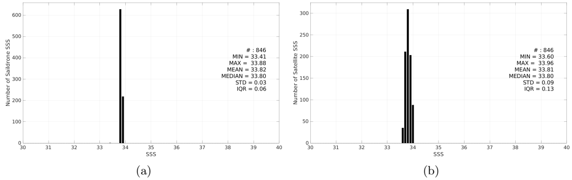
Figure 3: Histograms of SSS from Saildrone (a) and CCI SSS L4 Merged-OI v4.41 - 7-day running (ESA) (b) considering all match-up pairs per bins of 0.1 over the South Atlantic Ocean Pi-MEP region and for the full satellite product period.
