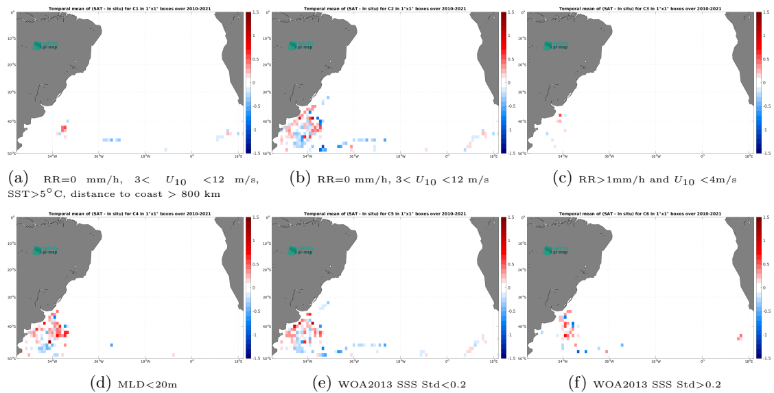
Figure 14: Temporal mean gridded over spatial boxes of size 1^\circ \times 1^\circ of \Delta SSS (CCI SSS L4 Merged-OI v4.41 - 7-day running (ESA) - Marine mammals) for 6 different subdatasets corresponding to:RR=0 mm/h, 3 < U_{10} < 12 m/s, SST >5^\circ C, distance to coast > 800 km (a), RR=0 mm/h, 3 < U_{10} < 12 m/s (b), RR >1 mm/h and U_{10} < 4 m/s (c),MLD <20 m (d),WOA2013 SSS Std <0.2 (e),WOA2013 SSS Std >0.2 (f).
