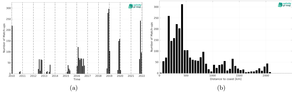
Figure 2: Number of match-ups between Marine mammals and CCI SSS L4 Merged-OI v4.41 - 7-day running (ESA) SSS as a function of time (a) and as function of the distance to coast (b) over the South Atlantic Ocean Pi-MEP region and for the full satellite product period.
