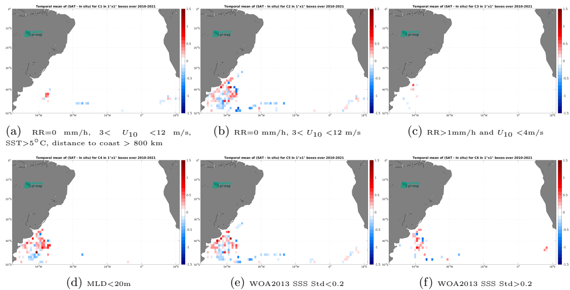
Figure 14: Temporal mean gridded over spatial boxes of size 1^\circ \times 1^\circ of \Delta\text{SSS} (CCI SSS L4 Merged-OI v4.41 - 7-day running (ESA) - Marine mammals) for 6 different subdatasets corresponding to:RR=0 mm/h, 3 < U_{10} < 12 m/s, SST>5°C, distance to coast > 800 km (a), RR=0 mm/h, 3 < U_{10} < 12 m/s (b), RR>1mm/h and U_{10} < 4 m/s (c),MLD<20m (d),WOA2013 SSS Std<0.2 (e),WOA2013 SSS Std>0.2 (f).
