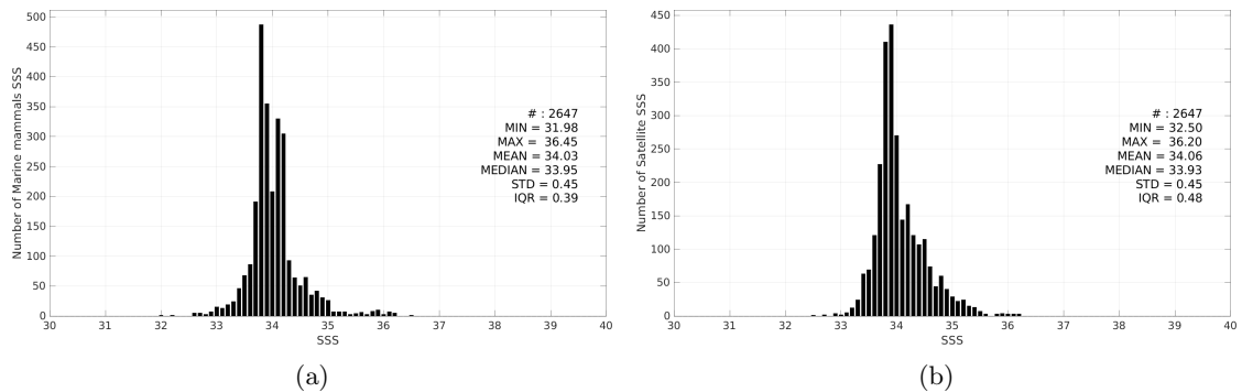
Figure 3: Histograms of SSS from Marine mammals (a) and CCI SSS L4 Merged-OI v4.41 - 7-day running (ESA) (b) considering all match-up pairs per bins of 0.1 over the South Atlantic Ocean Pi-MEP region and for the full satellite product period.
