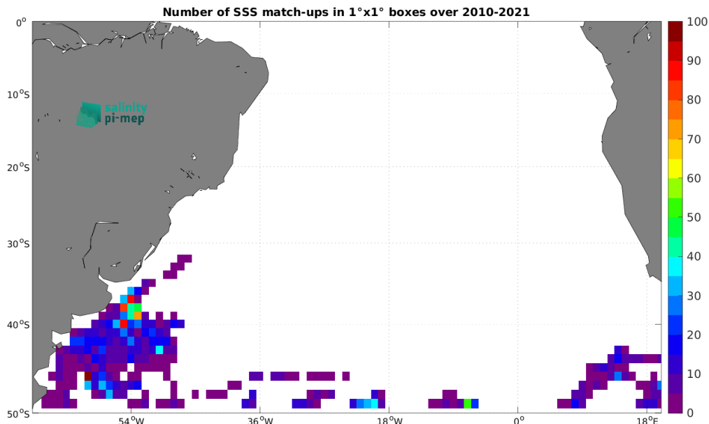
Figure 5: Number of SSS match-ups between Marine mammals SSS and the CCI SSS L4 Merged-OI v4.41 - 7-day running (ESA) SSS product for the South Atlantic Ocean Pi-MEP region over 1^\circ \times 1^\circ boxes and for the full satellite product period.
