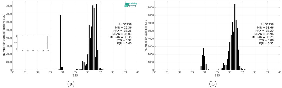
Figure 3: Histograms of SSS from Surface drifters (a) and CCI SSS L4 Merged-OI v4.41 - 7-day running (ESA) (b) considering all match-up pairs per bins of 0.1 over the South Atlantic Ocean Pi-MEP region and for the full satellite product period.
