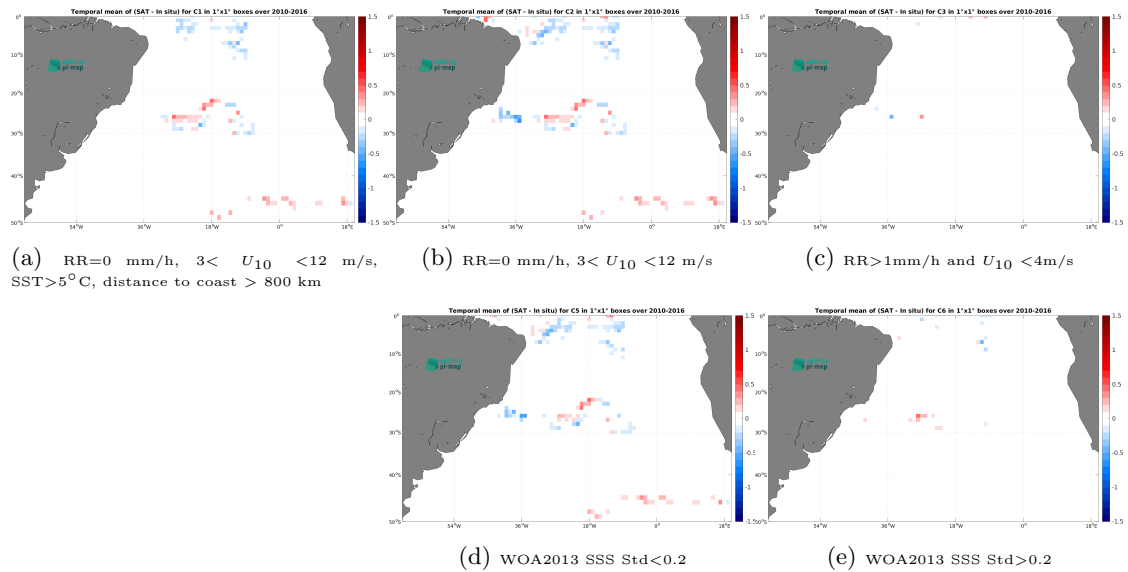
Figure 13: Temporal mean gridded over spatial boxes of size 1^\circ \times 1^\circ of \Delta SSS (CCI SSS L4 Merged-OI v4.41 - 7-day running (ESA) - Surface drifters) for 5 different subdatasets corresponding to:RR=0 mm/h, 3 < U_{10} < 12 m/s, SST >5^\circ\text{C} , distance to coast > 800 km (a), RR=0 mm/h, 3 < U_{10} < 12 m/s (b), RR >1 mm/h and U_{10} < 4 m/s (c), WOA2013 SSS Std <0.2 (d), WOA2013 SSS Std >0.2 (e).
