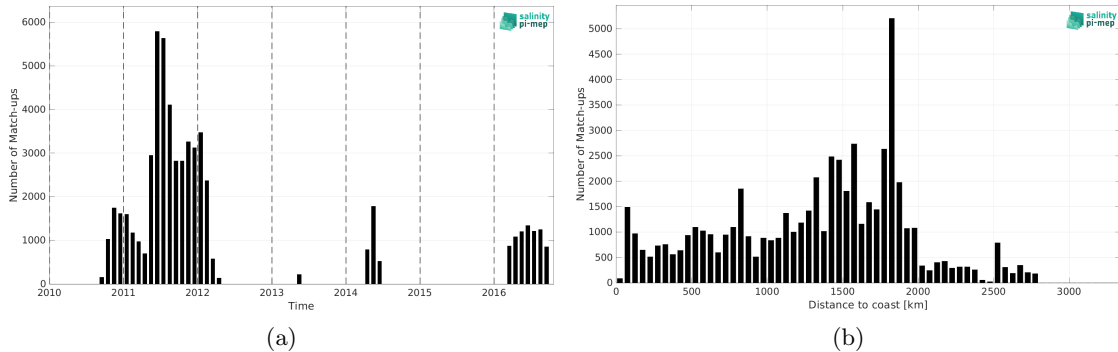
Figure 2: Number of match-ups between Surface drifters and CCI SSS L4 Merged-OI v4.41 - 7-day running (ESA) SSS as a function of time (a) and as function of the distance to coast (b) over the South Atlantic Ocean Pi-MEP region and for the full satellite product period.
