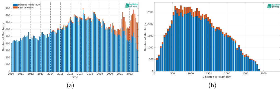
Figure 2: Number of match-ups between Argo and CCI SSS L4 Merged-OI v4.41 - 7-day running (ESA) SSS as a function of time (a) and as function of the distance to coast (b) over the South Atlantic Ocean Pi-MEP region and for the full satellite product period.
