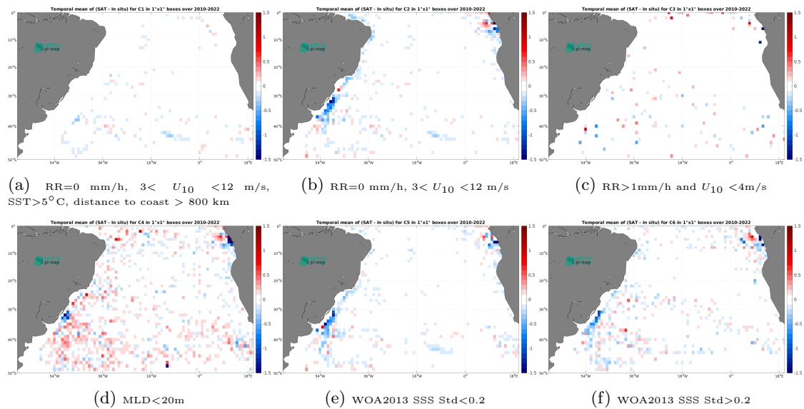
Figure 14: Temporal mean gridded over spatial boxes of size 1^\circ \times 1^\circ of \Delta\text{SSS} (CCI SSS L4 Merged-OI v4.41 - 7-day running (ESA) - Argo) for 6 different subdatasets corresponding to: RR=0 mm/h, 3 < U_{10} < 12 m/s, SST > 5°C, distance to coast > 800 km (a), RR=0 mm/h, 3 < U_{10} < 12 m/s (b), RR > 1mm/h and U_{10} < 4 m/s (c), MLD < 20m (d), WOA2013 SSS Std < 0.2 (e), WOA2013 SSS Std > 0.2 (f).
