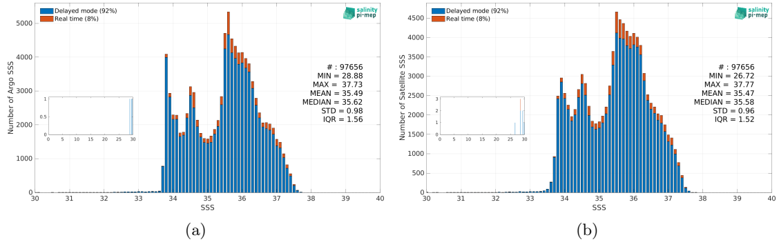
Figure 3: Histograms of SSS from Argo (a) and CCI SSS L4 Merged-OI v4.41 - 7-day running (ESA) (b) considering all match-up pairs per bins of 0.1 over the South Atlantic Ocean Pi-MEP region and for the full satellite product period.
