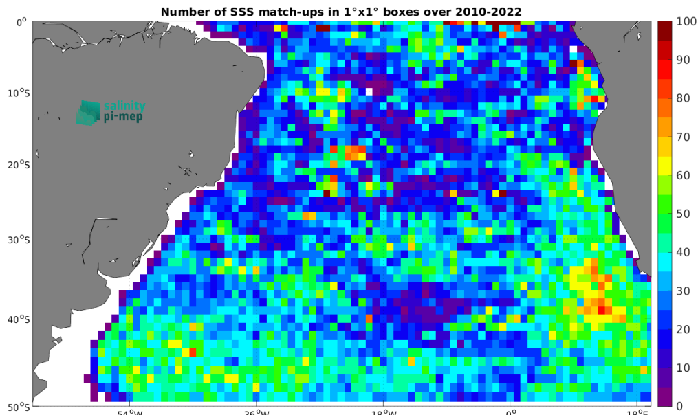
Figure 5: Number of SSS match-ups between Argo SSS and the CCI SSS L4 Merged-OI v4.41 - 7-day running (ESA) SSS product for the South Atlantic Ocean Pi-MEP region over 1^\circ \times 1^\circ boxes and for the full satellite product period.
