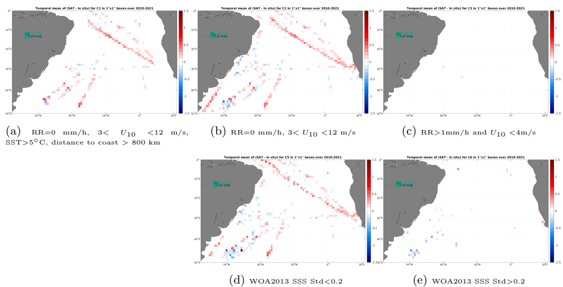
Figure 14: Temporal mean gridded over spatial boxes of size 1^\circ \times 1^\circ of \Delta\text{SSS} (CCI SSS L4 Merged-OI v4.41 - 30-day running (ESA) - TSG (SAMOS)) for 5 different subdatasets corresponding to:RR=0 mm/h, 3 < U_{10} < 12 m/s, SST >5^\circ\text{C} , distance to coast > 800 km (a), RR=0 mm/h, 3 < U_{10} < 12 m/s (b), RR >1 mm/h and U_{10} < 4 m/s (c), WOA2013 SSS Std <0.2 (d), WOA2013 SSS Std >0.2 (e).
