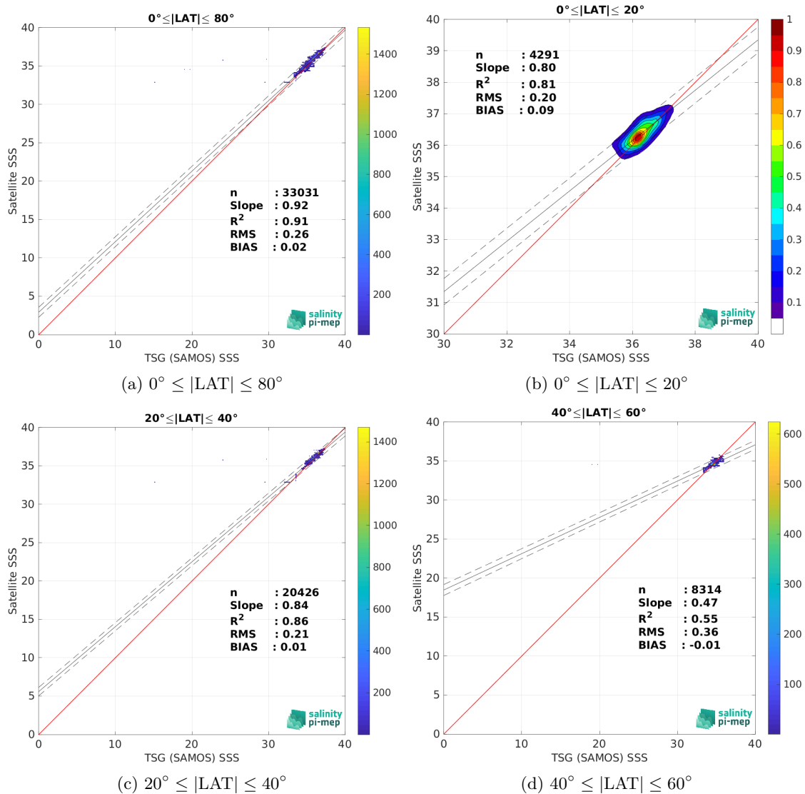
Figure 10: Contour maps of the concentration of CCI SSS L4 Merged-OI v4.41 - 30-day running (ESA) SSS (y-axis) versus TSG (SAMOS) SSS (x-axis) at match-up pairs for different latitude bands. For each plot, the red line shows x=y . The black thin and dashed lines indicate a linear fit through the data cloud and the \pm 95\% confidence levels, respectively. The number match-up pairs n , the slope and R^2 coefficient of the linear fit, the root mean square (RMS) and the mean bias between satellite and in situ data are indicated for each latitude band in each plots.
