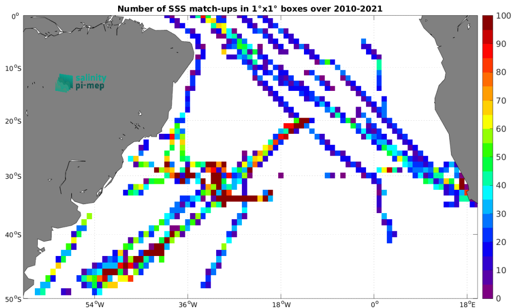
Figure 5: Number of SSS match-ups between TSG (SAMOS) SSS and the CCI SSS L4 Merged-OI v4.41 - 30-day running (ESA) SSS product for the South Atlantic Ocean Pi-MEP region over 1^\circ \times 1^\circ boxes and for the full satellite product period.
