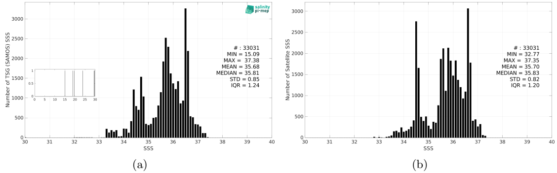
Figure 3: Histograms of SSS from TSG (SAMOS) (a) and CCI SSS L4 Merged-OI v4.41 - 30-day running (ESA) (b) considering all match-up pairs per bins of 0.1 over the South Atlantic Ocean Pi-MEP region and for the full satellite product period.
