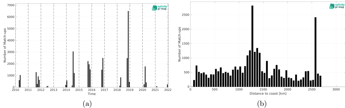
Figure 2: Number of match-ups between TSG (SAMOS) and CCI SSS L4 Merged-OI v4.41 - 30-day running (ESA) SSS as a function of time (a) and as function of the distance to coast (b) over the South Atlantic Ocean Pi-MEP region and for the full satellite product period.
