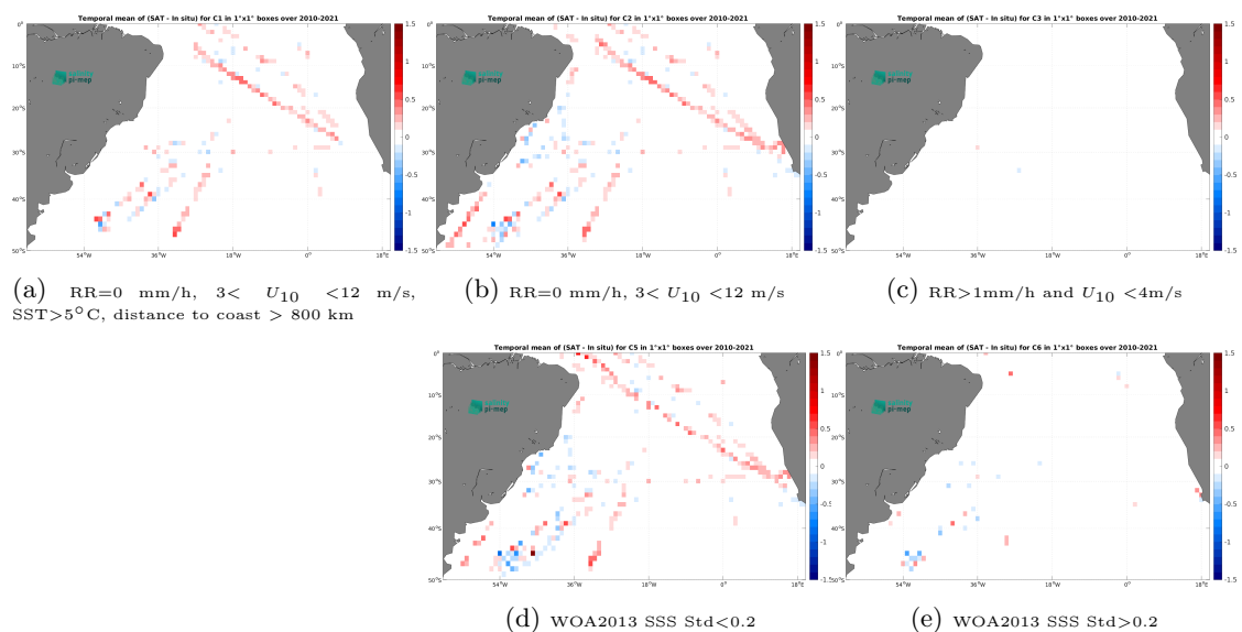
Figure 14: Temporal mean gridded over spatial boxes of size 1^\circ \times 1^\circ of \Delta\text{SSS} (CCI SSS L4 Merged-OI v4.41 - 30-day running (ESA) - TSG (SAMOS)) for 5 different subdatasets corresponding to:RR=0 mm/h, 3 < U_{10} < 12 m/s, SST >5^\circ\text{C} , distance to coast > 800 km (a), RR=0 mm/h, 3 < U_{10} < 12 m/s (b), RR >1 mm/h and U_{10} < 4 m/s (c), WOA2013 SSS Std <0.2 (d), WOA2013 SSS Std >0.2 (e).
