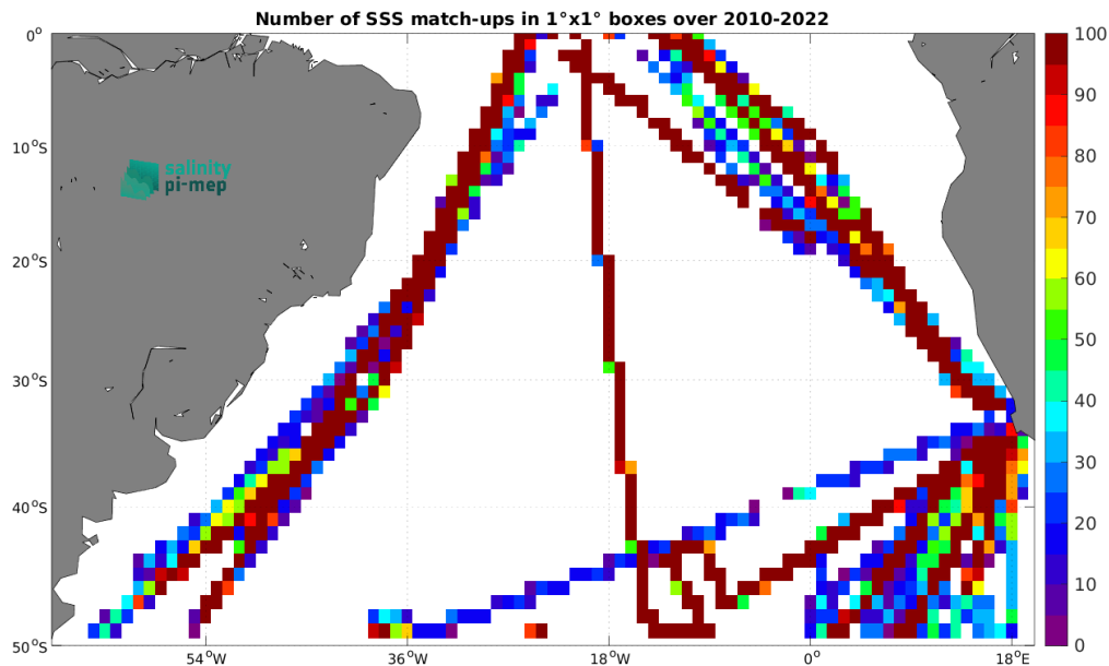
Figure 5: Number of SSS match-ups between TSG (Polarstern) SSS and the CCI SSS L4 Merged-OI v4.41 - 30-day running (ESA) SSS product for the South Atlantic Ocean Pi-MEP region over 1^\circ \times 1^\circ boxes and for the full satellite product period.
