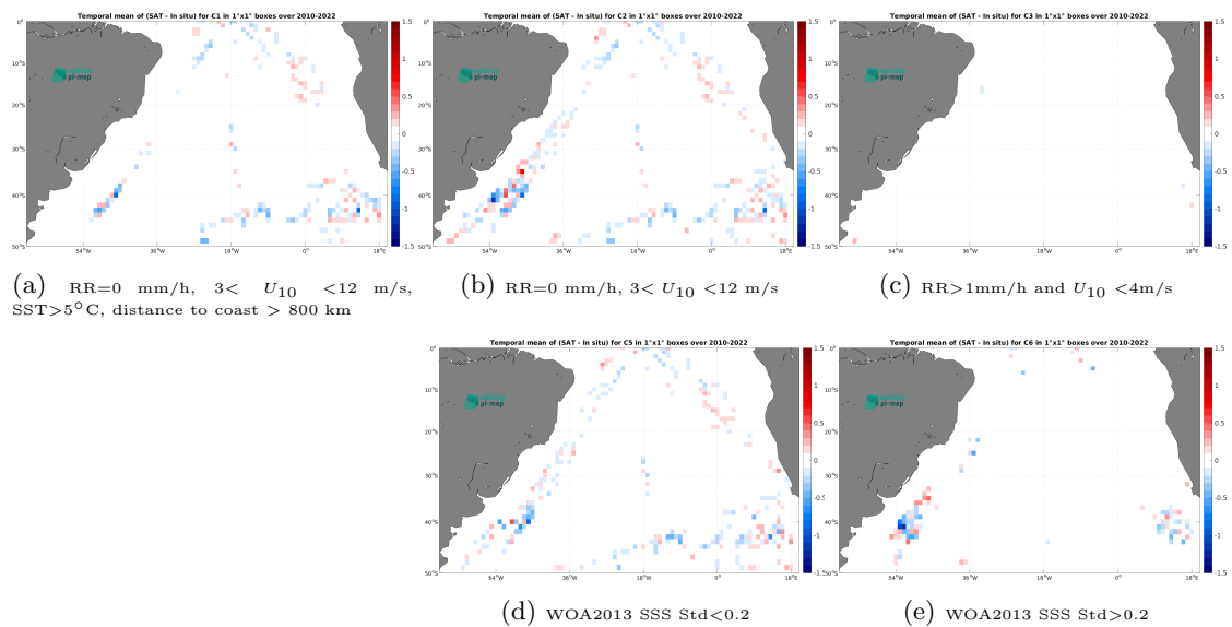
Figure 14: Temporal mean gridded over spatial boxes of size 1^\circ \times 1^\circ of \Delta\text{SSS} (CCI SSS L4 Merged-OI v4.41 - 30-day running (ESA) - TSG (Polarstern)) for 5 different subdatasets corresponding to:RR=0 mm/h, 3 < U_{10} < 12 m/s, SST >5^\circ\text{C} , distance to coast > 800 km (a), RR=0 mm/h, 3 < U_{10} < 12 m/s (b), RR >1 mm/h and U_{10} < 4 m/s (c), WOA2013 SSS Std <0.2 (d), WOA2013 SSS Std >0.2 (e).
