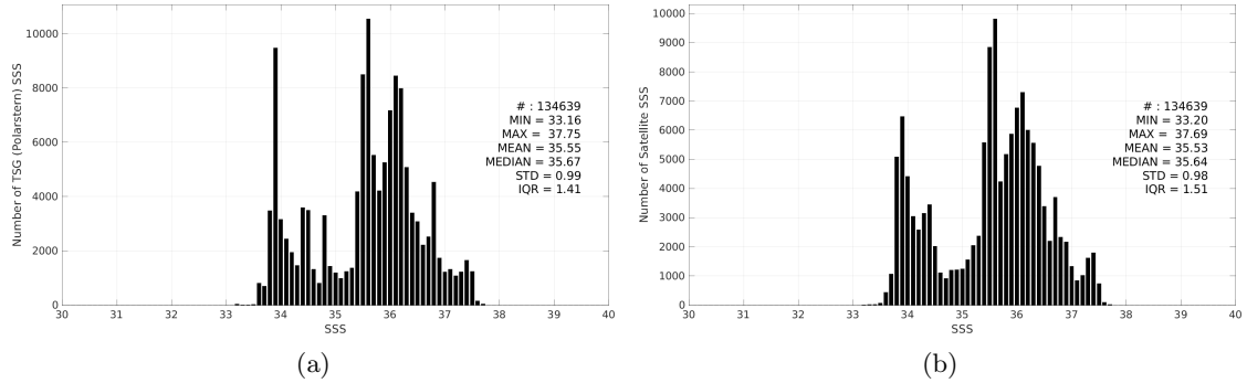
Figure 3: Histograms of SSS from TSG (Polarstern) (a) and CCI SSS L4 Merged-OI v4.41 - 30-day running (ESA) (b) considering all match-up pairs per bins of 0.1 over the South Atlantic Ocean Pi-MEP region and for the full satellite product period.
