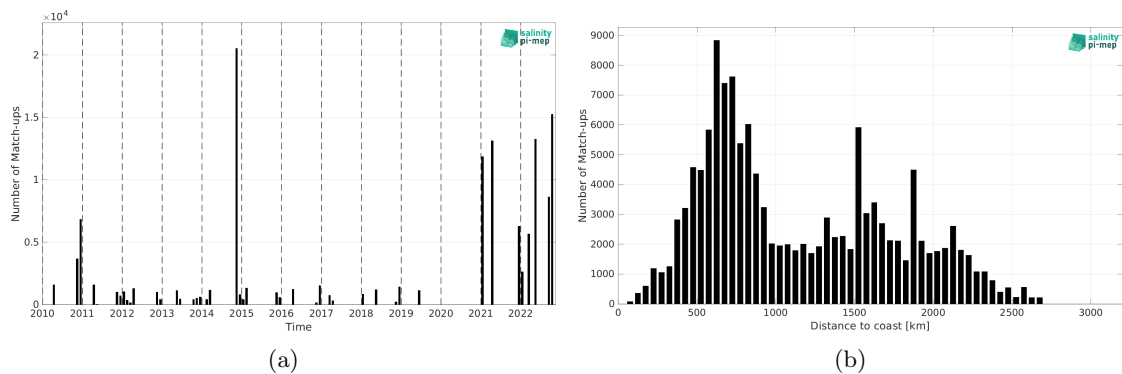
Figure 2: Number of match-ups between TSG (Polarstern) and CCI SSS L4 Merged-OI v4.41 - 30-day running (ESA) SSS as a function of time (a) and as function of the distance to coast (b) over the South Atlantic Ocean Pi-MEP region and for the full satellite product period.
