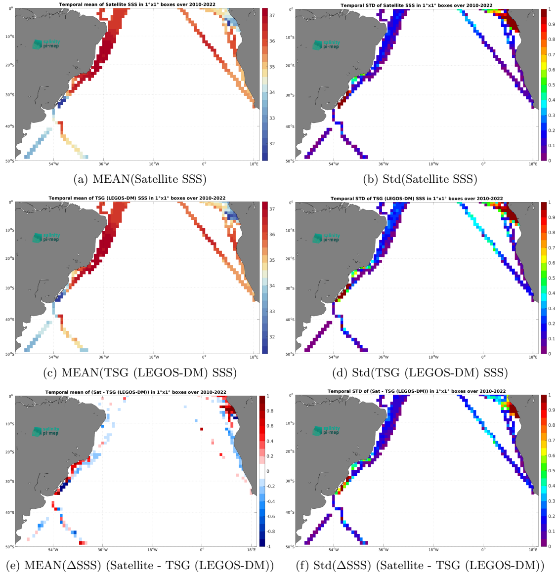
Figure 7: Temporal mean (left) and Std (right) of SSS from CCI SSS L4 Merged-OI v4.41 - 30-day running (ESA) (top), TSG (LEGOS-DM) (middle), and of \Delta SSS (Satellite - TSG (LEGOS-DM)). Only match-up pairs are used to generate these maps.
