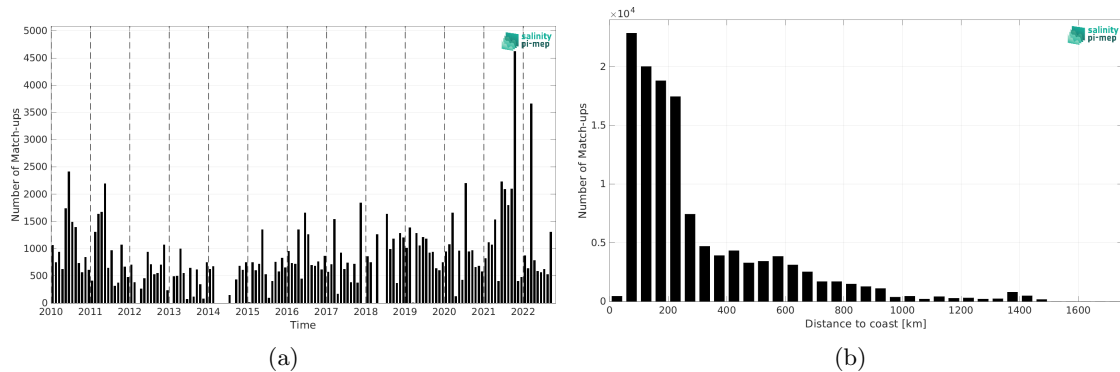
Figure 2: Number of match-ups between TSG (LEGOS-DM) and CCI SSS L4 Merged-OI v4.41 - 30-day running (ESA) SSS as a function of time (a) and as function of the distance to coast (b) over the South Atlantic Ocean Pi-MEP region and for the full satellite product period.
