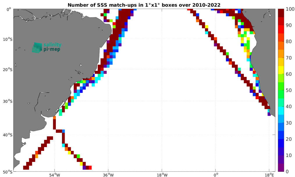
Figure 5: Number of SSS match-ups between TSG (LEGOS-DM) SSS and the CCI SSS L4 Merged-OI v4.41 - 30-day running (ESA) SSS product for the South Atlantic Ocean Pi-MEP region over 1^\circ \times 1^\circ boxes and for the full satellite product period.
