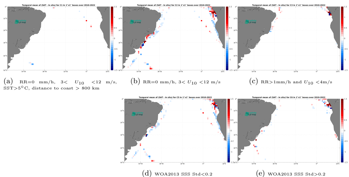
Figure 14: Temporal mean gridded over spatial boxes of size 1^\circ \times 1^\circ of \Delta\text{SSS} (CCI SSS L4 Merged-OI v4.41 - 30-day running (ESA) - TSG (LEGOS-DM)) for 5 different subdatasets corresponding to:RR=0 mm/h, 3 < U_{10} < 12 m/s, SST >5^\circ\text{C} , distance to coast > 800 km (a), RR=0 mm/h, 3 < U_{10} < 12 m/s (b), RR >1 mm/h and U_{10} < 4 m/s (c), WOA2013 SSS Std <0.2 (d), WOA2013 SSS Std >0.2 (e).
