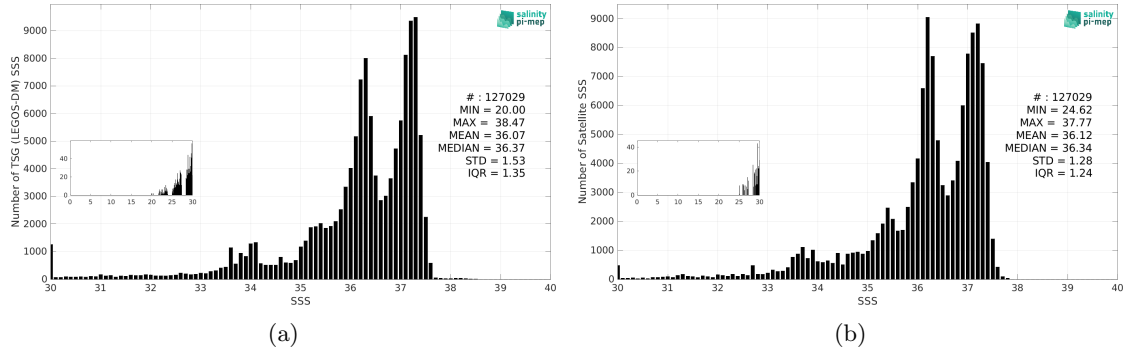
Figure 3: Histograms of SSS from TSG (LEGOS-DM) (a) and CCI SSS L4 Merged-OI v4.41 - 30-day running (ESA) (b) considering all match-up pairs per bins of 0.1 over the South Atlantic Ocean Pi-MEP region and for the full satellite product period.
