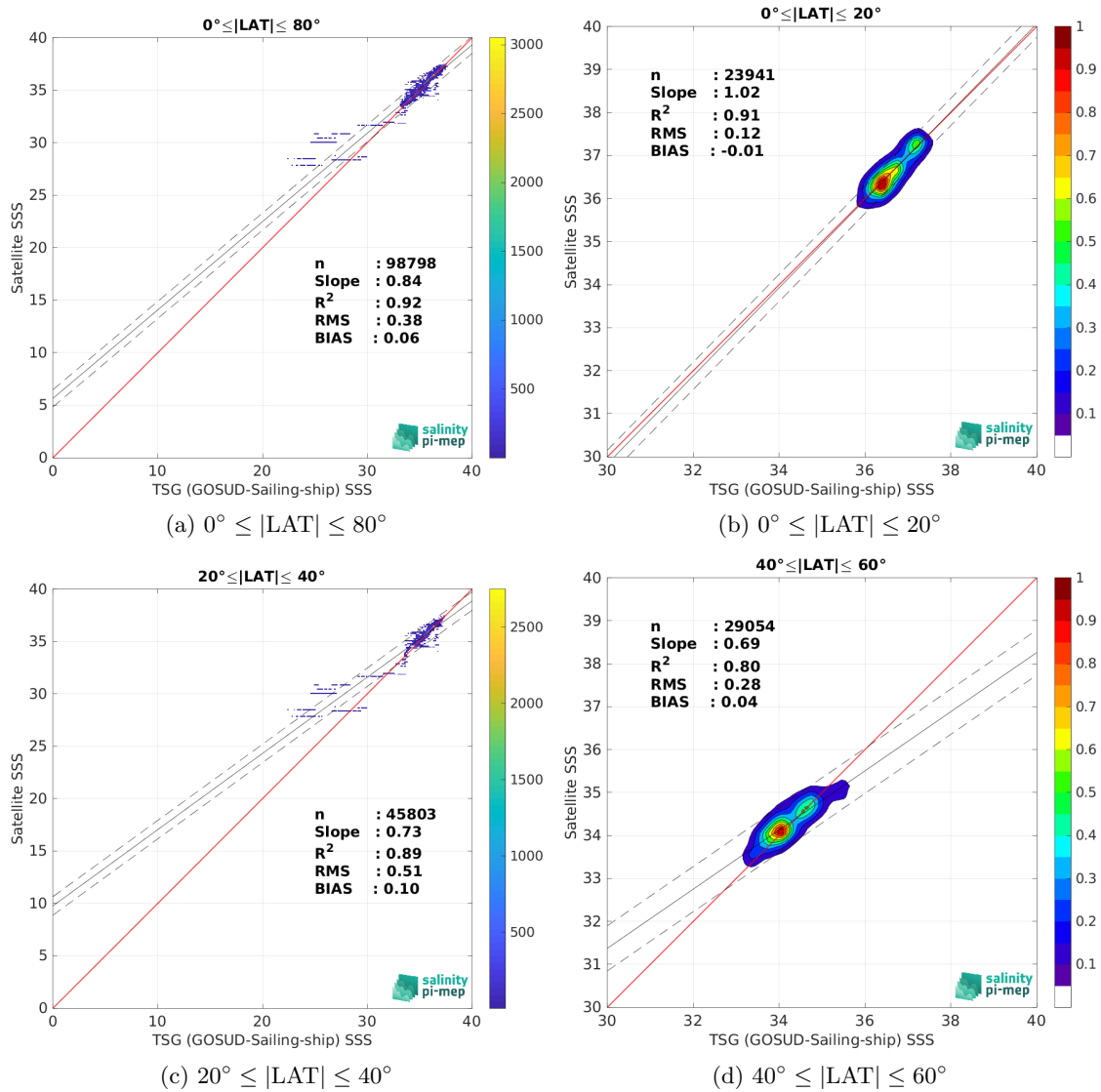
Figure 10: Contour maps of the concentration of CCI SSS L4 Merged-OI v4.41 - 30-day running (ESA) SSS (y-axis) versus TSG (GOSUD-Sailing-ship) SSS (x-axis) at match-up pairs for different latitude bands. For each plot, the red line shows x=y . The black thin and dashed lines indicate a linear fit through the data cloud and the \pm 95\% confidence levels, respectively. The number match-up pairs n , the slope and R^2 coefficient of the linear fit, the root mean square (RMS) and the mean bias between satellite and in situ data are indicated for each latitude band in each plots.
