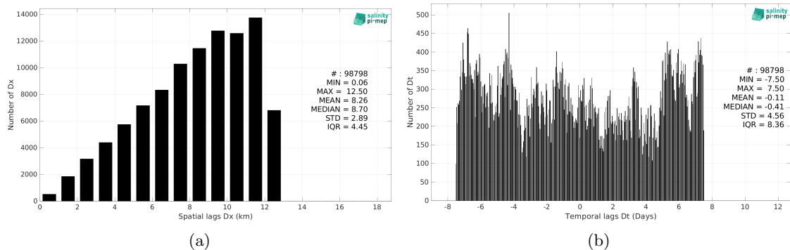
Figure 6: Histograms of the spatial (a) and temporal (b) lags between the location/time of the TSG (GOSUD-Sailing-ship) measurement and the date of the corresponding CCI SSS L4 Merged-OI v4.41 - 30-day running (ESA) SSS pixel.
