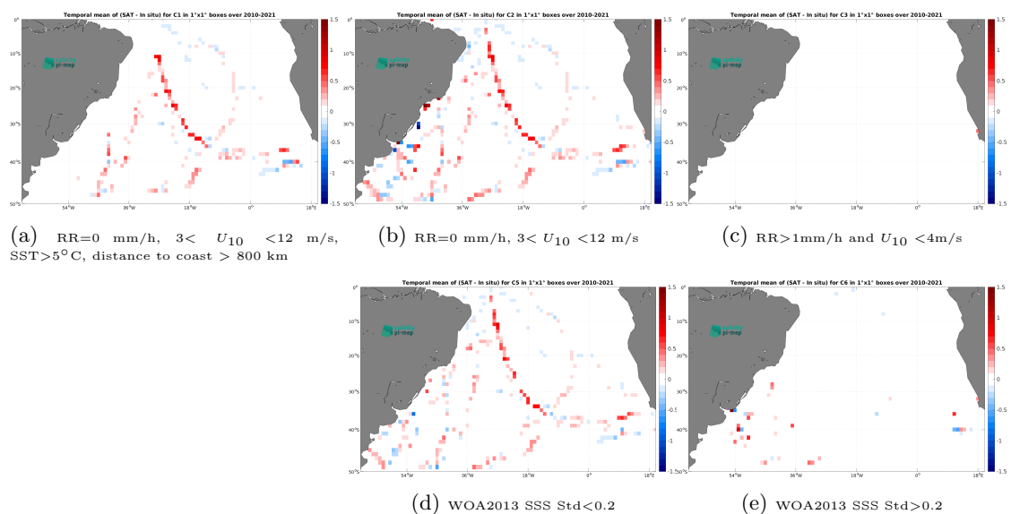
Figure 14: Temporal mean gridded over spatial boxes of size 1^\circ \times 1^\circ of \Delta\text{SSS} (CCI SSS L4 Merged-OI v4.41 - 30-day running (ESA) - TSG (GOSUD-Sailing-ship)) for 5 different subdatasets corresponding to:RR=0 mm/h, 3 < U_{10} < 12 m/s, SST >5^\circ\text{C} , distance to coast > 800 km (a), RR=0 mm/h, 3 < U_{10} < 12 m/s (b), RR >1 mm/h and U_{10} < 4 m/s (c), WOA2013 SSS Std <0.2 (d), WOA2013 SSS Std >0.2 (e).
