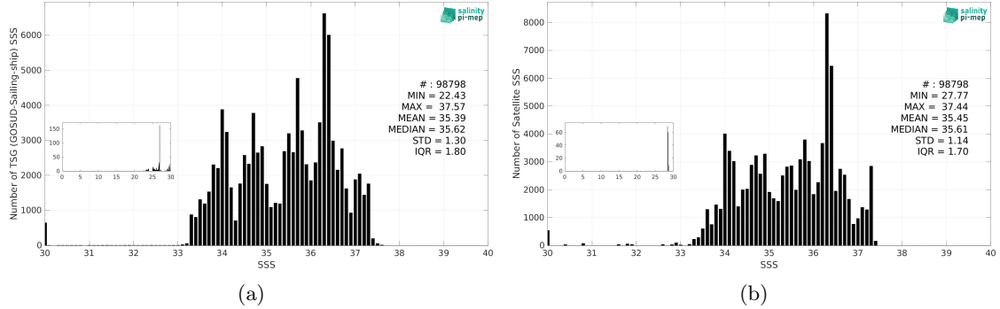
Figure 3: Histograms of SSS from TSG (GOSUD-Sailing-ship) (a) and CCI SSS L4 Merged-OI v4.41 - 30-day running (ESA) (b) considering all match-up pairs per bins of 0.1 over the South Atlantic Ocean Pi-MEP region and for the full satellite product period.
