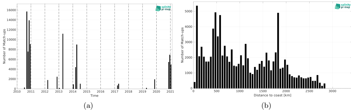
Figure 2: Number of match-ups between TSG (GOSUD-Sailing-ship) and CCI SSS L4 Merged-OI v4.41 - 30-day running (ESA) SSS as a function of time (a) and as function of the distance to coast (b) over the South Atlantic Ocean Pi-MEP region and for the full satellite product period.
