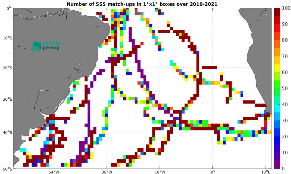
Figure 5: Number of SSS match-ups between TSG (GOSUD-Sailing-ship) SSS and the CCI SSS L4 Merged-OI v4.41 - 30-day running (ESA) SSS product for the South Atlantic Ocean Pi-MEP region over 1^\circ \times 1^\circ boxes and for the full satellite product period.
