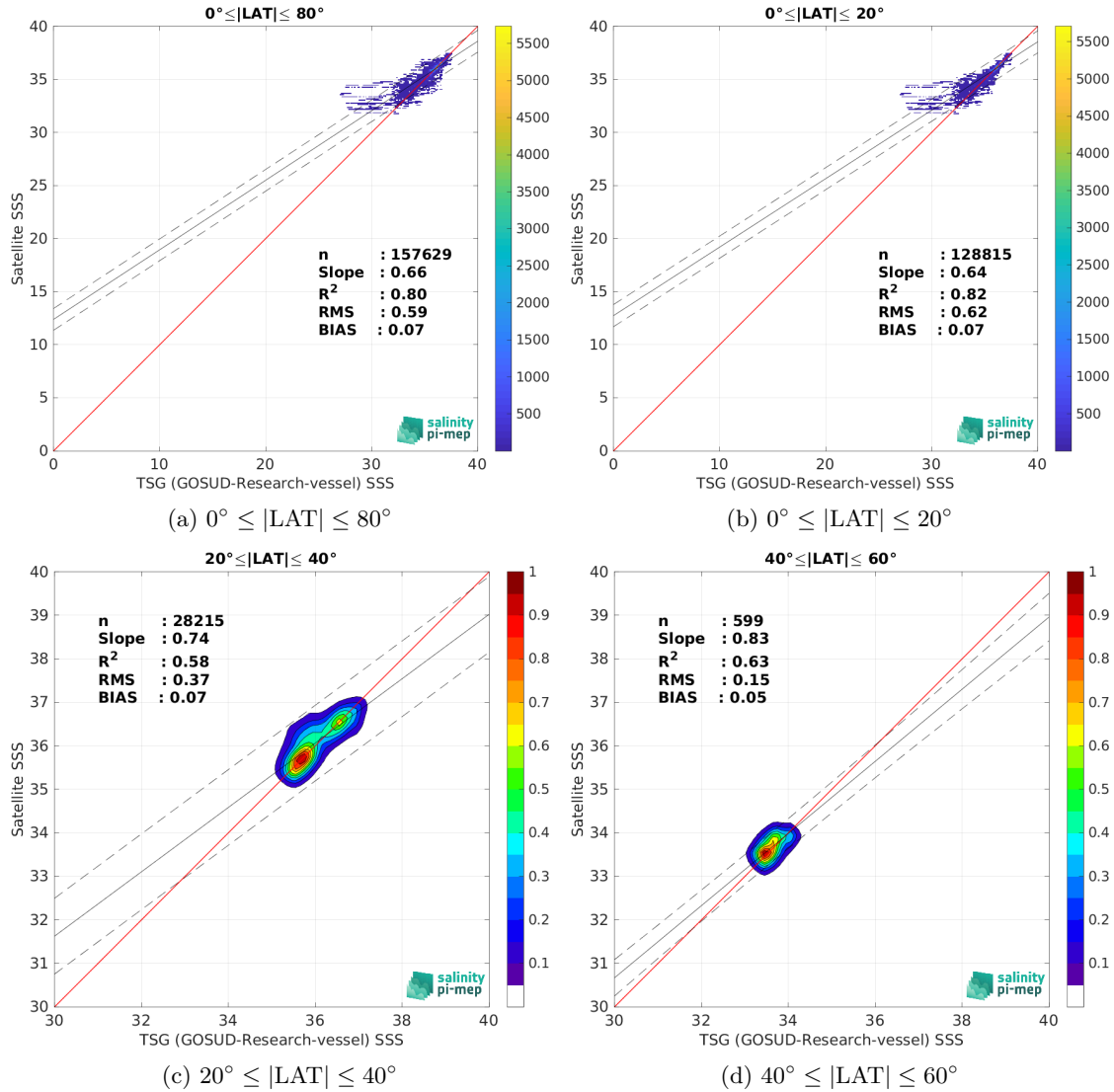
Figure 10: Contour maps of the concentration of CCI SSS L4 Merged-OI v4.41 - 30-day running (ESA) SSS (y-axis) versus TSG (GOSUD-Research-vessel) SSS (x-axis) at match-up pairs for different latitude bands. For each plot, the red line shows x=y . The black thin and dashed lines indicate a linear fit through the data cloud and the \pm 95\% confidence levels, respectively. The number match-up pairs n , the slope and R^2 coefficient of the linear fit, the root mean square (RMS) and the mean bias between satellite and in situ data are indicated for each latitude band in each plots.
