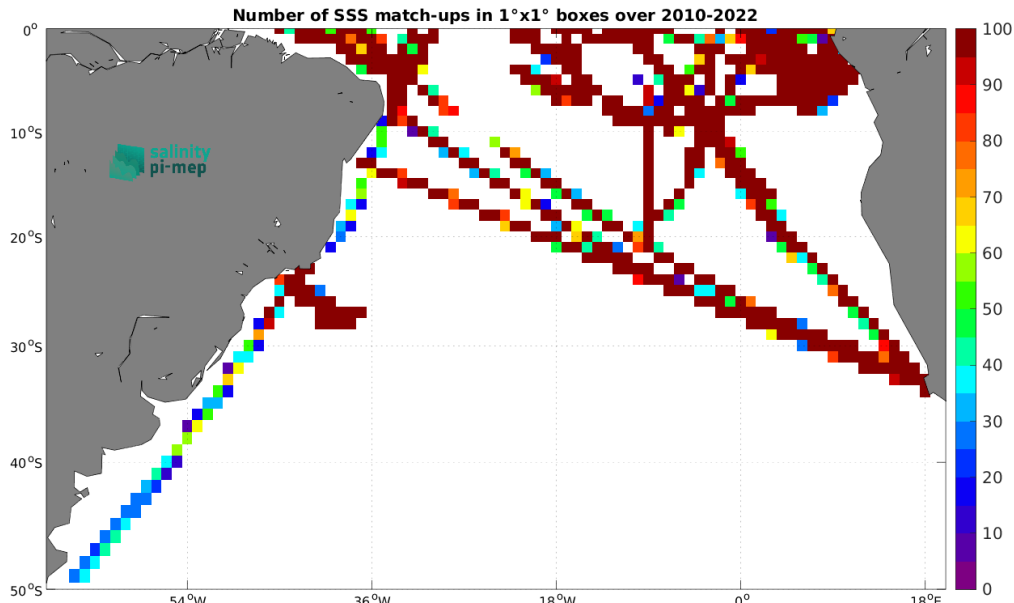
Figure 5: Number of SSS match-ups between TSG (GOSUD-Research-vessel) SSS and the CCI SSS L4 Merged-OI v4.41 - 30-day running (ESA) SSS product for the South Atlantic Ocean Pi-MEP region over 1^\circ \times 1^\circ boxes and for the full satellite product period.
