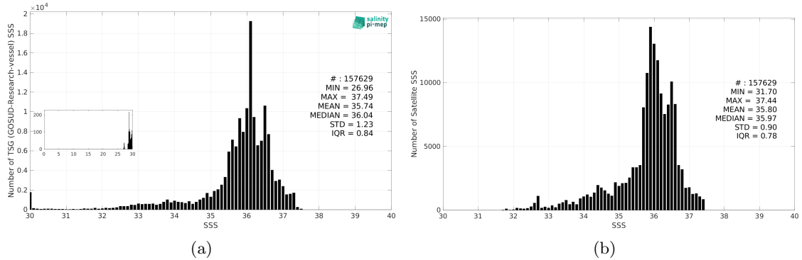
Figure 3: Histograms of SSS from TSG (GOSUD-Research-vessel) (a) and CCI SSS L4 Merged-OI v4.41 - 30-day running (ESA) (b) considering all match-up pairs per bins of 0.1 over the South Atlantic Ocean Pi-MEP region and for the full satellite product period.
