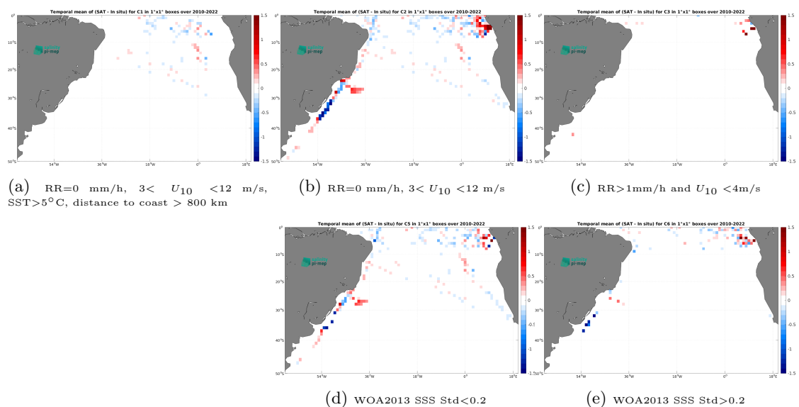
Figure 14: Temporal mean gridded over spatial boxes of size 1^\circ \times 1^\circ of \Delta\text{SSS} (CCI SSS L4 Merged-OI v4.41 - 30-day running (ESA) - TSG (GOSUD-Research-vessel)) for 5 different subdatasets corresponding to:RR=0 mm/h, 3 < U_{10} < 12 m/s, SST >5^\circ\text{C} , distance to coast > 800 km (a), RR=0 mm/h, 3 < U_{10} < 12 m/s (b), RR >1 mm/h and U_{10} < 4 m/s (c), WOA2013 SSS Std <0.2 (d), WOA2013 SSS Std >0.2 (e).
