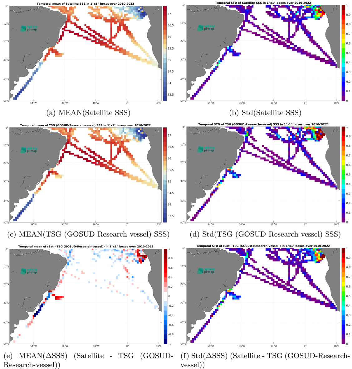
Figure 7: Temporal mean (left) and Std (right) of SSS from CCI SSS L4 Merged-OI v4.41 - 30-day running (ESA) (top), TSG (GOSUD-Research-vessel) (middle), and of \Delta SSS (Satellite - TSG (GOSUD-Research-vessel)). Only match-up pairs are used to generate these maps.
