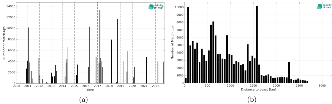
Figure 2: Number of match-ups between TSG (GOSUD-Research-vessel) and CCI SSS L4 Merged-OI v4.41 - 30-day running (ESA) SSS as a function of time (a) and as function of the distance to coast (b) over the South Atlantic Ocean Pi-MEP region and for the full satellite product period.
