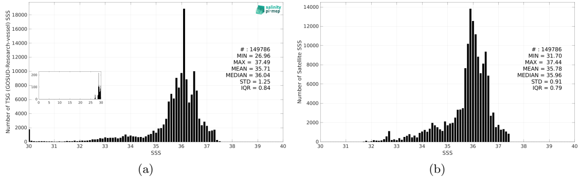
Figure 3: Histograms of SSS from TSG (GOSUD-Research-vessel) (a) and CCI SSS L4 Merged-OI v4.41 - 30-day running (ESA) (b) considering all match-up pairs per bins of 0.1 over the South Atlantic Ocean Pi-MEP region and for the full satellite product period.
