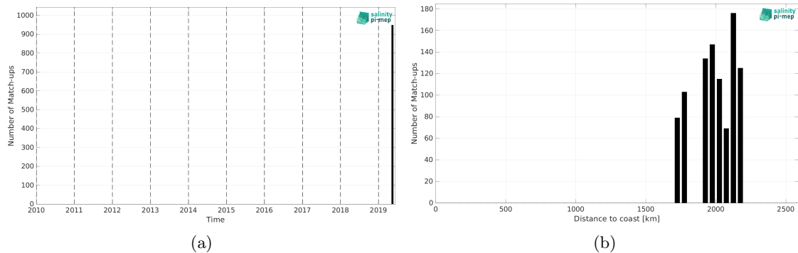
Figure 2: Number of match-ups between Saildrone and CCI SSS L4 Merged-OI v4.41 - 30-day running (ESA) SSS as a function of time (a) and as function of the distance to coast (b) over the South Atlantic Ocean Pi-MEP region and for the full satellite product period.
