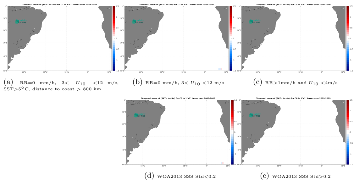
Figure 14: Temporal mean gridded over spatial boxes of size 1^\circ \times 1^\circ of \Delta\text{SSS} (CCI SSS L4 Merged-OI v4.41 - 30-day running (ESA) - Saildrone) for 5 different subdatasets corresponding to:RR=0 mm/h, 3 < U_{10} < 12 m/s, SST >5^\circ\text{C} , distance to coast > 800 km (a), RR=0 mm/h, 3 < U_{10} < 12 m/s (b), RR >1 mm/h and U_{10} < 4 m/s (c), WOA2013 SSS Std <0.2 (d), WOA2013 SSS Std >0.2 (e).
