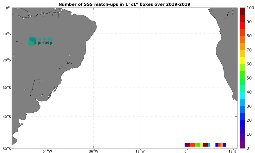
Figure 5: Number of SSS match-ups between Saildrone SSS and the CCI SSS L4 Merged-OI v4.41 - 30-day running (ESA) SSS product for the South Atlantic Ocean Pi-MEP region over 1^\circ \times 1^\circ boxes and for the full satellite product period.
