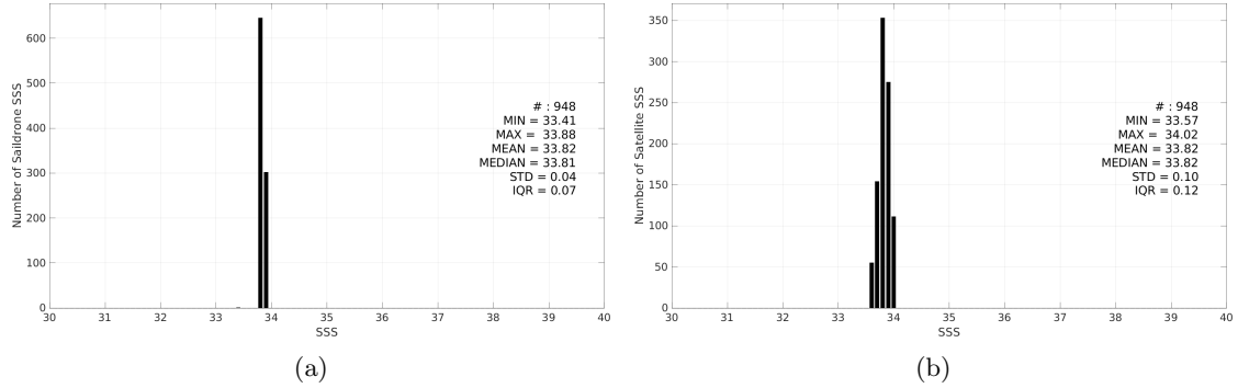
Figure 3: Histograms of SSS from Saildrone (a) and CCI SSS L4 Merged-OI v4.41 - 30-day running (ESA) (b) considering all match-up pairs per bins of 0.1 over the South Atlantic Ocean Pi-MEP region and for the full satellite product period.
