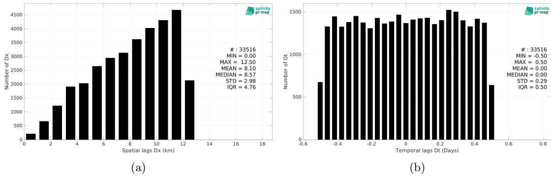
Figure 5: Histograms of the spatial (a) and temporal (b) lags between the location/time of the TSG (SAMOS) measurement and the date of the corresponding CCI SSS L4 Merged-OI v4.4 - 7-day running (ESA) SSS pixel.
