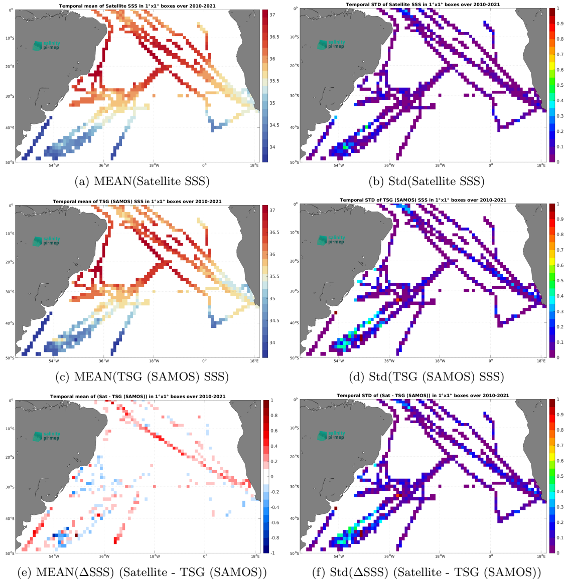
Figure 6: Temporal mean (left) and Std (right) of SSS from CCI SSS L4 Merged-OI v4.4 - 7-day running (ESA) (top), TSG (SAMOS) (middle), and of \Delta SSS (Satellite - TSG (SAMOS)). Only match-up pairs are used to generate these maps.
