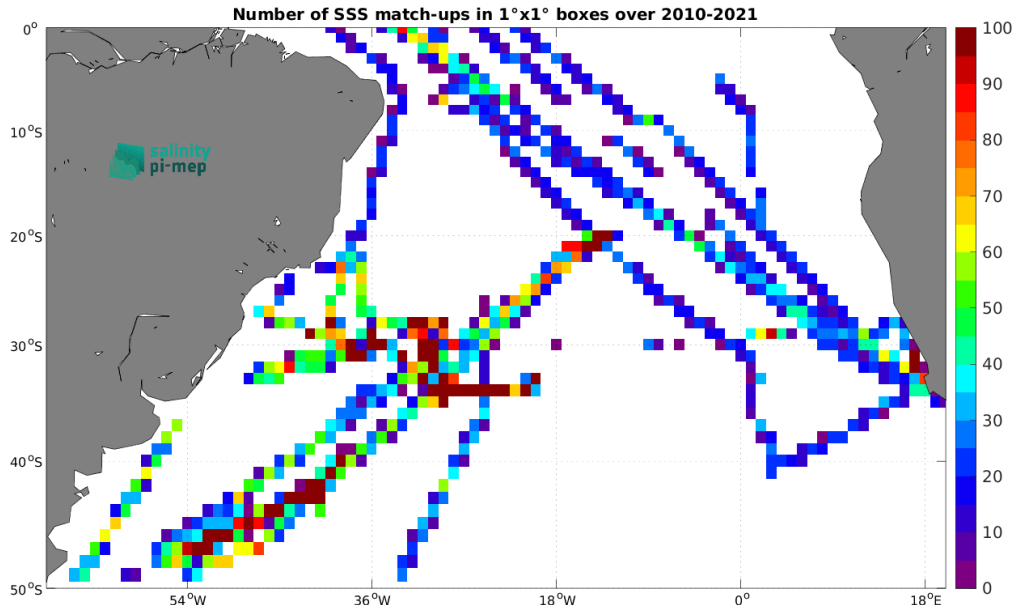
Figure 4: Number of SSS match-ups between TSG (SAMOS) SSS and the CCI SSS L4 Merged-OI v4.4 - 7-day running (ESA) SSS product for the South Atlantic Ocean Pi-MEP region over 1^\circ \times 1^\circ boxes and for the full satellite product period.
