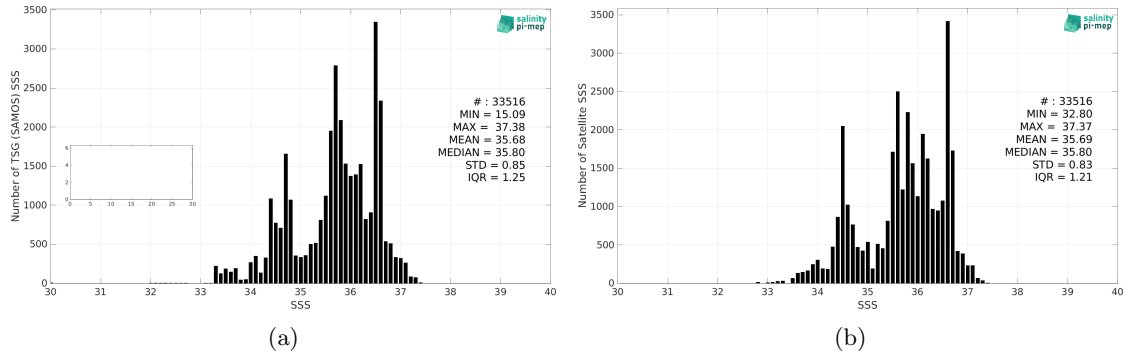
Figure 2: Histograms of SSS from TSG (SAMOS) (a) and CCI SSS L4 Merged-OI v4.4 - 7-day running (ESA) (b) considering all match-up pairs per bins of 0.1 over the South Atlantic Ocean Pi-MEP region and for the full satellite product period.
