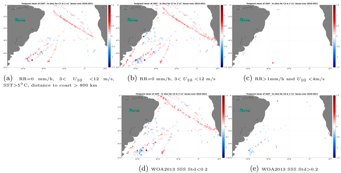
Figure 12: Temporal mean gridded over spatial boxes of size 1^\circ \times 1^\circ of \Delta\text{SSS} (CCI SSS L4 Merged-OI v4.4 - 7-day running (ESA) - TSG (SAMOS)) for 5 different subdatasets corresponding to:RR=0 mm/h, 3 < U_{10} < 12 m/s, SST >5^\circ\text{C} , distance to coast > 800 km (a), RR=0 mm/h, 3 < U_{10} < 12 m/s (b), RR >1 mm/h and U_{10} < 4 m/s (c), WOA2013 SSS Std <0.2 (d), WOA2013 SSS Std >0.2 (e).
