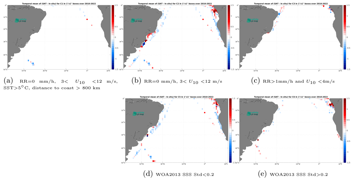
Figure 12: Temporal mean gridded over spatial boxes of size 1^\circ \times 1^\circ of \Delta\text{SSS} (CCI SSS L4 Merged-OI v4.4 - 7-day running (ESA) - TSG (LEGOS-DM)) for 5 different subdatasets corresponding to:RR=0 mm/h, 3 < U_{10} < 12 m/s, SST >5^\circ\text{C} , distance to coast > 800 km (a), RR=0 mm/h, 3 < U_{10} < 12 m/s (b), RR >1 mm/h and U_{10} < 4 m/s (c), WOA2013 SSS Std <0.2 (d), WOA2013 SSS Std >0.2 (e).
