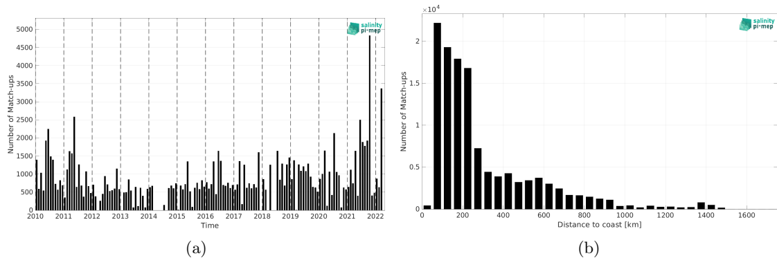
Figure 1: Number of match-ups between TSG (LEGOS-DM) and CCI SSS L4 Merged-OI v4.4 - 7-day running (ESA) SSS as a function of time (a) and as function of the distance to coast (b) over the South Atlantic Ocean Pi-MEP region and for the full satellite product period.
