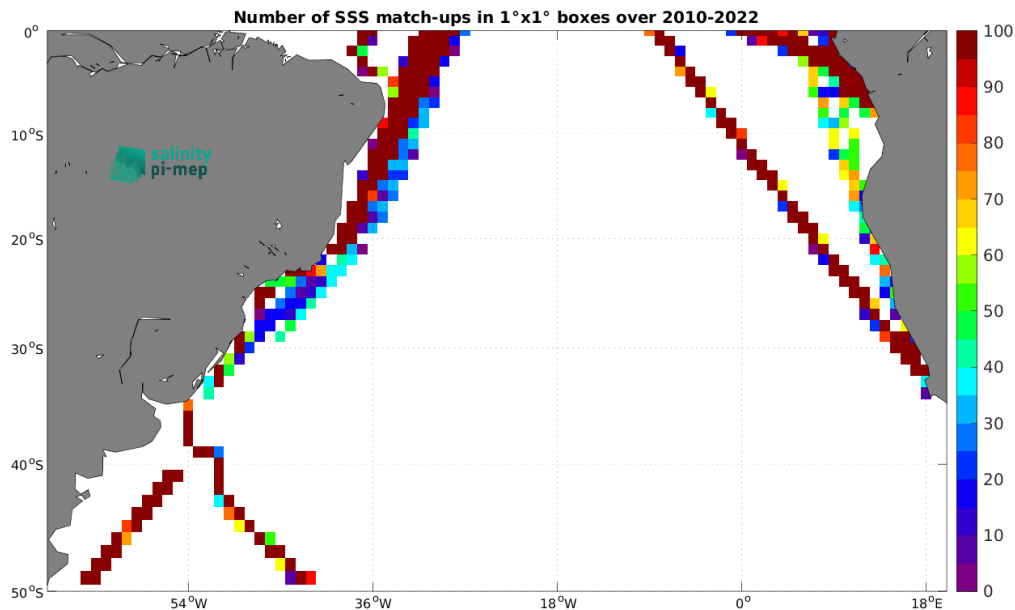
Figure 4: Number of SSS match-ups between TSG (LEGOS-DM) SSS and the CCI SSS L4 Merged-OI v4.4 - 7-day running (ESA) SSS product for the South Atlantic Ocean Pi-MEP region over 1^\circ \times 1^\circ boxes and for the full satellite product period.
