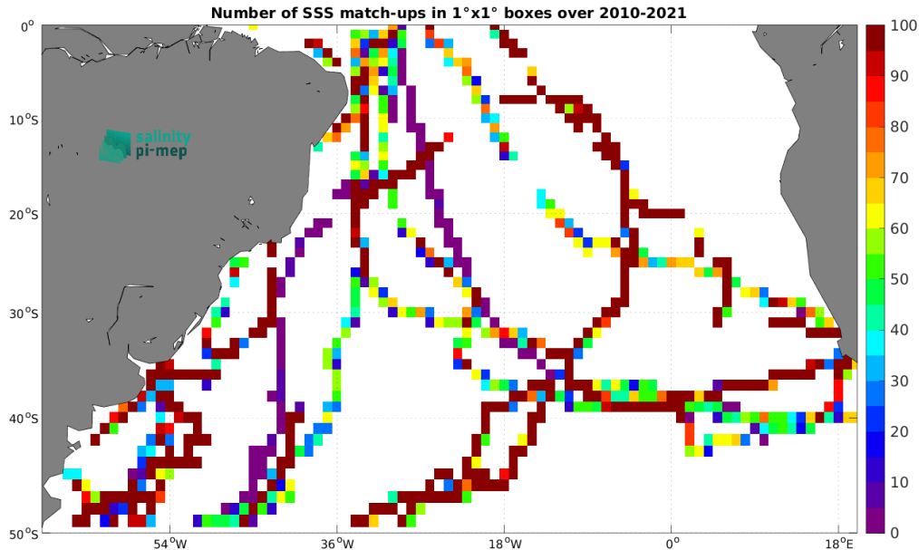
Figure 4: Number of SSS match-ups between TSG (GOSUD-Sailing-ship) SSS and the CCI SSS L4 Merged-OI v4.4 - 7-day running (ESA) SSS product for the South Atlantic Ocean Pi-MEP region over 1^\circ \times 1^\circ boxes and for the full satellite product period.
