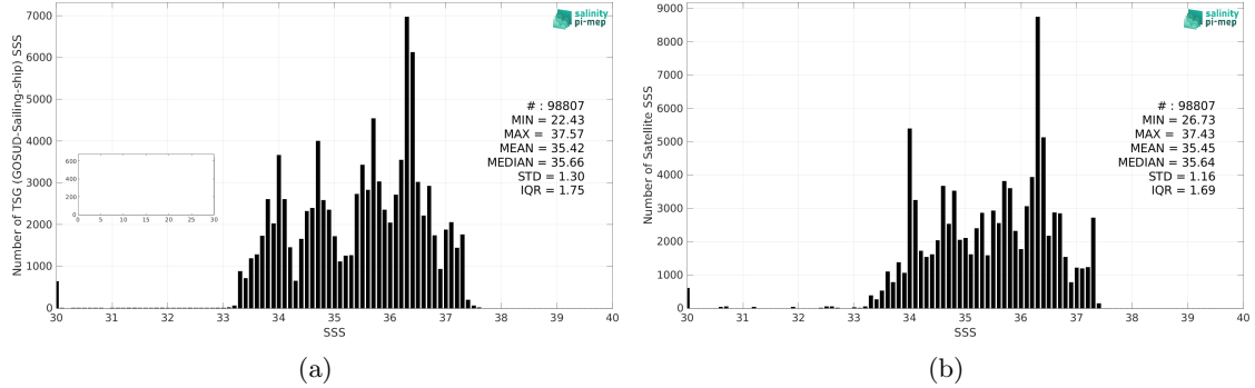
Figure 2: Histograms of SSS from TSG (GOSUD-Sailing-ship) (a) and CCI SSS L4 Merged-OI v4.4 - 7-day running (ESA) (b) considering all match-up pairs per bins of 0.1 over the South Atlantic Ocean Pi-MEP region and for the full satellite product period.
