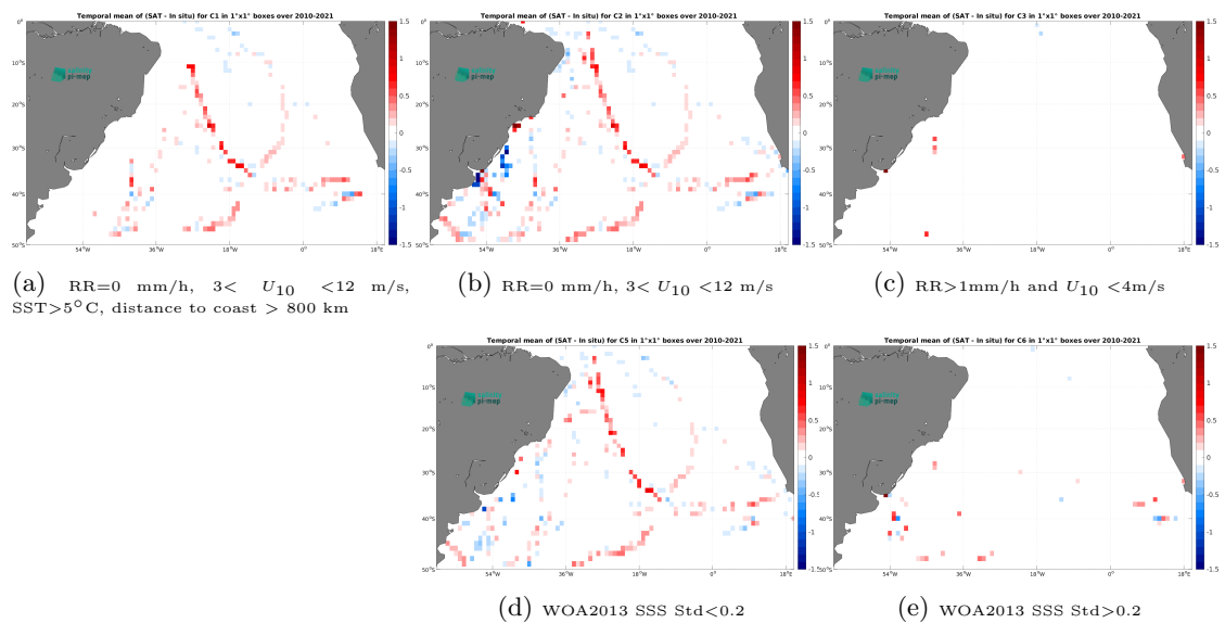
Figure 12: Temporal mean gridded over spatial boxes of size 1^\circ \times 1^\circ of \Delta SSS (CCI SSS L4 Merged-OI v4.4 - 7-day running (ESA) - TSG (GOSUD-Sailing-ship)) for 5 different subdatasets corresponding to:RR=0 mm/h, 3 < U_{10} < 12 m/s, SST >5^\circ\text{C} , distance to coast > 800 km (a), RR=0 mm/h, 3 < U_{10} < 12 m/s (b), RR >1 mm/h and U_{10} < 4 m/s (c), WOA2013 SSS Std <0.2 (d), WOA2013 SSS Std >0.2 (e).
