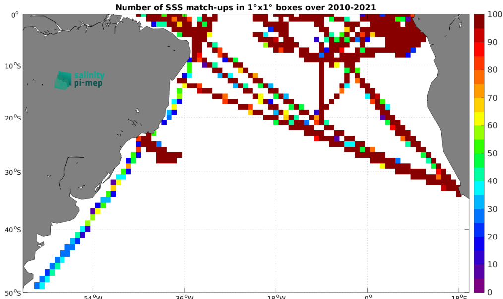
Figure 4: Number of SSS match-ups between TSG (GOSUD-Research-vessel) SSS and the CCI SSS L4 Merged-OI v4.4 - 7-day running (ESA) SSS product for the South Atlantic Ocean Pi-MEP region over 1^\circ \times 1^\circ boxes and for the full satellite product period.
