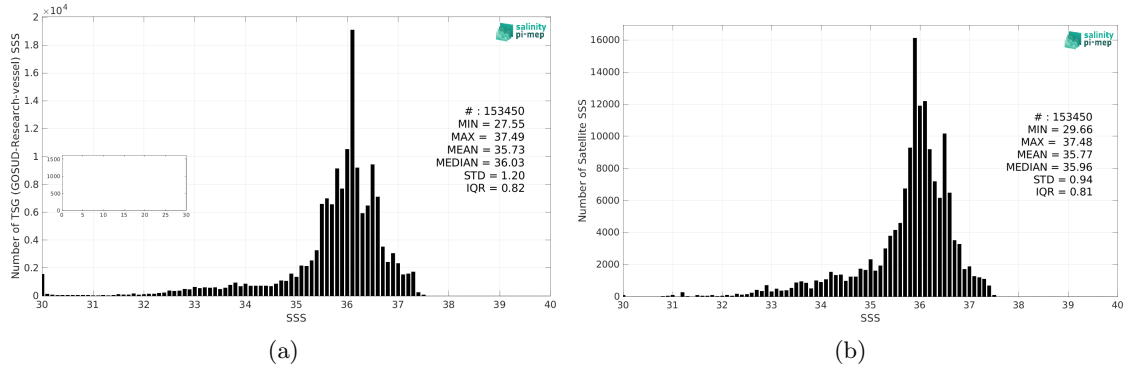
Figure 2: Histograms of SSS from TSG (GOSUD-Research-vessel) (a) and CCI SSS L4 Merged-OI v4.4 - 7-day running (ESA) (b) considering all match-up pairs per bins of 0.1 over the South Atlantic Ocean Pi-MEP region and for the full satellite product period.
