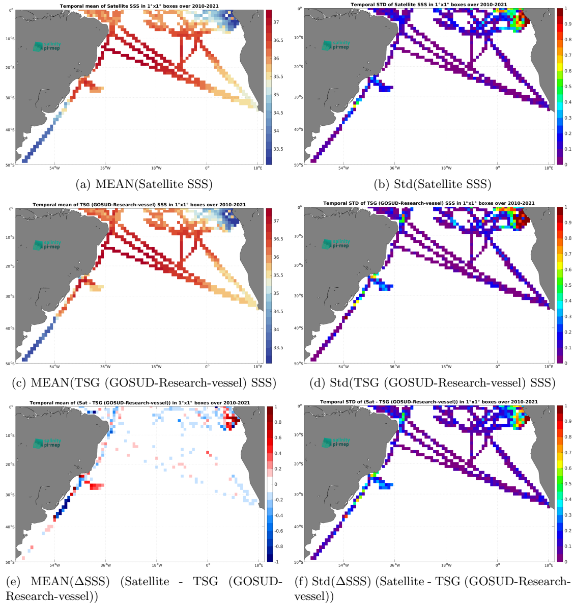
Figure 6: Temporal mean (left) and Std (right) of SSS from CCI SSS L4 Merged-OI v4.4 - 7-day running (ESA) (top), TSG (GOSUD-Research-vessel) (middle), and of \Delta SSS (Satellite - TSG (GOSUD-Research-vessel)). Only match-up pairs are used to generate these maps.
