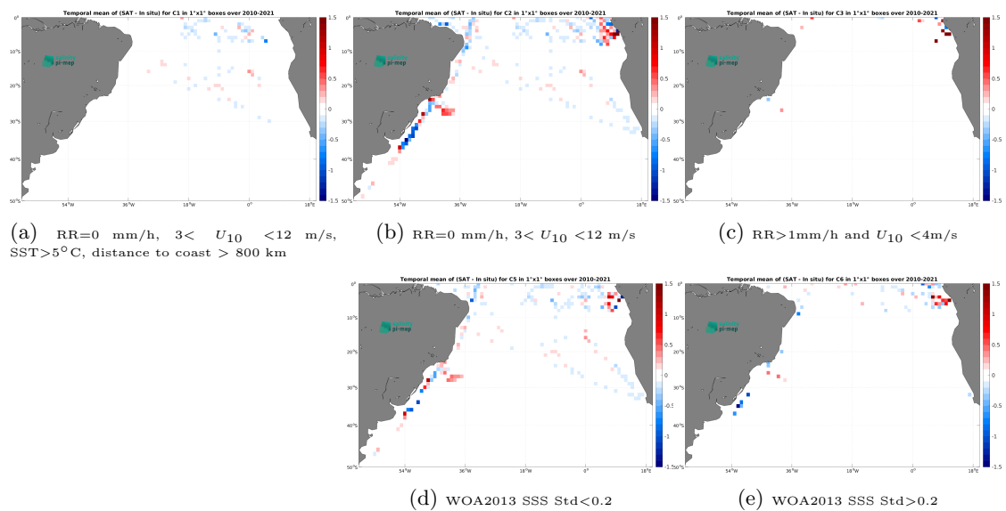
Figure 12: Temporal mean gridded over spatial boxes of size 1^\circ \times 1^\circ of \Delta\text{SSS} (CCI SSS L4 Merged-OI v4.4 - 7-day running (ESA) - TSG (GOSUD-Research-vessel)) for 5 different subdatasets corresponding to:RR=0 mm/h, 3 < U_{10} < 12 m/s, SST >5^\circ\text{C} , distance to coast > 800 km (a), RR=0 mm/h, 3 < U_{10} < 12 m/s (b), RR >1 mm/h and U_{10} < 4 m/s (c), WOA2013 SSS Std <0.2 (d), WOA2013 SSS Std >0.2 (e).
