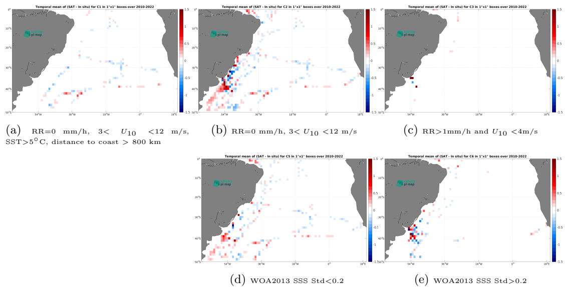
Figure 12: Temporal mean gridded over spatial boxes of size 1^\circ \times 1^\circ of \Delta\text{SSS} (CCI SSS L4 Merged-OI v4.4 - 7-day running (ESA) - TSG (CSIC-UTM)) for 5 different subdatasets corresponding to:RR=0 mm/h, 3 < U_{10} < 12 m/s, SST >5^\circ\text{C} , distance to coast > 800 km (a), RR=0 mm/h, 3 < U_{10} < 12 m/s (b), RR >1 mm/h and U_{10} < 4 m/s (c), WOA2013 SSS Std <0.2 (d), WOA2013 SSS Std >0.2 (e).
