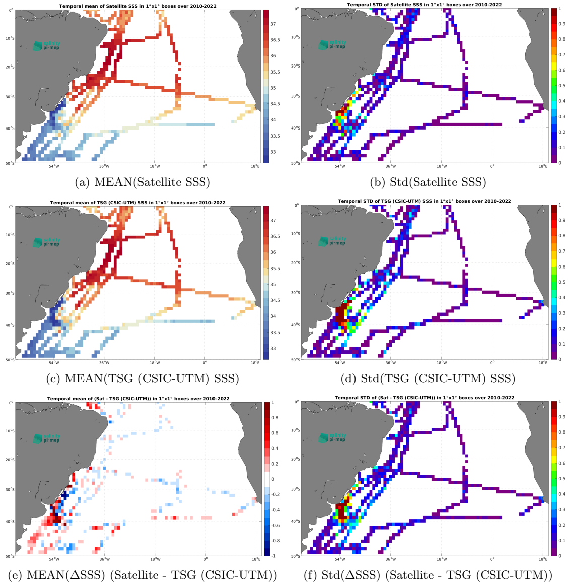
Figure 6: Temporal mean (left) and Std (right) of SSS from CCI SSS L4 Merged-OI v4.4 - 7-day running (ESA) (top), TSG (CSIC-UTM) ( in situ ) dataset (middle), and of \Delta SSS (Satellite - TSG (CSIC-UTM)). Only match-up pairs are used to generate these maps.
