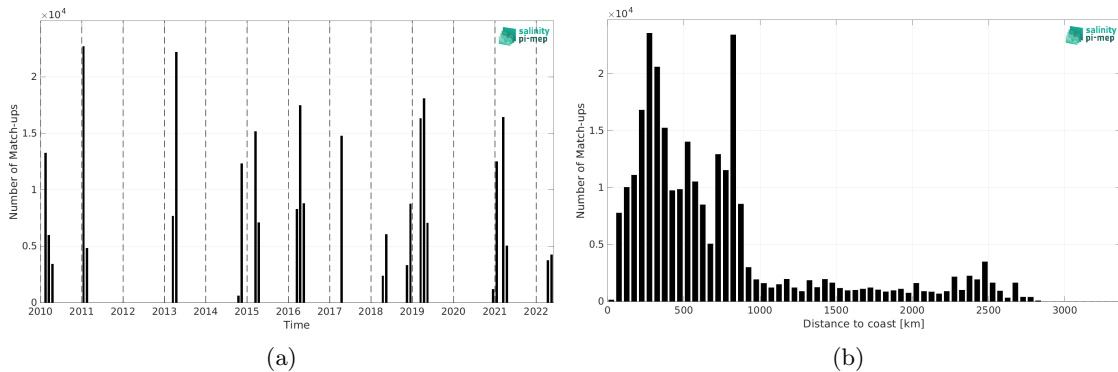
Figure 1: Number of match-ups between TSG (CSIC-UTM) and CCI SSS L4 Merged-OI v4.4 - 7-day running (ESA) SSS as a function of time (a) and as function of the distance to coast (b) over the South Atlantic Ocean Pi-MEP region and for the full satellite product period.
