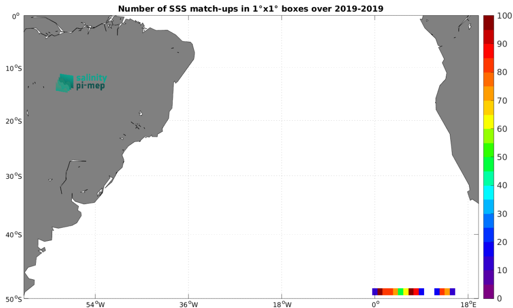
Figure 4: Number of SSS match-ups between Saildrone SSS and the CCI SSS L4 Merged-OI v4.4 - 7-day running (ESA) SSS product for the South Atlantic Ocean Pi-MEP region over 1^\circ \times 1^\circ boxes and for the full satellite product period.
