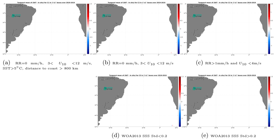
Figure 12: Temporal mean gridded over spatial boxes of size 1^{\circ}\times 1^{\circ} of \Delta\text{SSS} (CCI SSS L4 Merged-OI v4.4 - 7-day running (ESA) - Saildrone) for 5 different subdatasets corresponding to:RR=0 mm/h, 3 < U_{10} < 12 m/s, SST >5^{\circ}\text{C} , distance to coast > 800 km (a), RR=0 mm/h, 3 < U_{10} < 12 m/s (b), RR >1 mm/h and U_{10} < 4 m/s (c), WOA2013 SSS Std <0.2 (d), WOA2013 SSS Std >0.2 (e).
