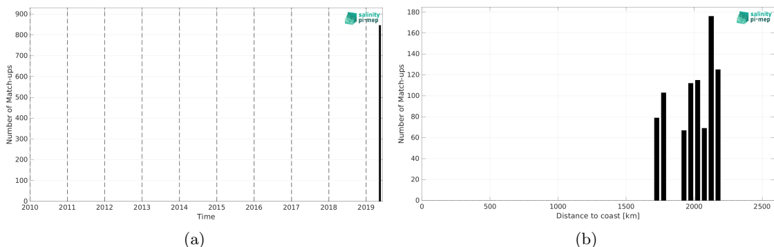
Figure 1: Number of match-ups between Saildrone and CCI SSS L4 Merged-OI v4.4 - 7-day running (ESA) SSS as a function of time (a) and as function of the distance to coast (b) over the South Atlantic Ocean Pi-MEP region and for the full satellite product period.
