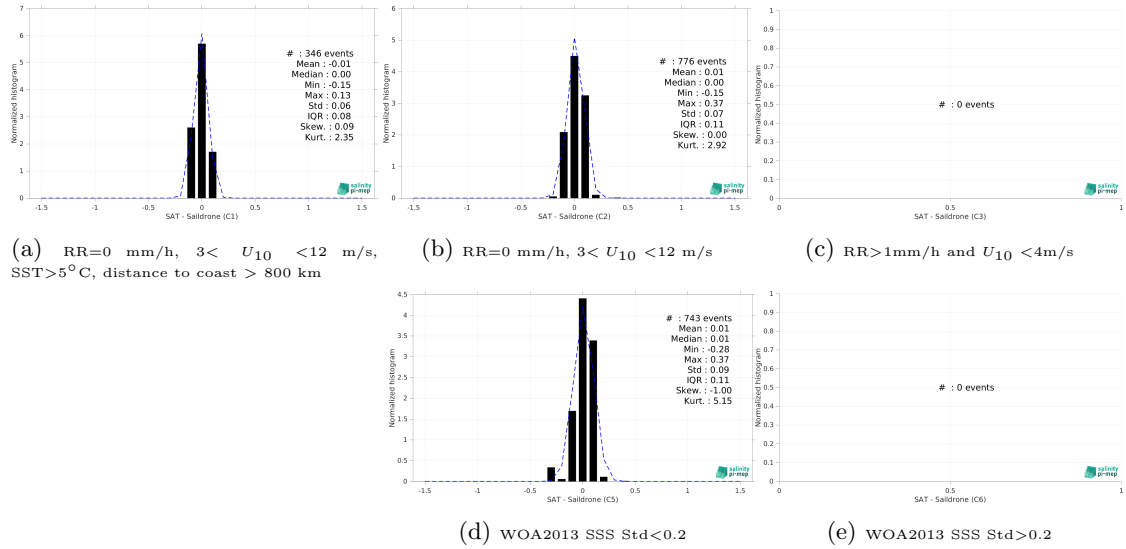
Figure 13: Normalized histogram of \Delta SSS (CCI SSS L4 Merged-OI v4.4 - 7-day running (ESA) - Saldrone) for 5 different subdatasets corresponding to: RR=0 mm/h, 3 < U_{10} < 12 m/s, SST > 5°C, distance to coast > 800 km (a), RR=0 mm/h, 3 < U_{10} < 12 m/s (b), RR > 1mm/h and U_{10} < 4 m/s (c), WOA2013 SSS Std < 0.2 (d), WOA2013 SSS Std > 0.2 (e).
