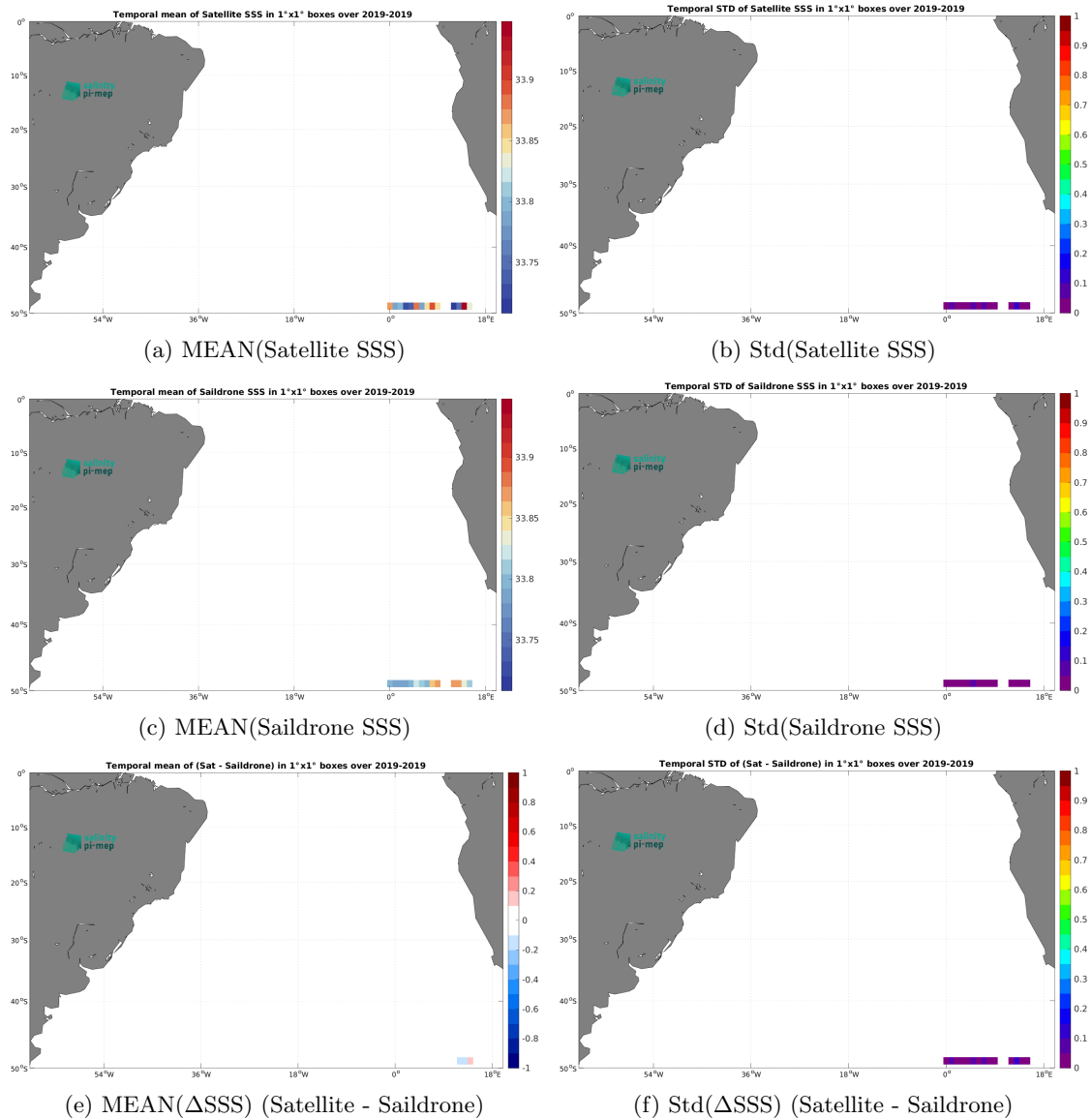
Figure 6: Temporal mean (left) and Std (right) of SSS from CCI SSS L4 Merged-OI v4.4 - 7-day running (ESA) (top), Saildrone (middle), and of \Delta SSS (Satellite - Saildrone). Only match-up pairs are used to generate these maps.
