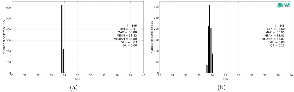
Figure 2: Histograms of SSS from Saildrone (a) and CCI SSS L4 Merged-OI v4.4 - 7-day running (ESA) (b) considering all match-up pairs per bins of 0.1 over the South Atlantic Ocean Pi-MEP region and for the full satellite product period.
