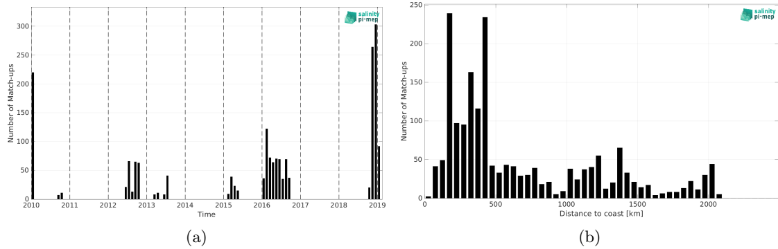
Figure 1: Number of match-ups between Marine mammals and CCI SSS L4 Merged-OI v4.4 - 7-day running (ESA) SSS as a function of time (a) and as function of the distance to coast (b) over the South Atlantic Ocean Pi-MEP region and for the full satellite product period.
