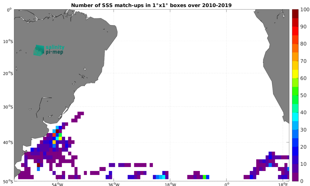
Figure 4: Number of SSS match-ups between Marine mammals SSS and the CCI SSS L4 Merged-OI v4.4 - 7-day running (ESA) SSS product for the South Atlantic Ocean Pi-MEP region over 1^\circ \times 1^\circ boxes and for the full satellite product period.
