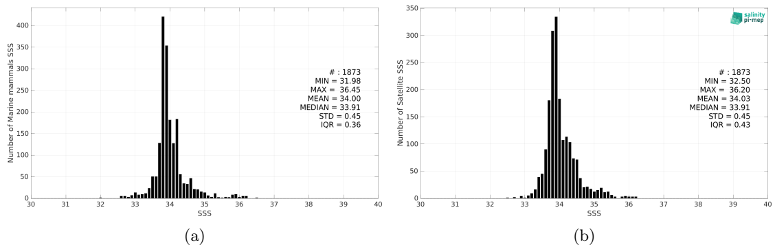
Figure 2: Histograms of SSS from Marine mammals (a) and CCI SSS L4 Merged-OI v4.4 - 7-day running (ESA) (b) considering all match-up pairs per bins of 0.1 over the South Atlantic Ocean Pi-MEP region and for the full satellite product period.
