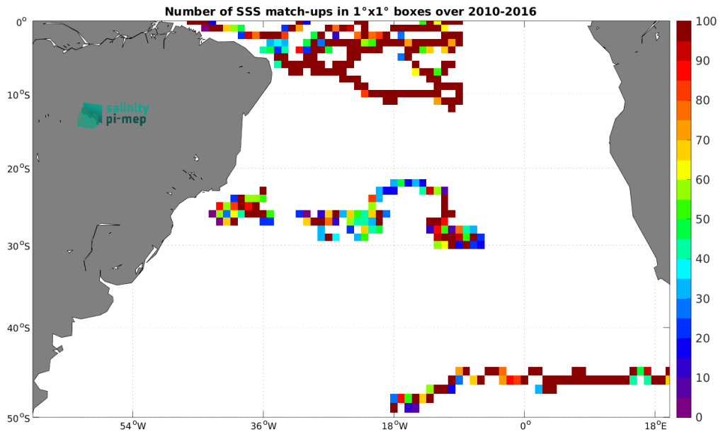
Figure 3: Number of SSS match-ups between Surface drifters SSS and the CCI SSS L4 Merged-OI v4.4 - 7-day running (ESA) SSS product for the South Atlantic Ocean Pi-MEP region over 1^\circ \times 1^\circ boxes and for the full satellite product period.
