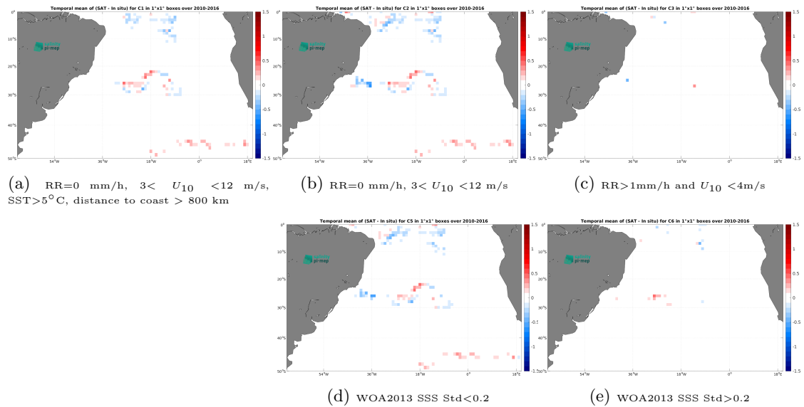
Figure 11: Temporal mean gridded over spatial boxes of size 1^\circ \times 1^\circ of \Delta SSS (CCI SSS L4 Merged-OI v4.4 - 7-day running (ESA) - Surface drifters) for 5 different subdatasets corresponding to:RR=0 mm/h, 3 < U_{10} < 12 m/s, SST >5^\circ C, distance to coast > 800 km (a), RR=0 mm/h, 3 < U_{10} < 12 m/s (b), RR >1 mm/h and U_{10} < 4 m/s (c), WOA2013 SSS Std <0.2 (d), WOA2013 SSS Std >0.2 (e).
