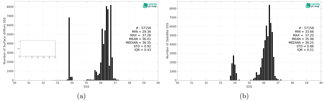
Figure 2: Histograms of SSS from Surface drifters (a) and CCI SSS L4 Merged-OI v4.4 - 7-day running (ESA) (b) considering all match-up pairs per bins of 0.1 over the South Atlantic Ocean Pi-MEP region and for the full satellite product period.
