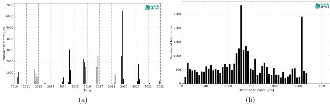
Figure 1: Number of match-ups between TSG (SAMOS) and CCI SSS L4 Merged-OI v4.4 - 30-day running (ESA) SSS as a function of time (a) and as function of the distance to coast (b) over the South Atlantic Ocean Pi-MEP region and for the full satellite product period.
